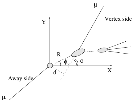
FIG. 1. Sketch of secondary vertex reconstruction scheme in a dimuon event. The primary vertex is represented in the figure as the origin of the X-Y axes. The impact parameter d and the azimuthal angle \phi of tracks from a displaced vertex are related by d = R \sin(\phi - \phi_0) .
