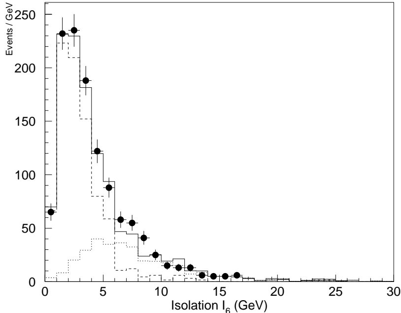
FIG. 12. The distribution in the isolation \mathcal{I}_6 for the W \rightarrow \mu\nu sample (data points), fitted to a linear sum of the signal and background. The dashed histogram corresponds to isolated muons, the dotted histogram shows muons originating from QCD processes, and the solid histogram represents their sum.
