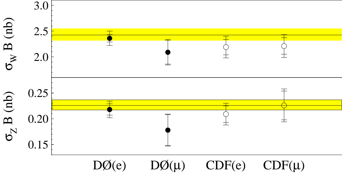
FIG. 15. Measurements and predictions for W \rightarrow l\nu and Z \rightarrow ll cross sections. The results for this experiment are plotted as filled circles and those for the CDF experiment as open circles. The inner error bars represent the combined statistical and systematic uncertainties and the outer error bars include the uncertainty on integrated luminosity. The bands correspond to the range of predictions discussed in the text.
