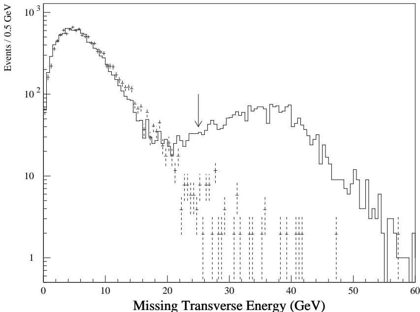
FIG. 11. The \cancel{E}_T distribution for the sample of W \rightarrow e\nu events (solid histogram). The dotted points with error bars represent the multijet QCD background normalized in the low \cancel{E}_T region (0–10 GeV) to the signal sample. The arrow indicates the cutoff for the final selection of \cancel{E}_T > 25 GeV.
