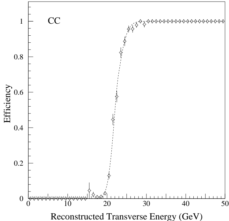
FIG. 13. Trigger efficiency for electrons in the CC as a function of reconstructed E_T . The threshold behavior is similar for electrons in the EC. The line is a function fitted to the data points.
