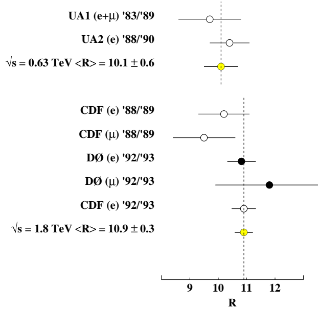
FIG. 16. Measurements of the ratio of the W \rightarrow l\nu and Z \rightarrow ll cross sections multiplied by their respective branching fractions. The results are shown as a function of the years of the data run.
