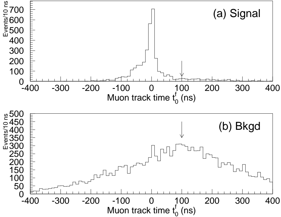
FIG. 6. The t_0^f distributions for (a) good muons and (b) background. The arrows indicate the cut used in this analysis at t_0^f = 100 ns.
