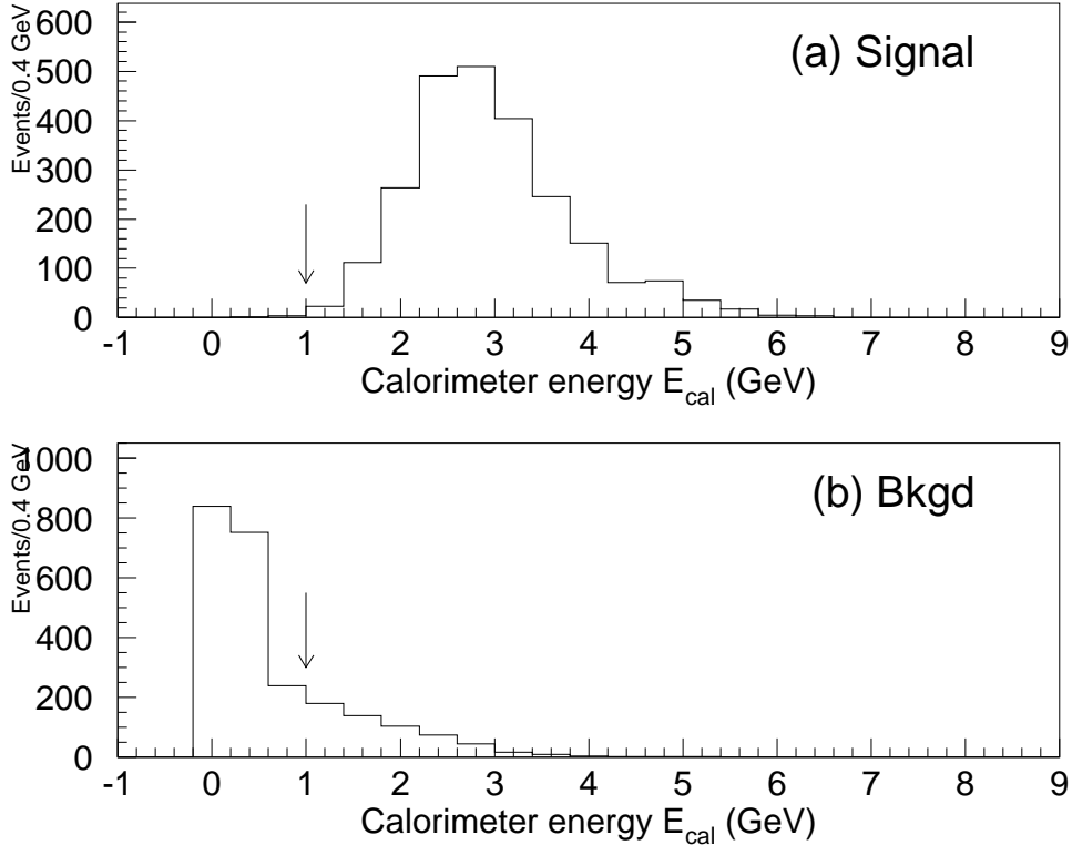
FIG. 5. Calorimeter energy for (a) good muons and (b) background. The arrows indicate the cutoff used in this analysis at E_{\text{cal}} = 1 GeV.
