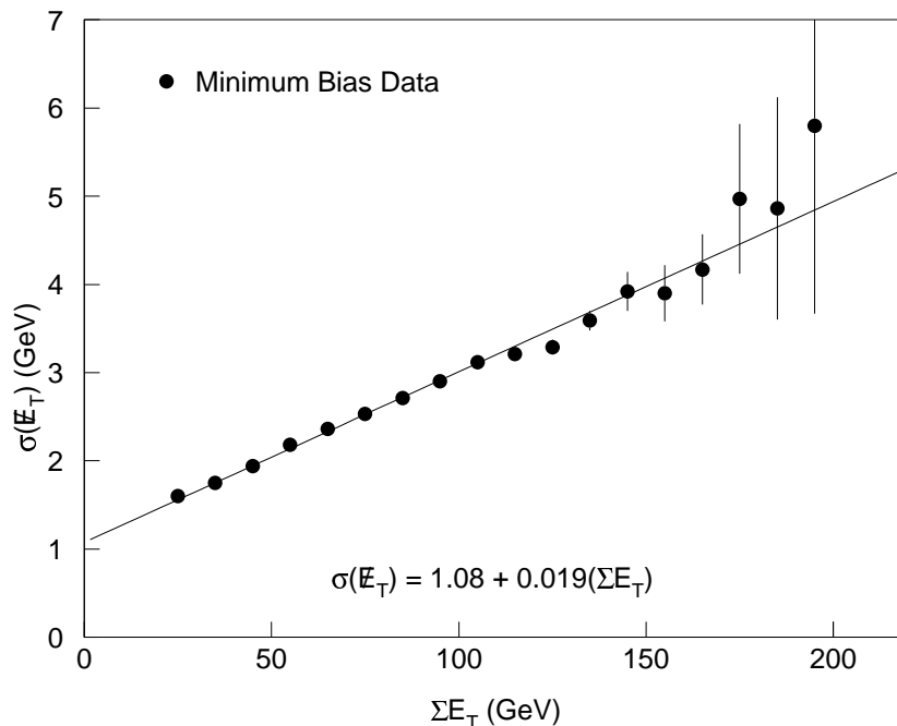
FIG. 10. Resolution in missing transverse energy for minimum bias data.
