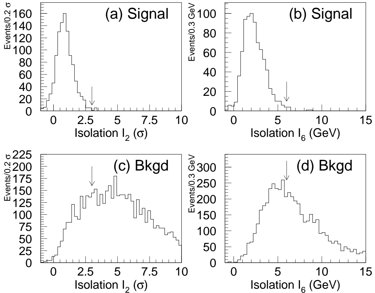
FIG. 8. Isolation distributions for (a) and (b) isolated muons, and (c) and (d) non-isolated muons. The arrows indicate the cutoffs used in this analysis: I_2 = 3 and I_6 = 6 GeV.
