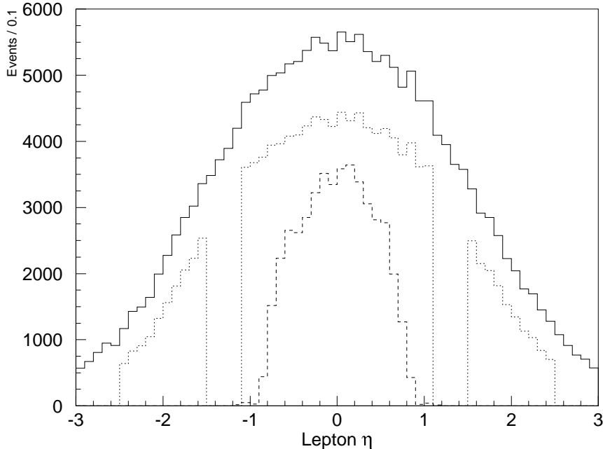
FIG. 14. Pseudorapidity distributions for charged leptons in W \rightarrow l\nu events. The solid line is the generated distribution for either electrons or muons. The dotted and dashed lines show the distributions for the electron and muon channels, respectively, after applying the fiducial requirements.
