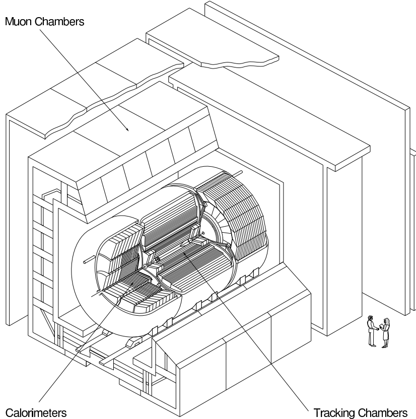
FIG. 1. Cutaway isometric view of the DØ detector.
