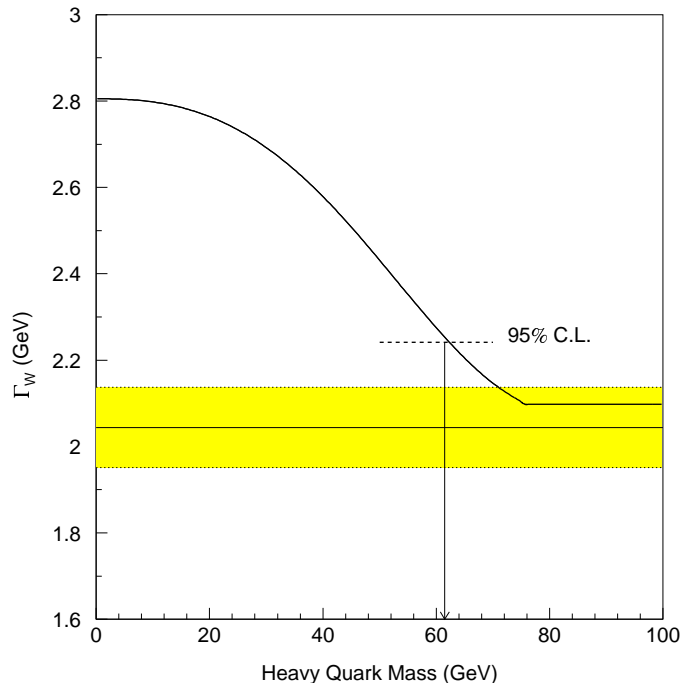
FIG. 17. The width of the W boson as a function of a new quark mass. Our measurement is shown as a one standard deviation band with the central value represented by the solid line. The darker curve represents the prediction of the standard model as a function of quark mass. The short dashed line indicates the upper limit at 95% CL on the width of the W boson from our data.
