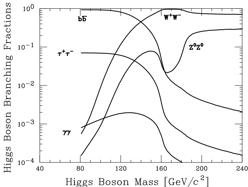
Fig. 5. Branching fractions for the prominent decay modes of a light Higgs boson.
