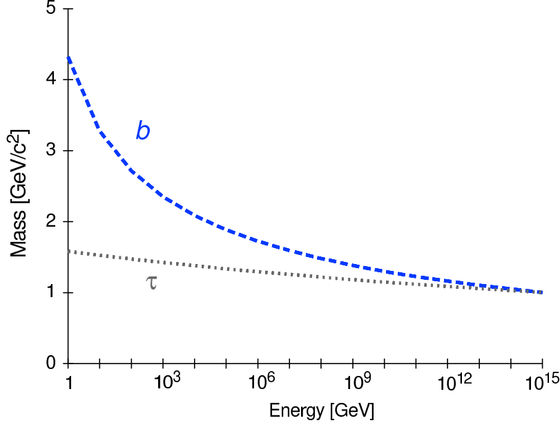
Fig. 15. Evolution of the \tau -lepton and b -quark masses from the unification scale to low energies.
