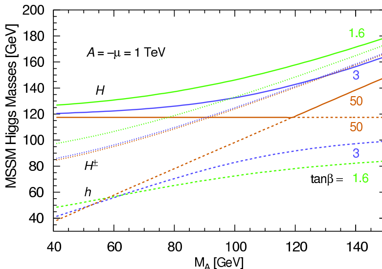
Fig. 12. Higgs-boson masses in the minimal supersymmetric standard model as a function of M_A for the case A = -\mu = M_S = 1 TeV, for a top-quark mass m_t = 175 GeV/ c^2 , from Ref. [76].
