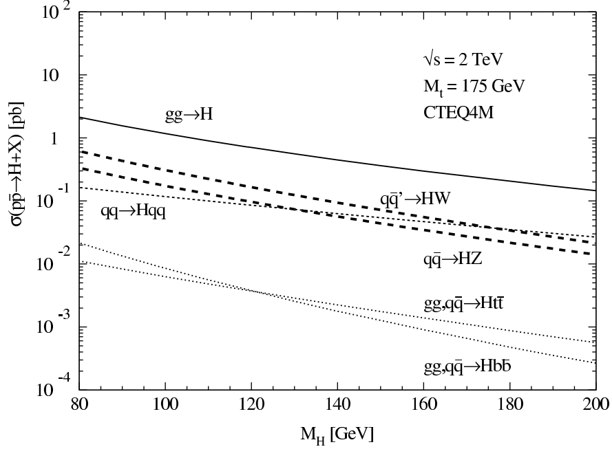
Fig. 9. Cross sections for Higgs-boson production in 2-TeV \bar{p}p collisions, from Ref. [41].
