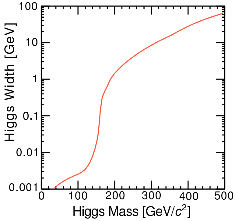
Fig. 7. Higgs-boson total width as a function of mass.
