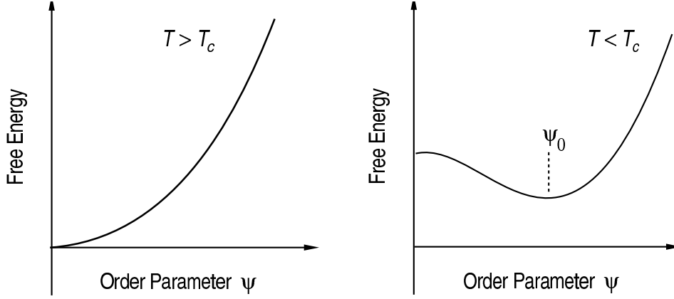
Fig. 1. Ginzburg-Landau description of the superconducting phase transition.
