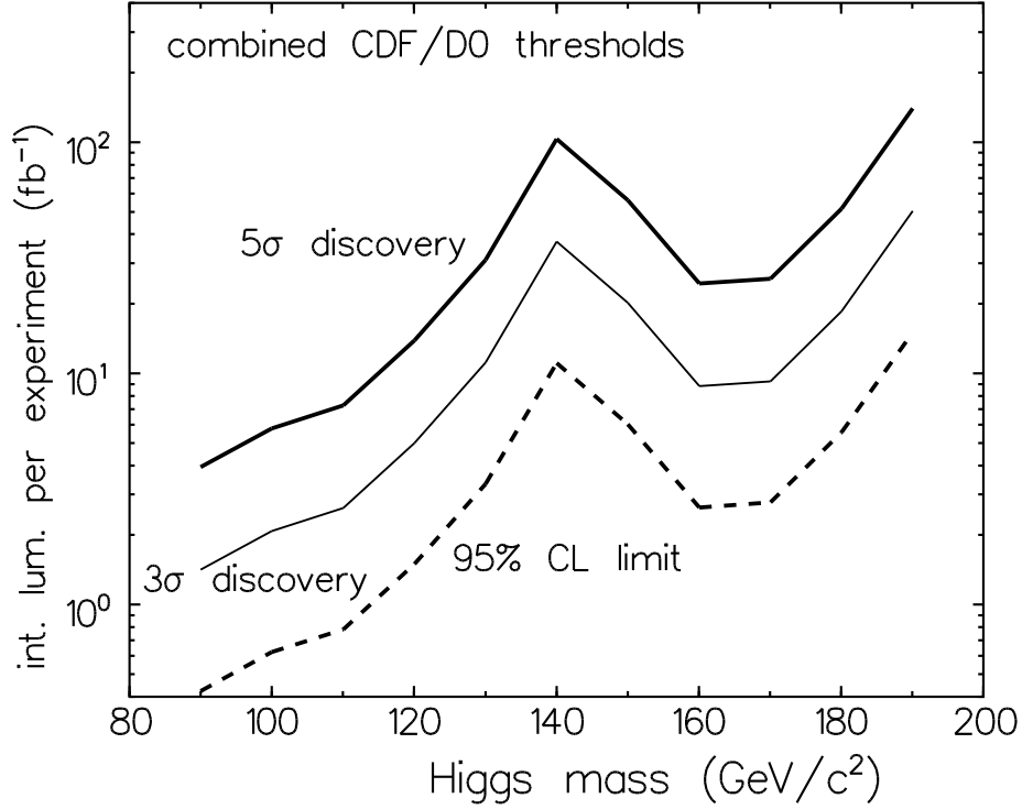
Fig. 10. Integrated luminosity projected for the detection of a standard-model Higgs boson at the Tevatron Collider.
