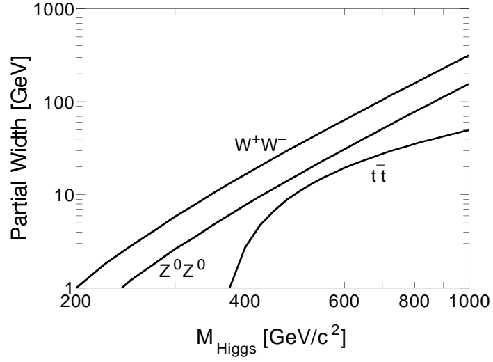
Fig. 6. Partial widths for the prominent decay modes of a heavy Higgs boson.
