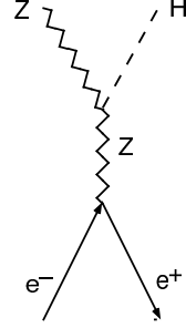
Fig. 8. Lowest-order contributions to the e^+e^- \rightarrow HZ^0 scattering amplitude.
