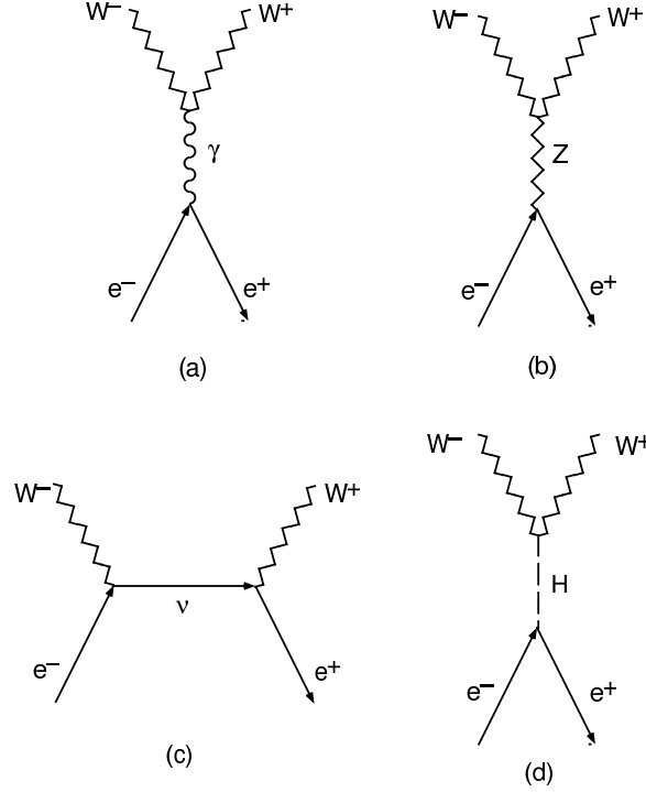
Fig. 3. Lowest-order contributions to the e^+e^- \rightarrow W^+W^- scattering amplitude.
