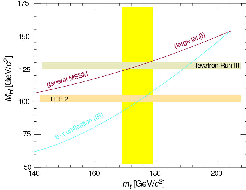
Fig. 13. Upper bounds on the mass of the lightest Higgs boson, as a function of the top-quark mass, in two variants of the minimal supersymmetric standard model. The upper curve refers to a general MSSM, in the large- \tan\beta limit; the lower curve corresponds to an infrared-fixed-point scenario with b - \tau unification, from Ref. [77].
