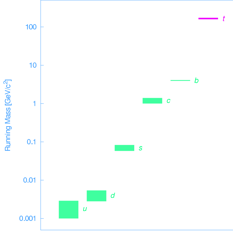
Fig. 14. Running masses [m_q(m_q)] of the quarks in the \overline{\text{MS}} scheme.
