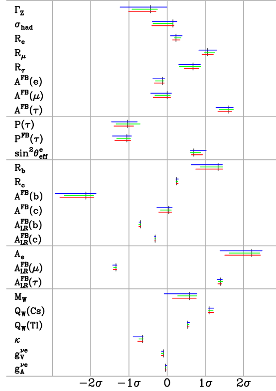
Fig. 11. The range of best fit predictions of precision observables in the supergravity model (upper horizontal lines), the 5 \oplus 5^* gauge-mediated model (middle lines), the 10 \oplus 10^* gauge-mediated model (lower lines), and in the standard model at its global best fit value (vertical lines), in units of standard deviation, from Ref. [63].
