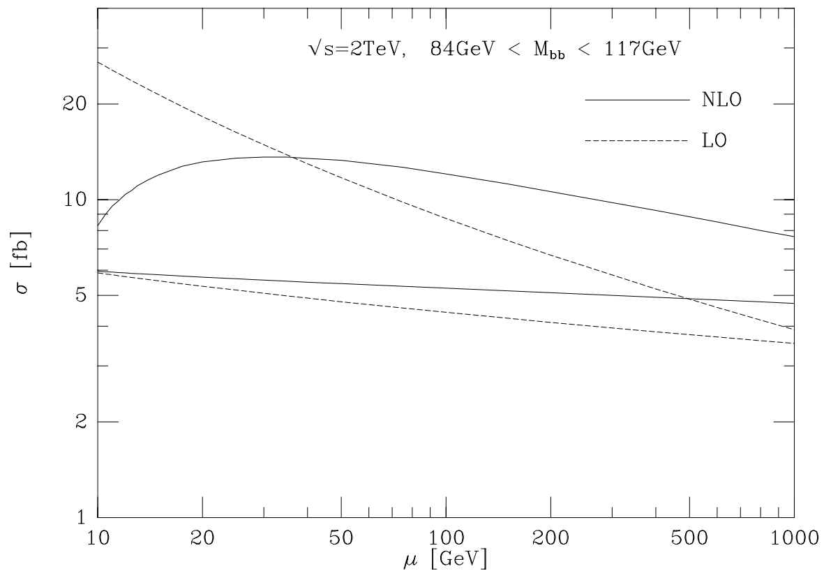
Figure 3: Cross section scale dependence for the signal (lower curves) and Wb\bar{b} background (upper curves). These results were obtained for 84 < M_{b\bar{b}} < 117 GeV ( M_H = 100 GeV), and after imposing cuts given in (4)-(6).
