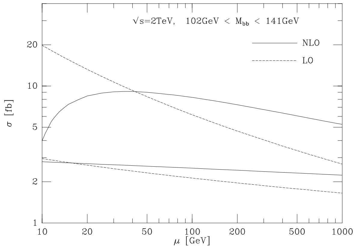
Figure 4: Cross section scale dependence for the signal (lower curves) and Wb\bar{b} background (upper curves). These results were obtained for 102 < M_{b\bar{b}} < 141 GeV ( M_H = 120 GeV), and after imposing cuts given in (4)-(6).
