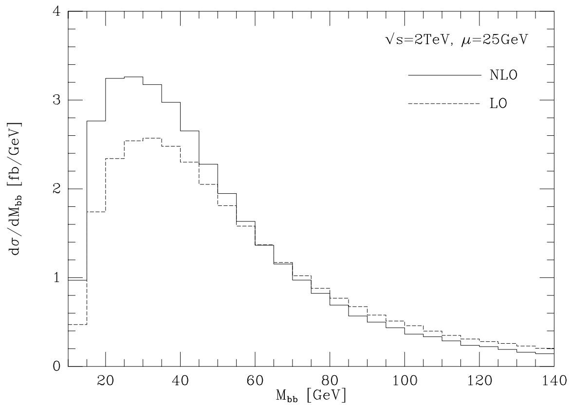
Figure 2: The LO and NLO M_{b\bar{b}} dependence of the Wb\bar{b} background process at a scale of \mu = 25 GeV. The results shown were obtained after imposing cuts given in (4)-(6).
