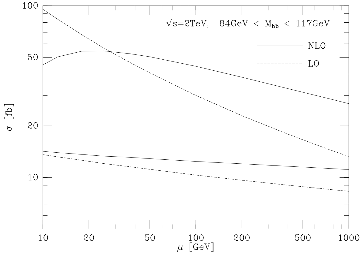
Figure 1: Cross section scale dependence for the signal (lower curves) and Wb\bar{b} background (upper curves). These results were obtained for 84 < M_{b\bar{b}} < 117 GeV ( M_H = 100 GeV). Apart from (3), no other cuts have been applied.
