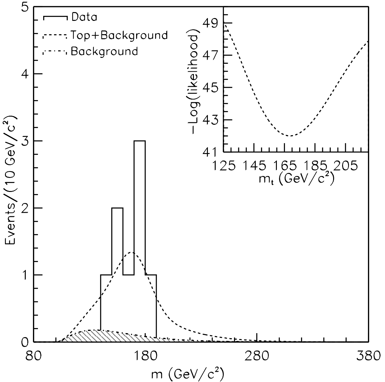
FIG. 2. Reconstructed top mass for the eight dilepton events (solid). Background distribution (shaded, 1.3 events) and top Monte Carlo (6.7 events) added to background (dashed). The negative log-likelihood distribution as a function of the top mass is shown in the inset.
