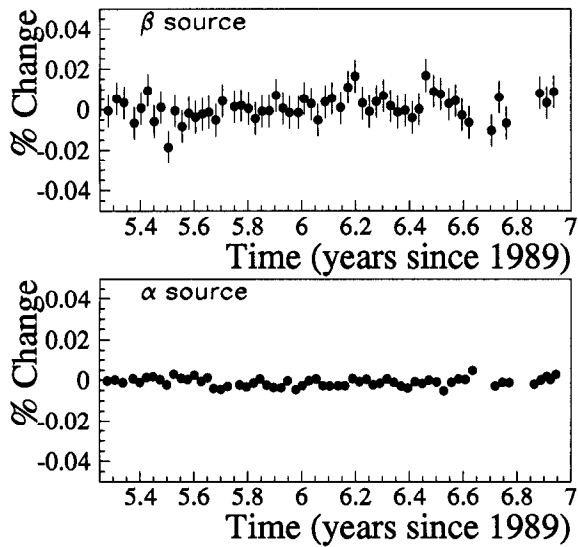
FIG. 7. The response of the liquid argon in the central calorimeter as monitored by \alpha and \beta sources.
