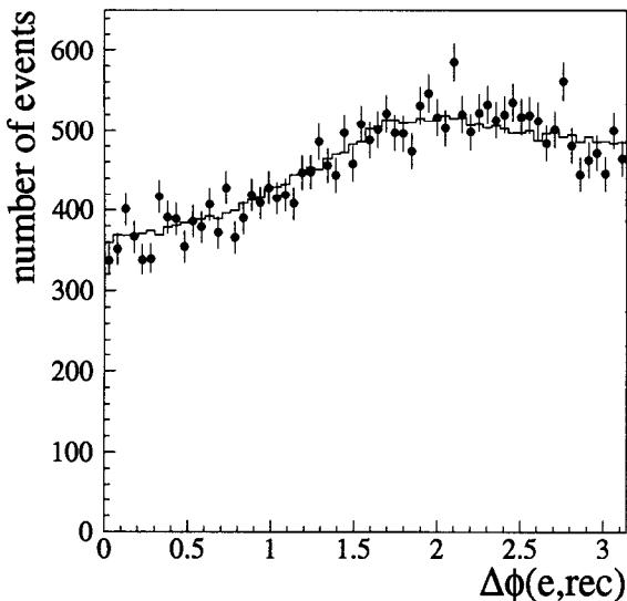
FIG. 50. The azimuthal difference between electron and recoil directions for the W data ( \bullet ) and the Monte Carlo simulation (—).
