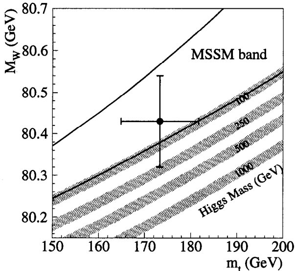
FIG. 75. A comparison of the W and top quark mass measurements by the DØ collaboration with the Standard Model predictions for different Higgs boson masses [53]. The width of the bands for each Higgs boson mass value indicates the uncertainty due to the error in \alpha(M_Z^2) . Also shown is the range allowed by the MSSM [21].
