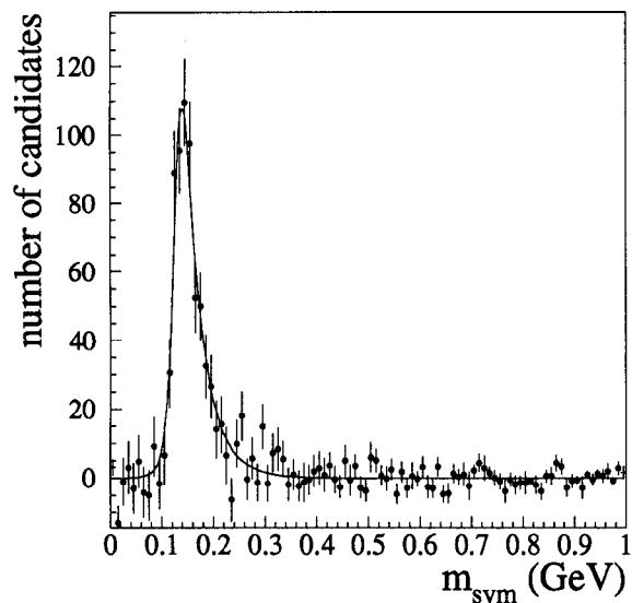
FIG. 30. The background-subtracted m_{sym} distribution. The superimposed curve shows the Monte Carlo simulation.
