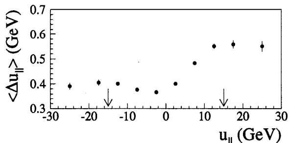
FIG. 25. The variation of \langle \Delta u_{\parallel} \rangle as a function of u_{\parallel} . The region between the arrows is populated by the W sample.
