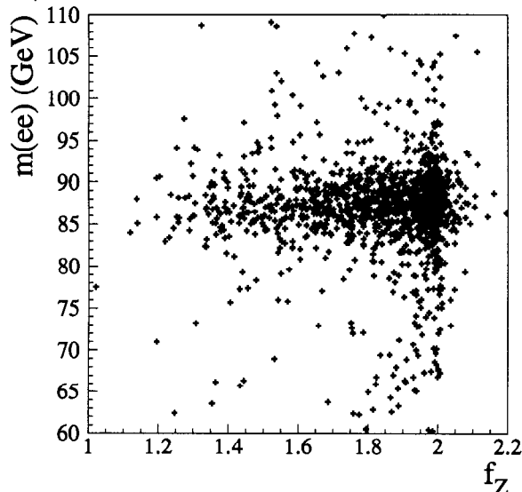
FIG. 33. The distribution of m(ee) versus f_Z for the C-C-CC Z \rightarrow ee sample.
