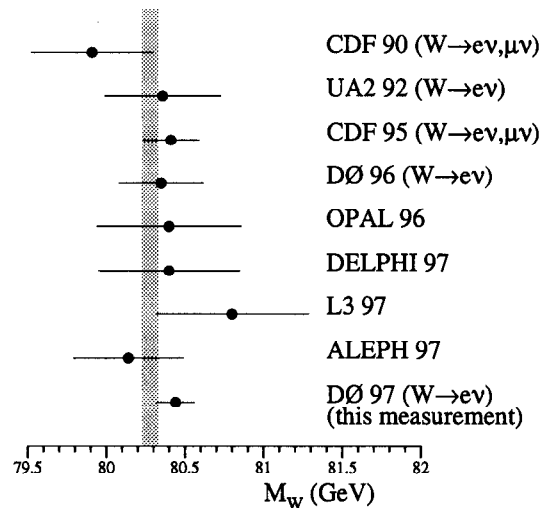
FIG. 74. A comparison of this measurement with previously published W mass measurements (Table XV). The shaded region indicates the predicted W mass value from global fits to the Z lineshape data [9].
