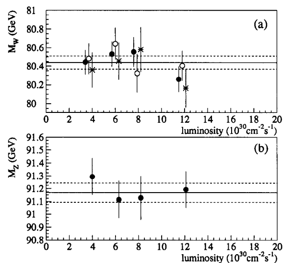
FIG. 66. The fitted W boson masses (a) in bins of luminosity from the m_T ( \bullet ), p_T(e) ( \circ ), and p_T(\nu) ( * ) fits (the points are offset for clarity) and the fitted Z boson masses (b). The solid line is the central value for the m_T and m(ee) mass fits respectively over the entire luminosity range and the dashed lines are the statistical errors.
