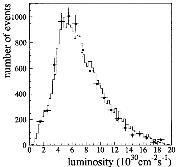
FIG. 17. The luminosity distribution of the W (—) and the Z (●) samples.
