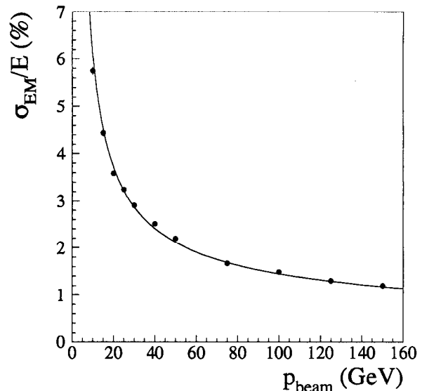
FIG. 11. The fractional electron energy resolution measured in beam tests of a CC-EM module for the data ( \bullet ) and the parameterization ( \text{—} ).
