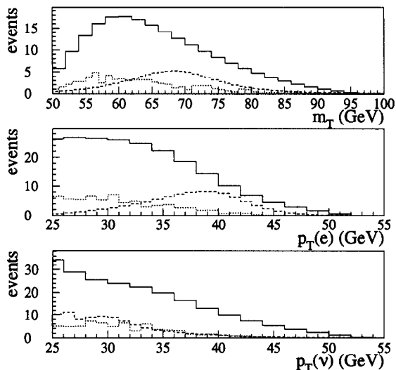
FIG. 56. Shape of m_T , p_T(e) , and p_T(\nu) spectra from hadron (—), Z (---), and \tau \rightarrow \text{hadron} backgrounds (.....) with the proper relative normalization.
