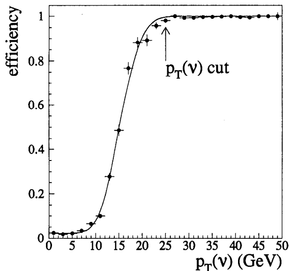
FIG. 13. The efficiency of a 15 GeV Level 2 p_T requirement. The arrow indicates the cut applied in the final event selection.
