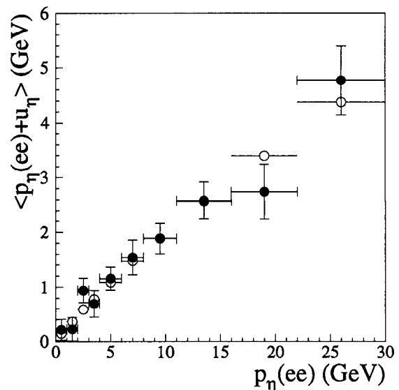
FIG. 39. The average p_\eta(ee) + u_\eta versus p_\eta(ee) for the Z data ( \bullet ) and the fast Monte Carlo simulation ( \circ ).
