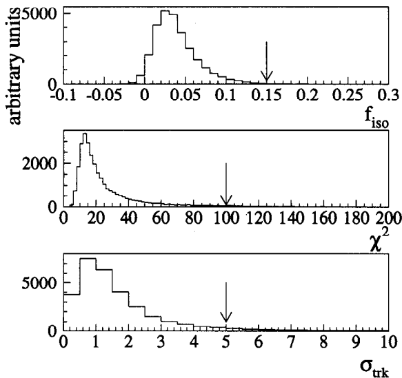
FIG. 16. Distributions of the electron identification variables. The arrows indicate the cut values.
