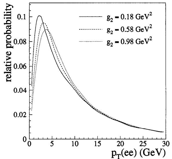
FIG. 53. The predicted p_T(ee) spectra after detector simulation using MRSA' parton distribution functions and g_2 = 0.18, 0.58, \text{ and } 0.98 \text{ GeV}^2 .
