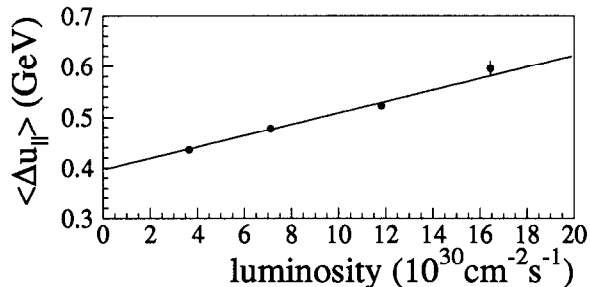
FIG. 24. The luminosity dependence of \langle \Delta u_{\parallel} \rangle .
