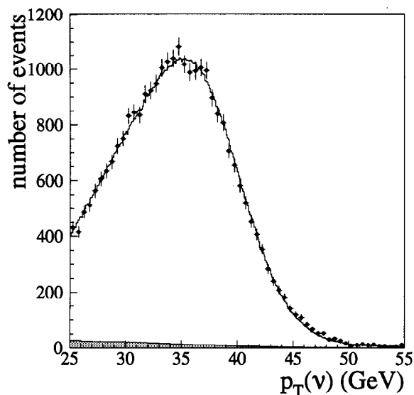
FIG. 64. Spectrum of p_T(\nu) from the W data. The superimposed curve shows the maximum likelihood fit and the shaded region shows the estimated background.
