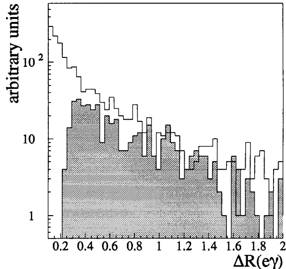
FIG. 20. The distribution of \Delta R(e\gamma) of photons from W \rightarrow e\nu\gamma decays that are reconstructed as separate objects (shaded) and those that are not, either because they are too close to the electron or too low in energy (—).
