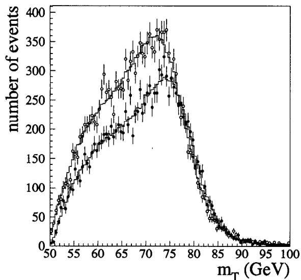
FIG. 67. Spectra of m_T from W data with u_{||} < 0 ( \circ ) and u_{||} > 0 ( \bullet ) compared to Monte Carlo simulations (—).
