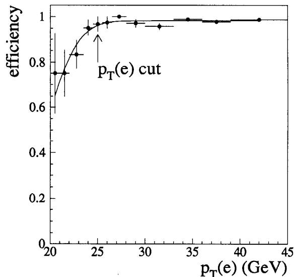
FIG. 12. The relative efficiency of the Level 2 electron filter for a threshold of 20 GeV. The arrow indicates the cut applied in the final event selection.
