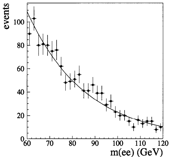
FIG. 32. The dielectron mass spectrum for the background data sample to the CC/CC Z sample. The fit is an exponential.
