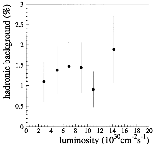
FIG. 55. The fraction of hadron background as a function of luminosity.
