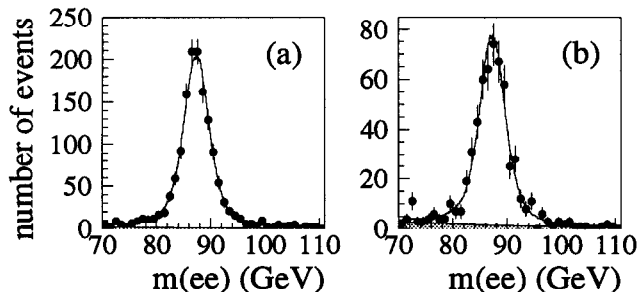
FIG. 36. The dielectron mass spectra from (a) the tight/tight and (b) the tight/loose CC-CC Z samples. The curves show the fitted Monte Carlo spectra.
