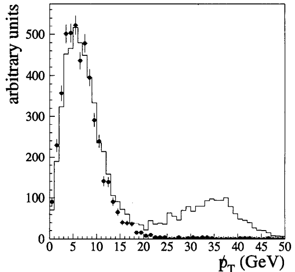
FIG. 54. The \cancel{p}_T spectra of a sample of events passing electron identification cuts (—) and a sample of events failing the cuts (•).
