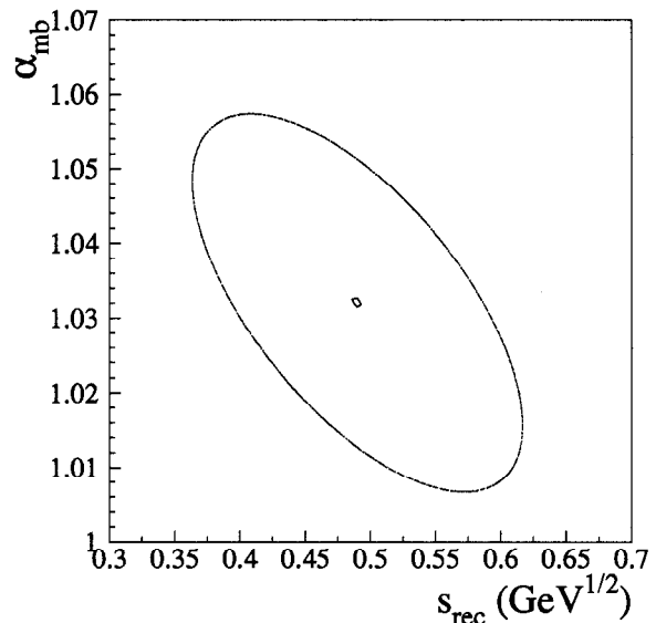
FIG. 42. The \chi_0^2 + 1 contour for the recoil resolution parameters \alpha_{\text{mb}} and s_{\text{rec}} .
