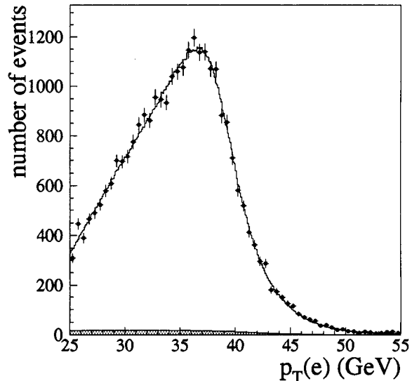
FIG. 57. Spectrum of p_T(e) from the W data. The superimposed curve shows the maximum likelihood fit and the shaded region the estimated background.
