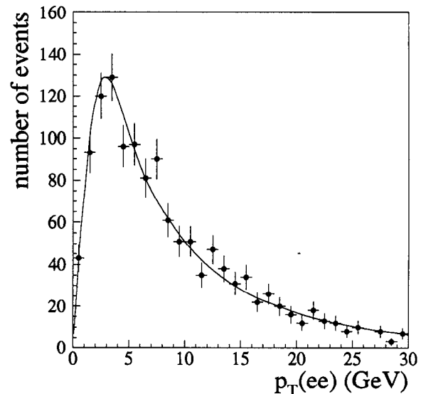
FIG. 51. Comparison of the p_T(ee) data ( \bullet ) and simulation (—) for the best fit g_2 using MRSA' parton distribution functions.
