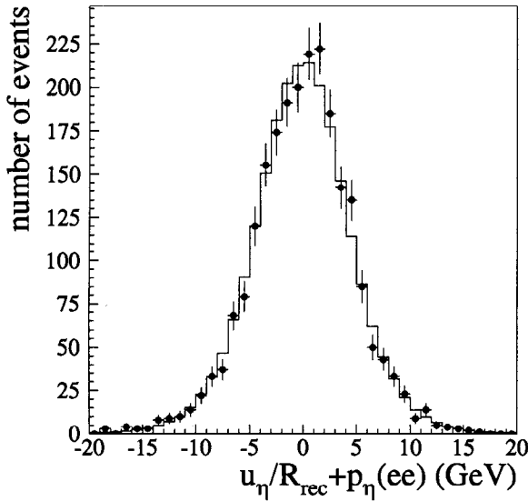
FIG. 43. The \eta -balance distribution for the Z data ( \bullet ) and the fast Monte Carlo simulation (—).
