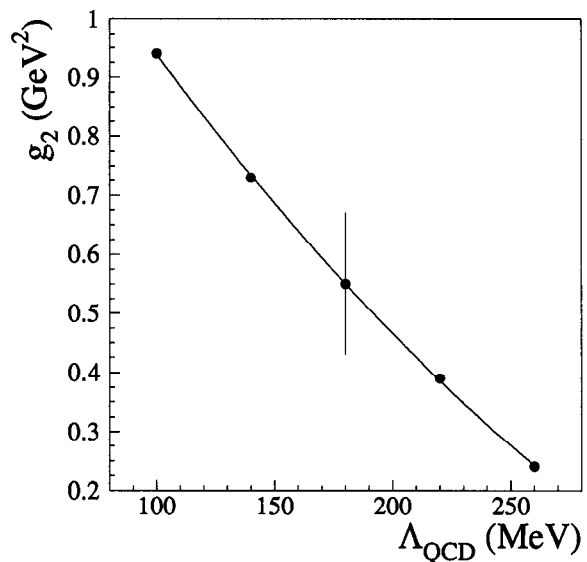
FIG. 73. Value of g_2 as a function of \Lambda_{QCD} . The error bar indicates the uncertainty in g_2 for fixed \Lambda_{QCD} .
