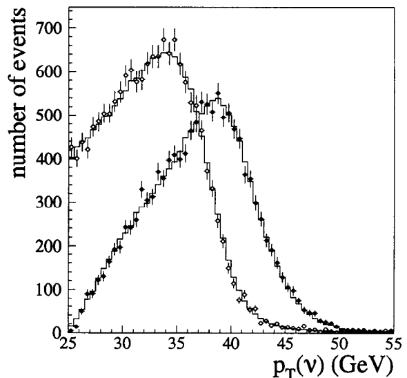
FIG. 69. Spectra of p_T(\nu) from W data with u_{||} < 0 ( \circ ) and u_{||} > 0 ( \bullet ) compared to Monte Carlo simulations (—).
