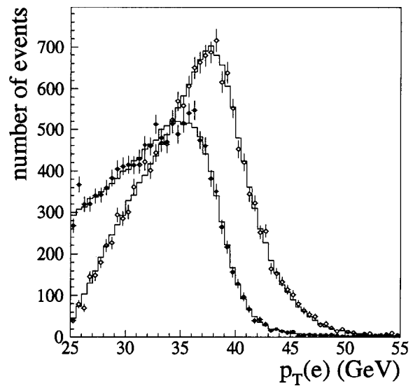
FIG. 68. Spectra of p_T(e) from W data with u_{||} < 0 ( \circ ) and u_{||} > 0 ( \bullet ) compared to Monte Carlo simulations (—).
