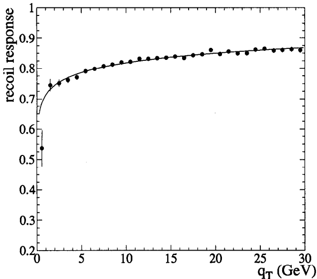
FIG. 38. The recoil momentum response in the Monte Carlo Z sample as a function of q_T .
