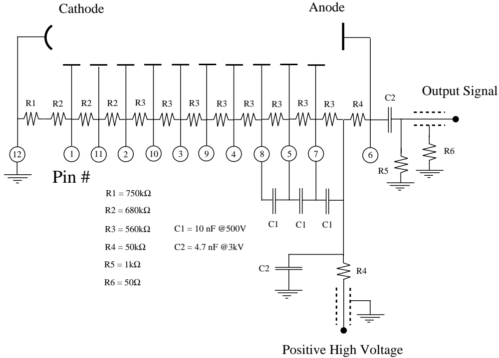
Fig. 9. The circuit diagram for the photomultiplier base.
