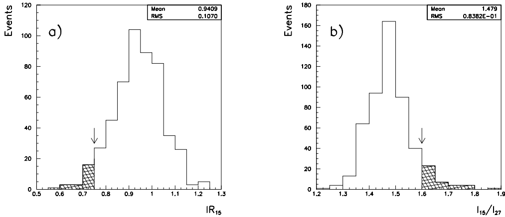
Fig. 12. (a)The distribution of the absolute light output parameter IR_{15} .
