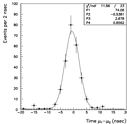
Fig. 21. The difference in scintillator times for a sample of dimuon events.
