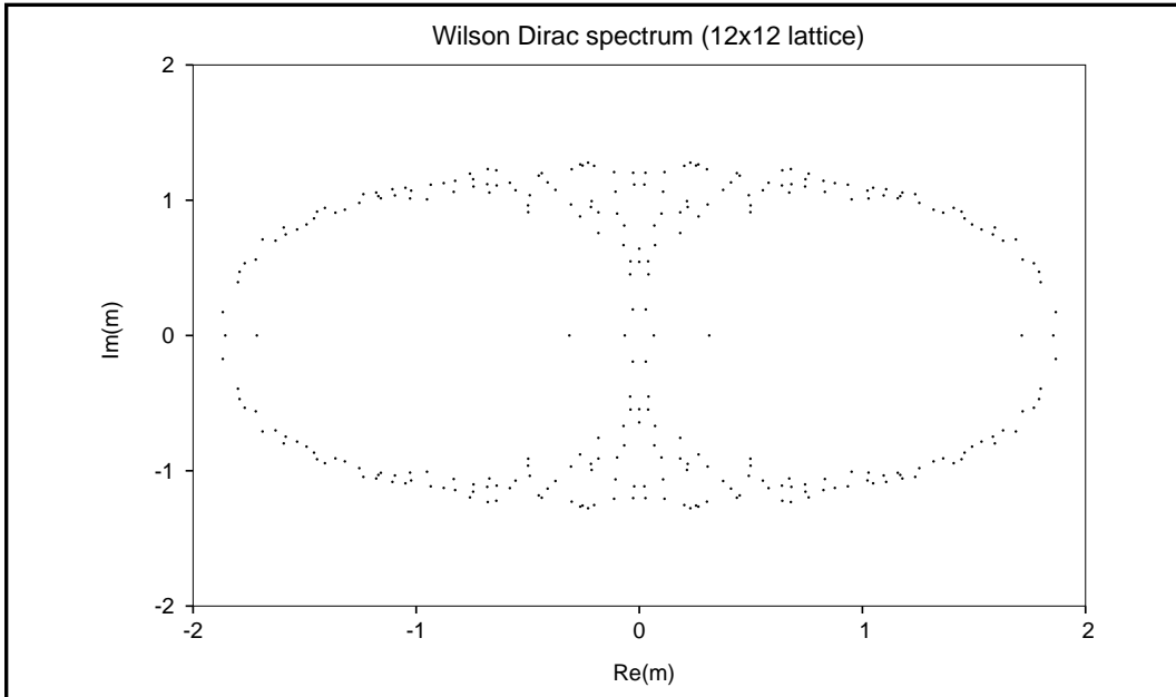
Figure 1: Example of the eigenvalue spectrum for the Wilson-Dirac operator for QED2 on a 12 \times 12 lattice with \beta = 4.5 .
