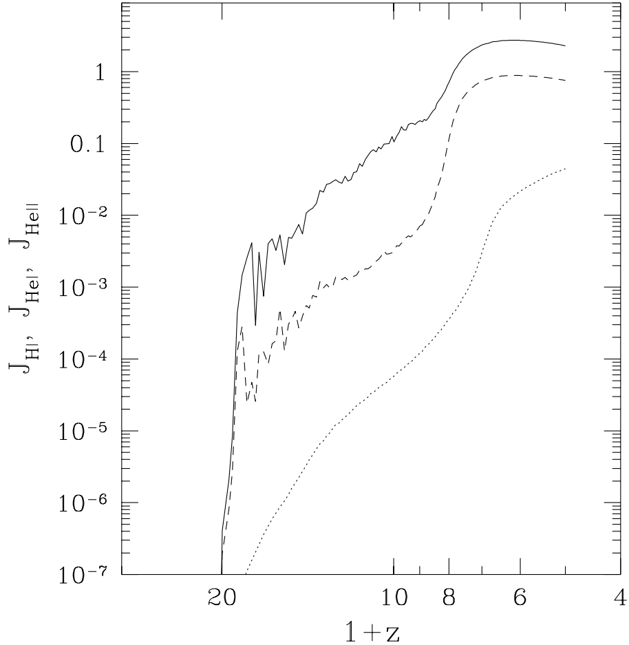
Figure 2. Evolution of J_{\text{HI}} (solid line), J_{\text{HeI}} (dashed line) and J_{\text{HeII}} (dotted line) as a function of redshift, used in the computations shown in Fig. 1. The J_i 's are defined in equation (5).
