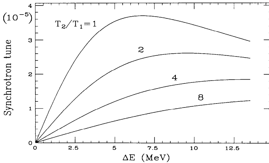
FIG. 2. The synchrotron tune vs the off-energy parameter \Delta E . The parameters used in this plot are E_0 = 8.9 GeV, f_{\text{rev}} = 89.8 kHz, V_0 = 2 kV, \gamma_T = 20.7 , and T_1 = 0.5\mu\text{s} . Note that if T_2 > 4T_1 , the synchrotron tune is a monotonic function of \Delta E . On the other hand, if T_2 < 4T_1 , the synchrotron tune is peaked at an off-energy \Delta E smaller than the bucket height \Delta E_b .
