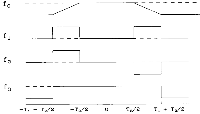
FIG. 3. Schematic drawing of the form factors f_0, f_1, f_2 and f_3 used in this paper for the barrier rf system.
