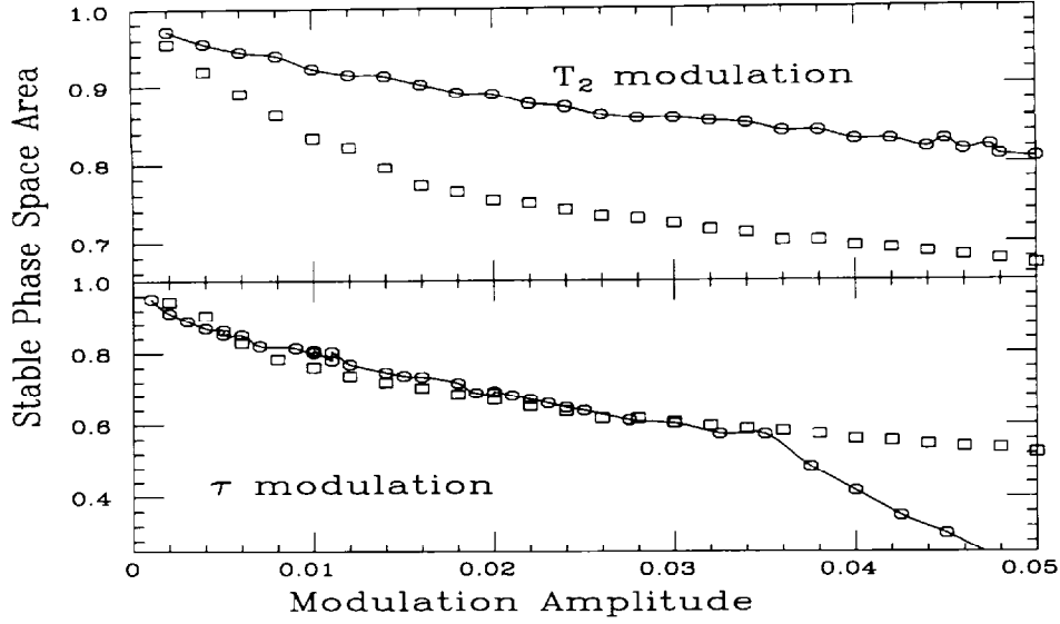
FIG. 9. The stable phase space area (in unit of the bucket area) vs the modulation amplitude at 1:1 parametric resonance for the shaking phase modulation (bottom plot) and 2:1 parametric resonance for the breathing phase modulation (top plot). Circular symbols (connected with a line) and rectangular symbols are obtained from the rf parameters with T_2/T_1 = 1 and 4 respectively. The cusp in the rf phase modulation is due to a peaked characteristic of the synchrotron tune.
