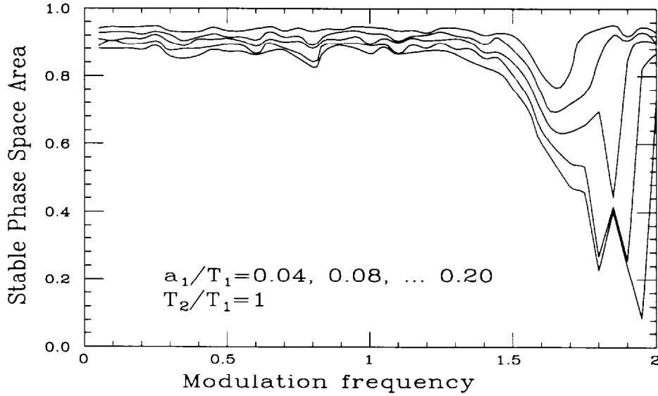
FIG. 6. The stable phase space area (in unit of the bucket area) vs the modulation frequency (in unit of the maximum synchrotron frequency) for the breathing rf phase modulation with T_2 = T_1 and a_1/T_1 = 0.04, 0.08, \dots, 0.20 .
