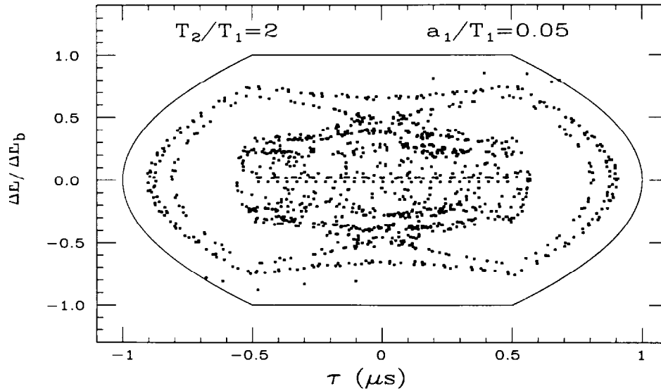
FIG. 4. The Poincaré surface of section at \omega_m = 1.95\omega_{s,\text{max}} . The 2:1 parametric resonance generated by the rf breathing phase modulation with a_1/T_1 = 0.05 , and T_2/T_1 = 2 . Note that the last torus is about 60% of the bucket height shown as solid lines. Orbits outside the last torus are not bounded by the barrier bucket.
