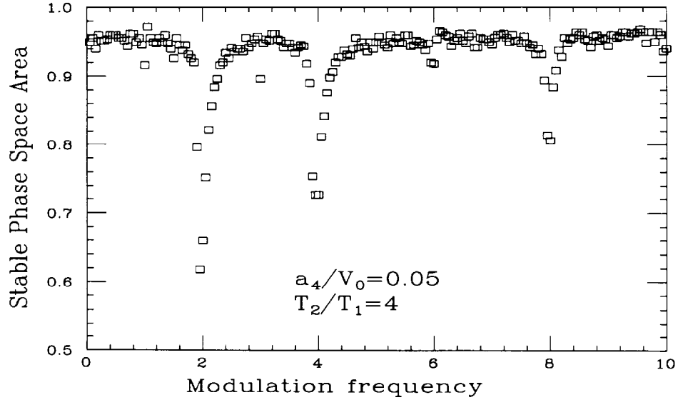
FIG. 10. The stable bucket area (in ratio to the bucket area) vs the rf voltage modulation frequency (in ratio to the maximum synchrotron frequency). The modulation amplitude is 5% of the rf voltage amplitude, i.e., a_4/V_0 = 0.05 . The ratio of the rf pulse gap to the pulse width is T_2/T_1 = 4 . A small excitation at the 6:1, 10:1, \dots is due to the vanishing cosine term in G_6, G_{10}, \dots for synchrotron orbits at the barrier height.
