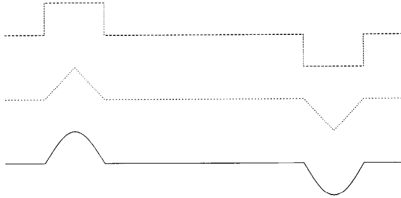
FIG. 1. Possible wave forms for the barrier bucket. The barrier rf wave is characterized by a voltage height V_0 , a pulse width T_1 and a pulse gap T_2 . Below the transition energy with \eta < 0 , particles are confined within the positive and negative pulses region. Above the transition energy, the sign of the voltage wave should be reversed.
