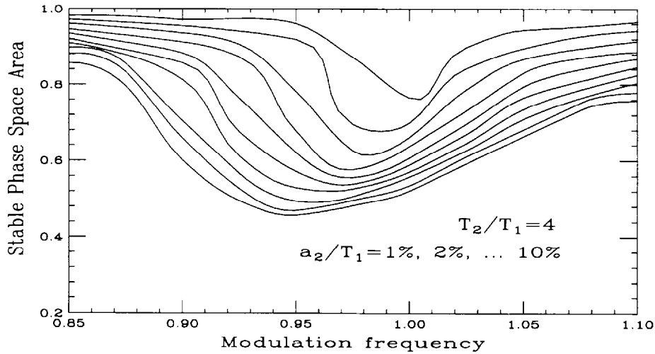
FIG. 8. The stable phase space area (in unit of the bucket area) near 1:1 parametric resonance due to the rf phase modulation for T_2/T_1 = 4 . The modulation frequency is in unit of the maximum rf frequency. The modulation amplitudes are a_2/T_1 = 0.01, 0.02, \dots, 0.10 respectively.
