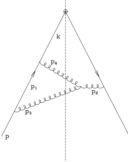
Figure 7: An example of the graph of topology (cd)
