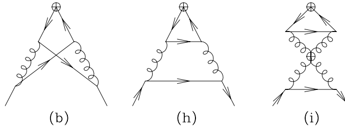
Figure 4: The q\bar{q} diagrams
