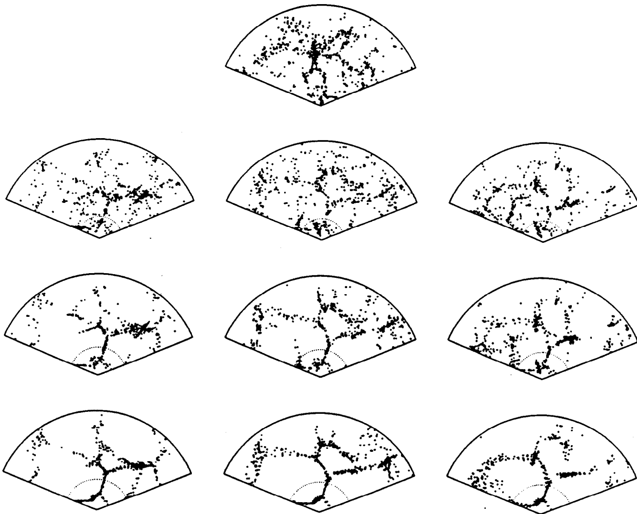
Figure 6: CfA-like redshift slices of the observed galaxy distribution. The observer is located at the bottom of each slice. The slices are 256 Mpc deep (with our choice of the Hubble constant). The top panel represents a slice of the real observed galaxy distribution (courtesy V. de Lapparent). The others panels correspond to artificial catalogs built from the simulations, taking into account redshift-space distortions and selection effects (see text). From top to bottom, one passes from CDM to WDM and HDM. The central slices have the same geometry as the CfA slice, i.e. are covering the declination range 26.5^\circ < \delta < 32.5^\circ . The left slices are the adjacent slices with 20.5^\circ < \delta < 26.5^\circ and the right ones are the adjacent slices with 26.5^\circ < \delta < 32.5^\circ . All the slices are projected on the plane \delta = 0 , and rescaled so that they have all the same apparent size. The small dotted arcs of a circle determine a limit below which we undersample the observed galaxy distribution (see text).
