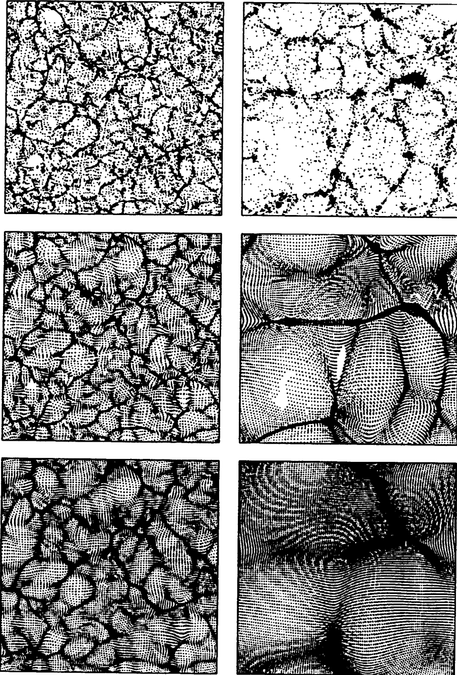
Figure 4: Thin slices L_{\text{box}}/32 thick extracted from the simulations PML (lefts panels) of physical size L_{\text{box}} = 720 Mpc and the simulations PMS (right panels) of physical size L_{\text{box}} = 144 Mpc. The top, middle and bottom panels correspond respectively to the CDM, WDM and HDM model.
