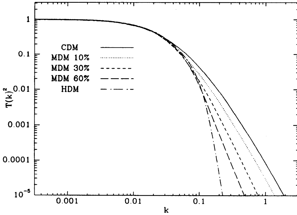
Figure 1: Transfer functions for WDM (top) and MDM (bottom) models. k is in units of h \text{ Mpc}^{-1} .
