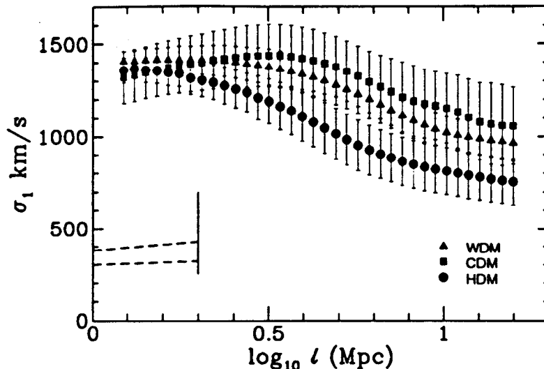
Figure 9: The quantity \sigma_1 (defined in Eq. [27]) as function of separation l measured in our N -body experiments, compared to measurements in the observed galaxy distribution. The two dashed lines at the bottom left correspond to the measurement of Davis & Peebles (1983) on the CfA1 catalog and the thick vertical segment to a compilation of the more recent measurements of Mo et al. (1993) on various galaxy catalogs (see text).
