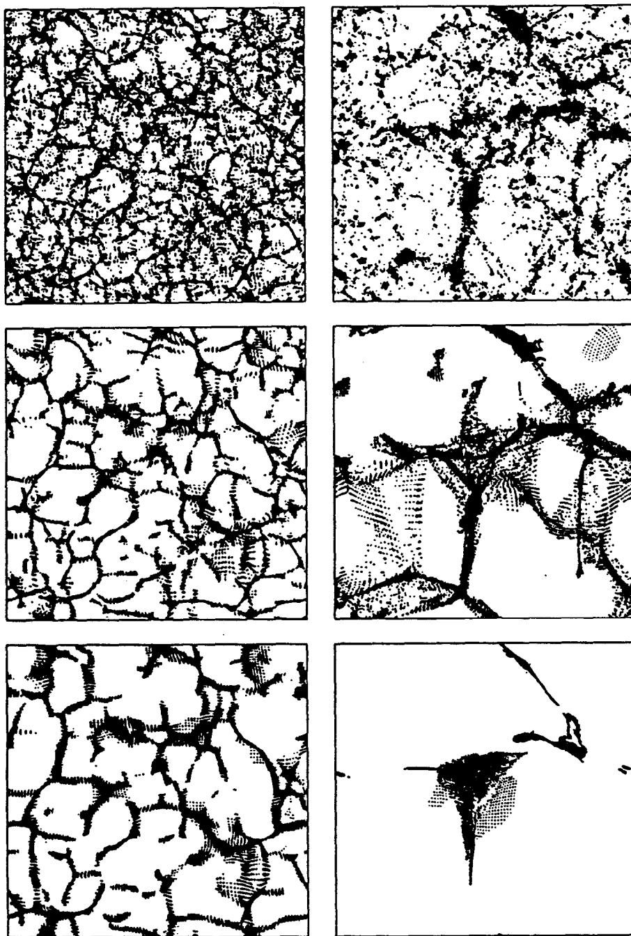
Figure 5: Same as in figure 4, but only overdense regions, where galaxies are expected to remain, have been kept and the slices are thicker. In the left panels, the slices are L_{\text{box}}/32 thick; the matter particles belonging to regions of density larger than \rho/\bar{\rho} \simeq 2.33 have been selected at a weakly evolved stage a = 2 and followed until present time. In the right panels, the slices are L_{\text{box}}/4 thick; each point represent a connected group of particles belonging to regions of density larger than \rho/\bar{\rho} \simeq 250 .
