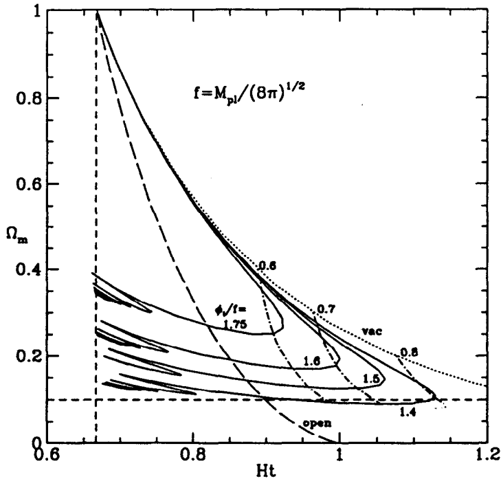
Fig. 2: The non-relativistic mass density \Omega_m = 1 - \Omega_\phi vs. Ht , for f = M_{Pl}/\sqrt{8\pi} . The solid curves correspond to several initial values for the field, \phi_i/f = 1.4, 1.5, 1.6, and 1.75 . The evolution starts at the top of the figure and ends at the lower left. The vertical dashed line shows the Einstein-de Sitter expansion age Ht = 2/3 , the horizontal dashed line shows the lower bound \Omega_m = 0.1 from dynamical mass estimates, the dotted curve (labelled ‘vac’) shows the evolution for a cosmological constant model, and the long-dashed curve corresponds to an open model with \Omega_\phi = 0 . The dot-dashed curves (labelled 0.6, 0.7, 0.8) bracket the constraints from lensed QSOs in the HST snapshot survey (see text).
