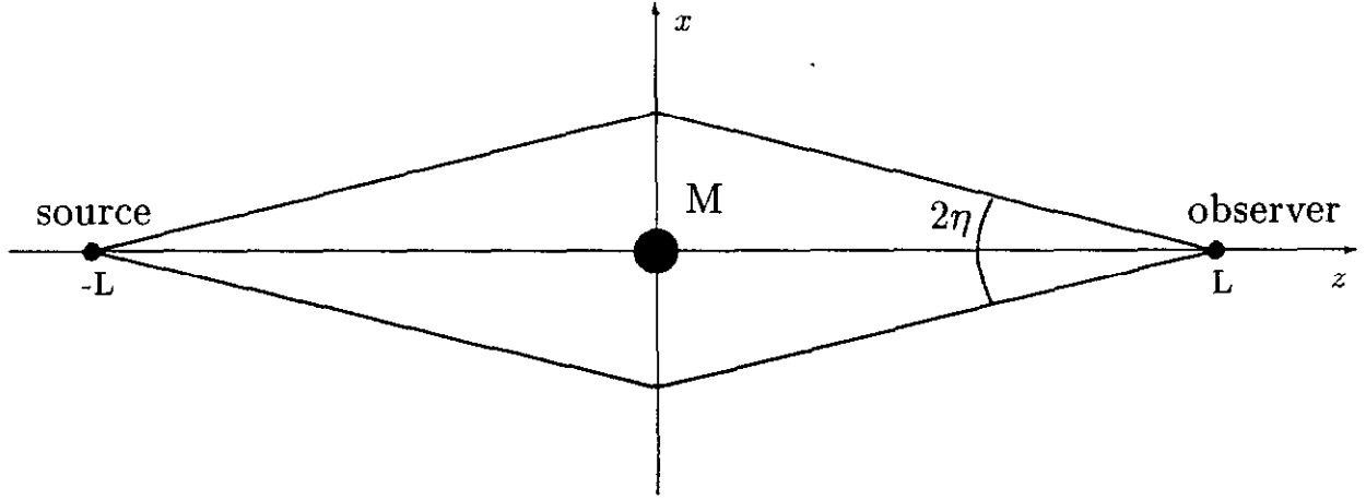
Figure 1: The geometry of an aligned lens. The deflector is a point mass M at the origin of coordinates. Source and observer lie along the z -axis, equidistant from the deflector. The observer sees two images of the same source (actually an Einstein ring) with angular separation 2\eta . The trajectories are approximated by straight segments.
