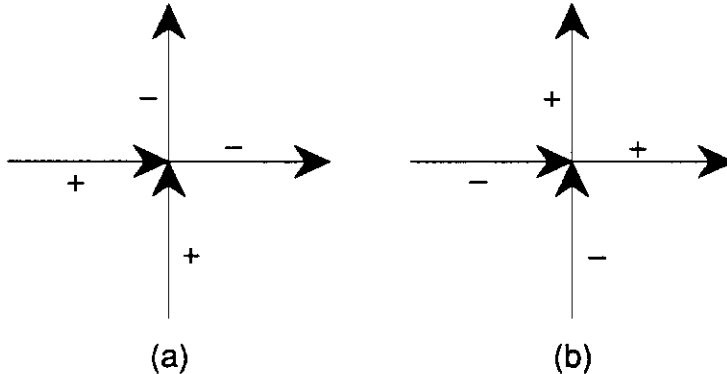
Fig. 3. The two vertex configurations for which all four links couple symmetrically to each other. In figure 2(a) all four links contribute to the \mathcal{J}_+ current at the vertex, and in figure 2(b) all four contribute to \mathcal{J}_- .
