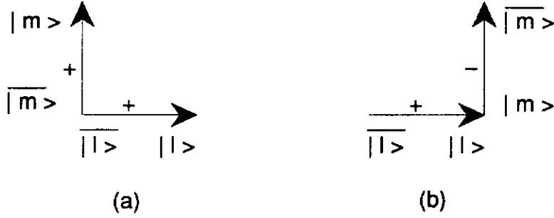
Fig. 5. The two cases encountered when gluing together the zero modes of two links to satisfy the global gauge invariance constraints at a site. Figure 5(a) (5(b)) denotes two links of the same (opposite) lattice parity.
