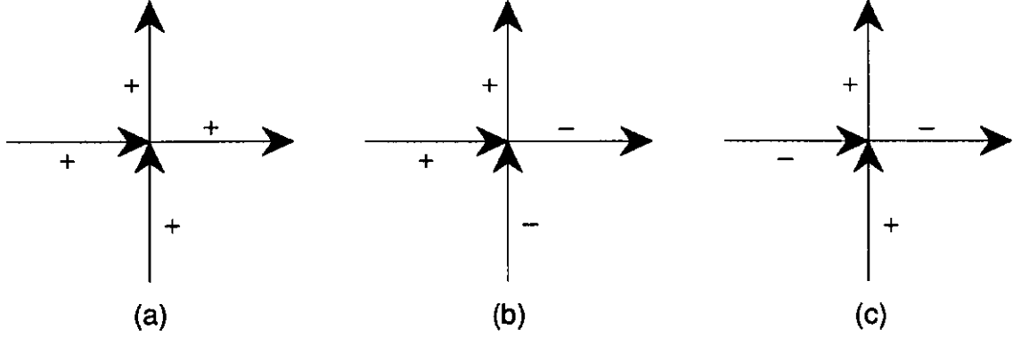
Fig. 2. Up to an overall change of sign, the figures 2(a)-(c) denote the anomaly-free vertices allowed for the action \tilde{I}_{TL} . The signs correspond to Wess-Zumino coupling \pm k , where k is a positive integer.
