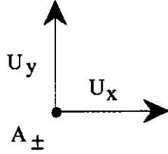
Fig. 1. The degrees of freedom associated with each site \vec{x}_\perp are the 2-D gauge fields A_\pm(\vec{x}_\perp) , and the link fields U_x(\vec{x}_\perp) and U_y(\vec{x}_\perp) , defined on the links as in fig. 1.
