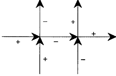
Fig. 4. For the bilocal model, each gauge field A_\mu(\vec{x}_\perp^\pm) interacts with seven links. Figure 4 shows the case where \vec{x}_\perp^+ is to the right of \vec{x}_\perp^- .
