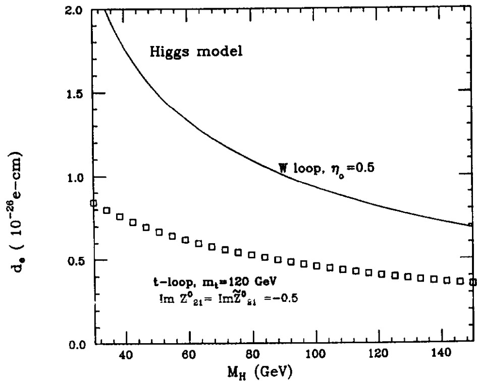
FIG. 2. Numerical estimate of the d_e/e via the W -loop when \eta_n = \frac{1}{2} . The data points show the contribution due to the top quark loop for the case \text{Im}Z_{21}^0 = \text{Im}\tilde{Z}_{21}^0 = -\frac{1}{2} and m_t = 120 GeV.
