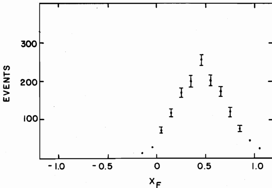
Figure 3. Acceptance in Feynman-x. Dimuons were generated with m = 9.5 GeV, p_T = 0 , and a flat x_F distribution. Reconstructed value of x_F is plotted.
