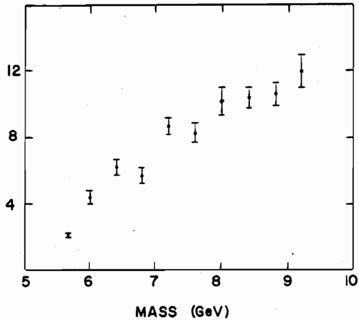
Figure 2. Mass acceptance as calculated by Monte Carlo program. The generated x_F and p_T distribution was (1 - |x|)^2 e^{-p_T^2/1.8} .
