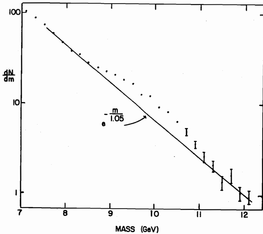
Figure 4. Dimuon mass spectrum after correction for acceptance. There are \sim 2700 events in the upsilon peak.
