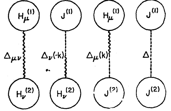
FIG. 2. Diagrammatic representation of Eq. (6.7).
