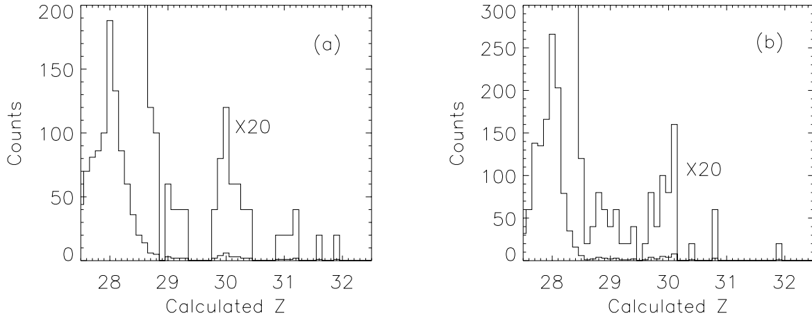
Figure 1: Total counts in the SIS instrument during the November 6, 1997 event, with various cuts: (a) particles in range 0; (b) particles in ranges 1 through 5.
