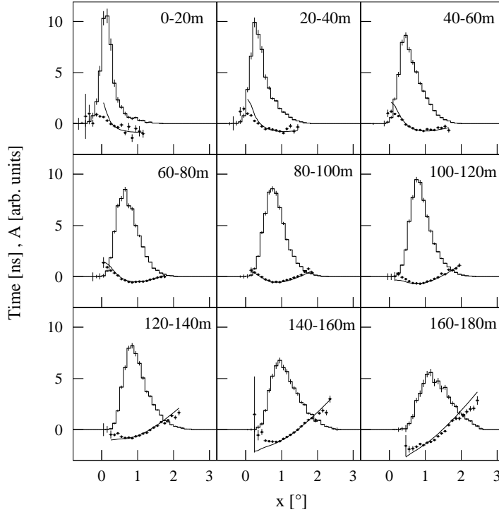
Figure 2: Longitudinal time profiles t(x, 0) of \gamma -ray images, for different ranges in core distance (filled points). The profiles correspond to a slice along x through the image, with |y| < 0.1^\circ . Also shown are the corresponding intensity profiles. The smooth lines refer to the simple model for time profiles, using v = c for the shower particles.
