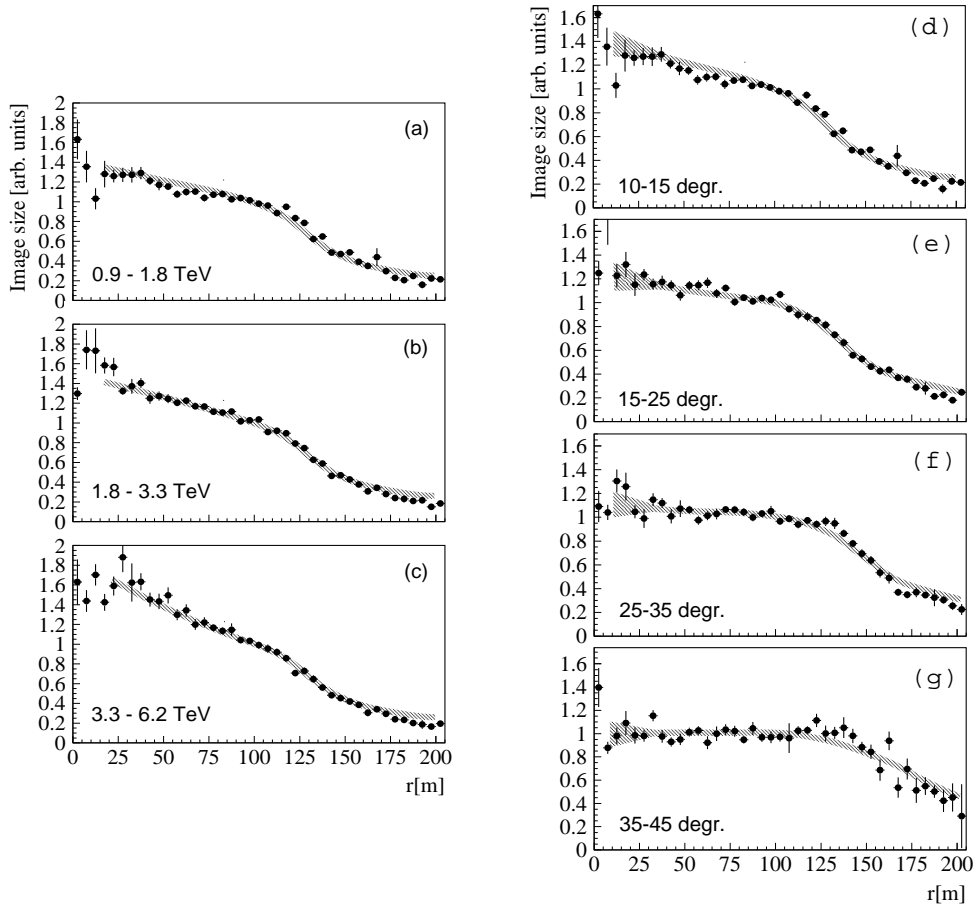
Figure 1: (a)-(c): Light yield as a function of core distance, for image size in the reference telescope between 100 and 200 photoelectrons (a), 200 and 400 photoelectrons (b), and 400 to 800 photoelectrons (c). The corresponding ranges in shower energy are indicated in the figure. (d)-(g) Light yield as a function of core distance, for zenith angles between 10^\circ and 15^\circ (d), 15^\circ and 25^\circ (e), 25^\circ and 35^\circ (f), and 35^\circ and 45^\circ (g). The shaded bands indicate the Monte-Carlo results. The distributions are normalized at r \approx 100 m. Only statistical errors are shown.
