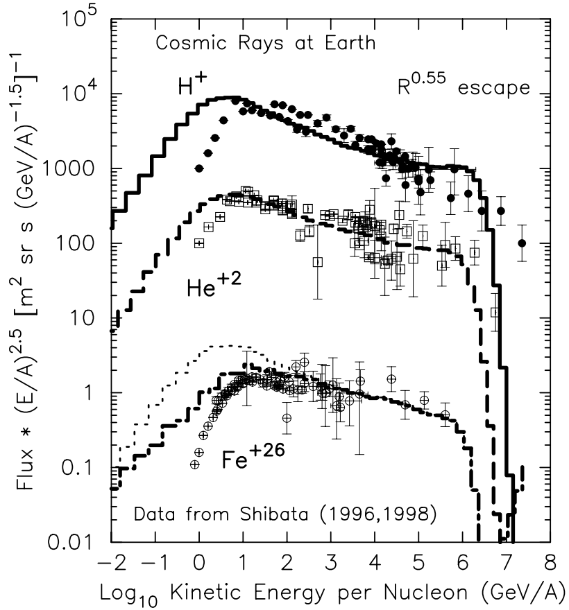
Figure 2: Cosmic ray spectra measured at the Earth (data from Shibata 1996, 1998) compared to model spectra with same parameters as shown in Fig. 1. The model spectra have been multiplied by Rigidity -0.55 to account for escape during propagation and have been normalized separately to match the observations. The light dotted histogram is the model Fe spectrum without nuclear destruction during propagation while the dot-dashed histogram includes nuclear destruction. The turnover in the data below \sim 1 GeV/A is from solar modulation, which is not included in the model.
