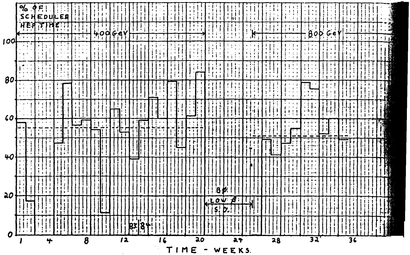
Fig. 1. Tevatron Performance
