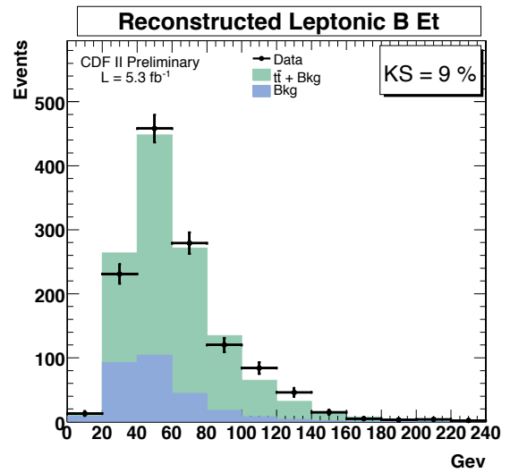
Figure 5.18. Leptonic B et
