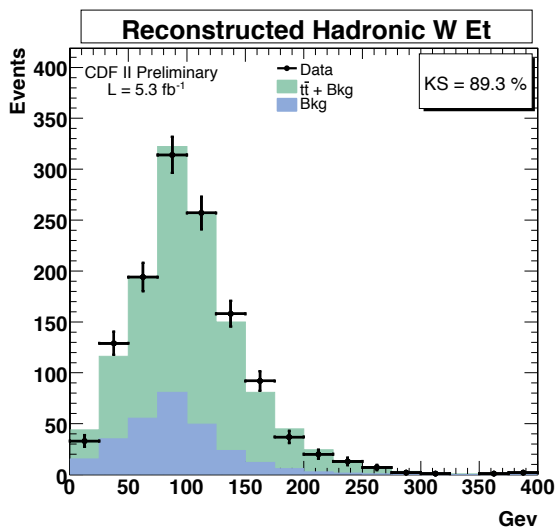
Figure 5.15. Hadronic W et
