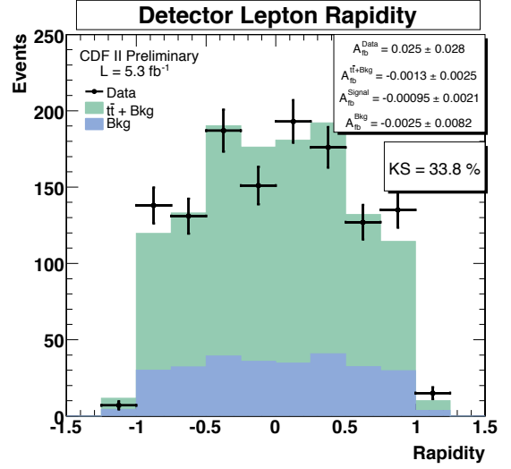
Figure 5.13. Lepton rapidity
