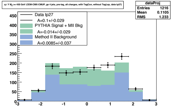
Figure 8.27. The distribution of \Delta y_{lh} at high mass for pre-tag events.
