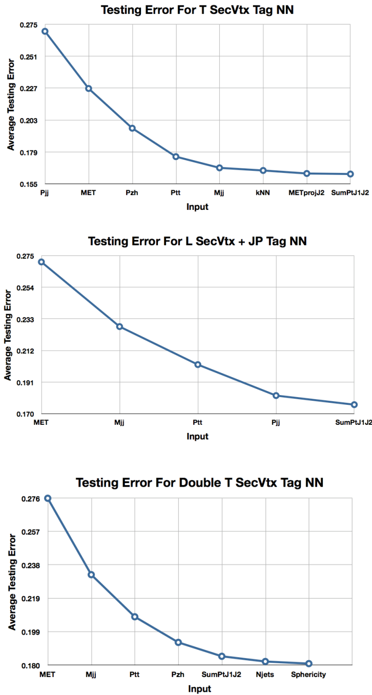
Figure 8.12: The selected NN variables, in order of selection from left to right, and the average testing error produced by their addition.
