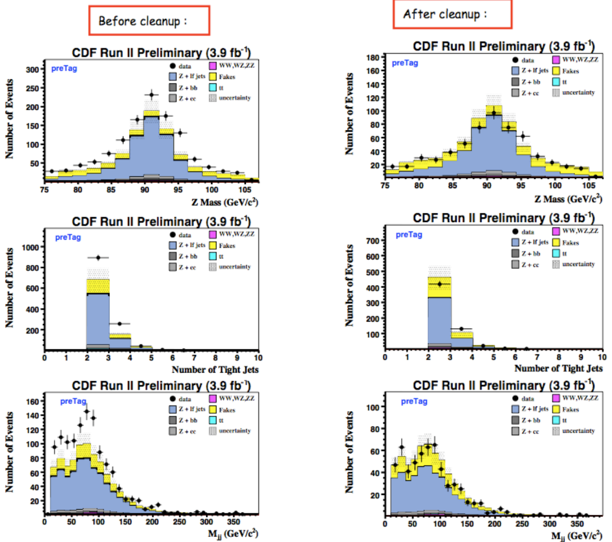
Figure 7.10: Distributions of the Z mass, dijet Mass and Number of tight jets for Lc1Lc1 , LpLp , TpLp , and Lc1Lp Z 's before and after the additional cuts listed in Table 7.25 are applied.
