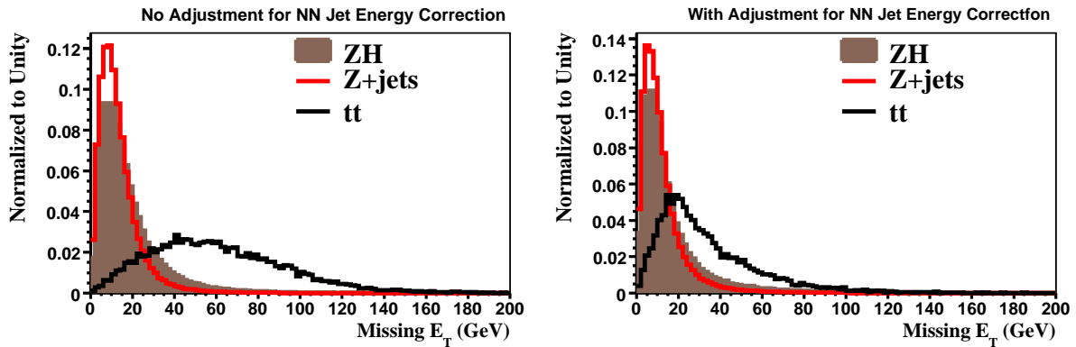
Figure 8.4: The magnitude of missing \vec{E}_T without (left) and with (right) Neural Network corrections. Missing E_T is shown for ZH(brown), t\bar{t} (black) and Z+jets (red) MC.
