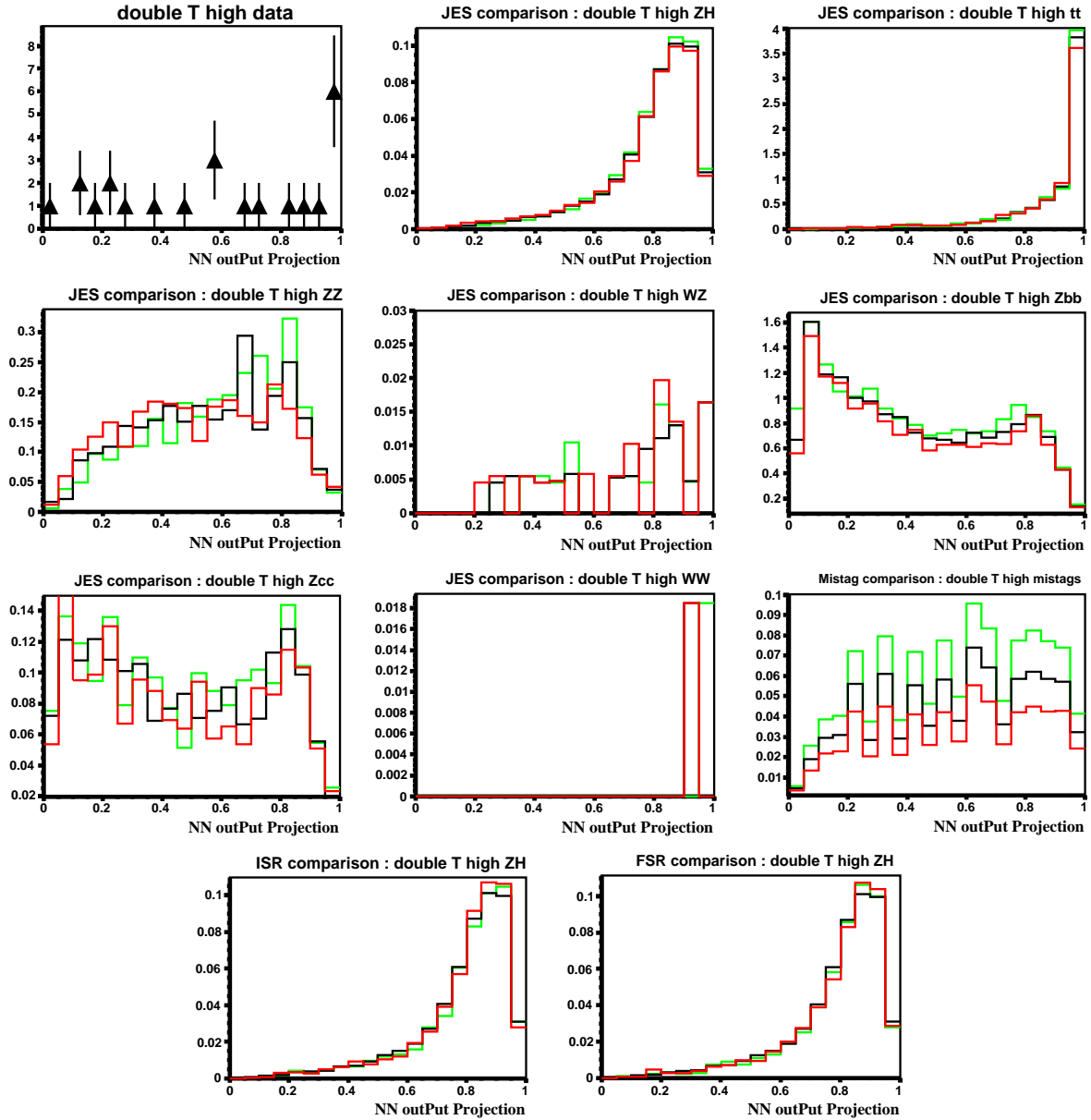
Figure 9.3: Projections of templates affected by shape uncertainties used in the calculation of limits for the double tag high S/B category. Green lines show +1\sigma shifted templates, while red lines show -1\sigma shifts.
