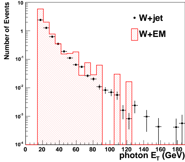
Figure 4.15: E_T distribution of W +jet applied W +jet based fake rate and W +EM object applied W +EM based fake rate after subtracting W\gamma signal contamination.
