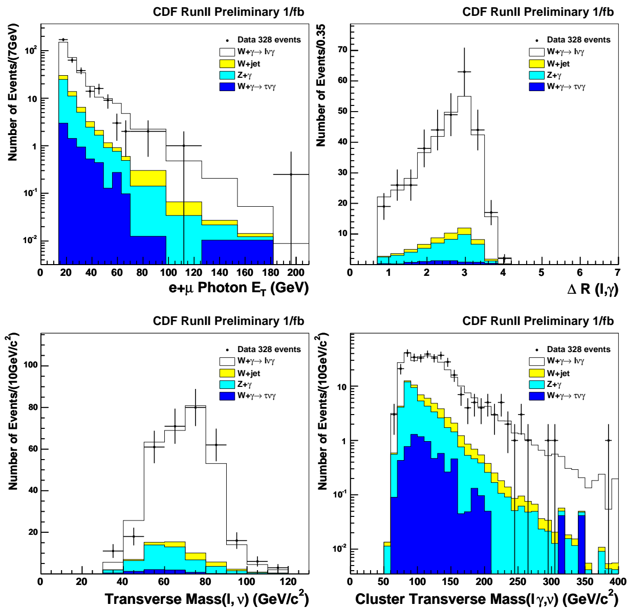
Figure 5.3: Plug photon E_T , \Delta R(\ell, \gamma) , M_T(\ell, \cancel{E}_T) and cluster transverse mass for 1 \text{ fb}^{-1} data.
