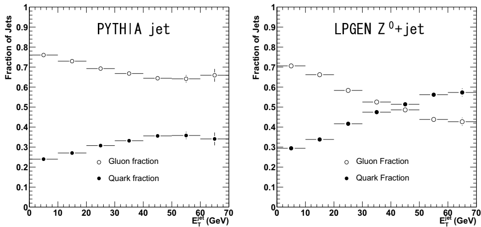
Figure 4.8: Fraction Contribution of Quark and Gluon Jets for PYTHIA jet MC (left) and Alpgen Z^0 +jet MC (right) in central region.
