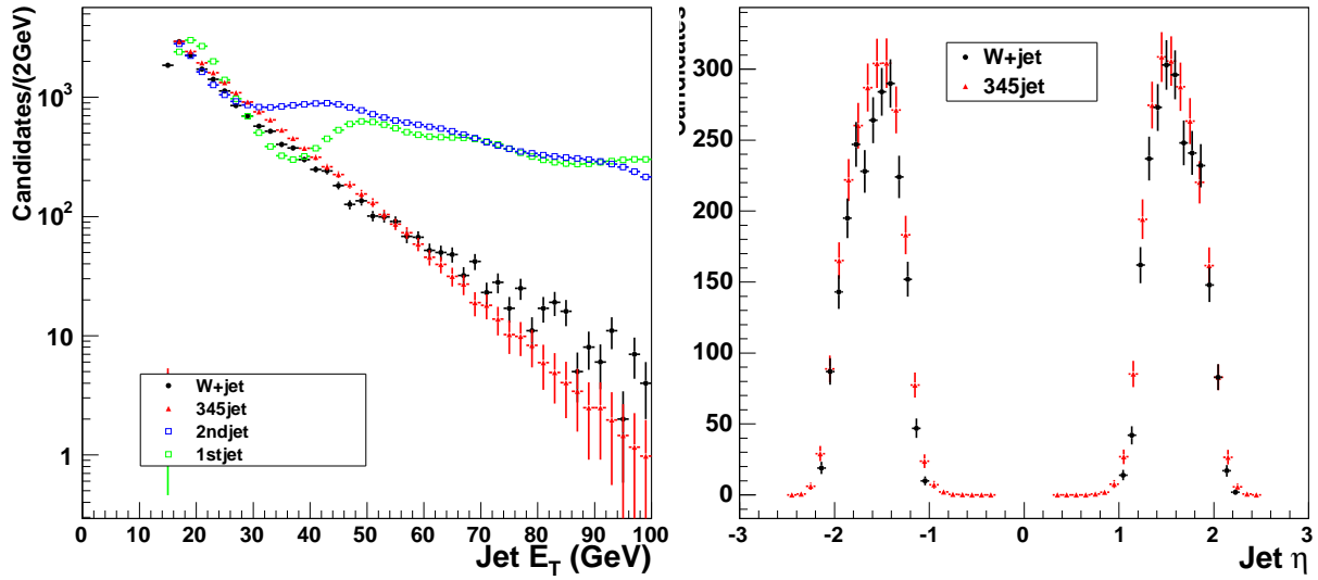
Figure 4.1: The E_T distribution in W sample comparing to the 345th E_T distribution in jet sample (left). Number of events normalized between 15 and 40 GeV. The \eta distribution in W sample comparing to the 345th jet \eta distribution in jet sample (right).
