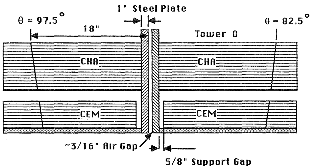
Figure 3.6: The 90^\circ crack, an uninstrumented region near \theta = 90^\circ
