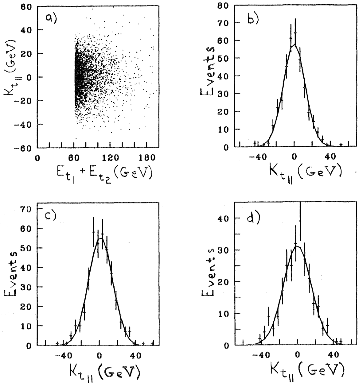
Figure 5.3: K_{t\parallel} distributions. a) A scatter plot of K_{t\parallel} versus the sum of the two leading jets E_t . b) K_{t\parallel} distribution for 75 < E_{t_1} + E_{t_2} < 79 GeV fit to a Gaussian of width \sigma = 12 GeV. c) K_{t\parallel} distribution for 84 < E_{t_1} + E_{t_2} < 91 GeV fit to a Gaussian of width \sigma = 13 GeV. d) K_{t\parallel} distribution for 102 < E_{t_1} + E_{t_2} < 117 GeV fit to a Gaussian of width \sigma = 15 GeV.
