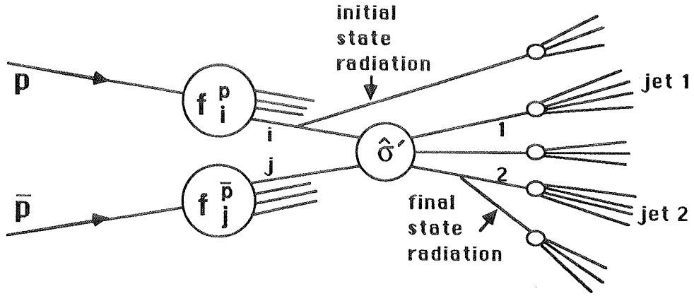
Figure 2.5: The parton model of \bar{p}p collisions, schematically modified to account for energetic initial state radiation , energetic final state radiation , and higher order processes (such as 2 \rightarrow 3 , or 2 \rightarrow 4 , etc.). The final state picture can become quite complicated, but the 2 \rightarrow 2 process is still dominant.
