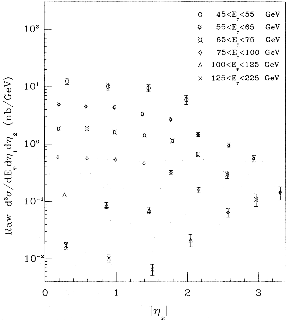
Figure 4.12: The raw two jet differential cross section. The raw cross section, for finding a trigger jet with pseudorapidity within |\eta_1| < 0.6 and E_t within an E_t interval when a probe jet is within a given |\eta_2| bin, is shown for 6 different trigger jet E_t intervals. The raw cross section has not been corrected for resolution smearing.
