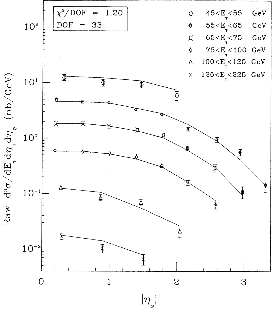
Figure 6.1: The raw two jet differential cross section (points) and a resolution smeared fit (line). The modified SES approximation, in which we parameterized the effective structure function, was smeared with E_t and \eta_2 resolution functions to produce the fit.
