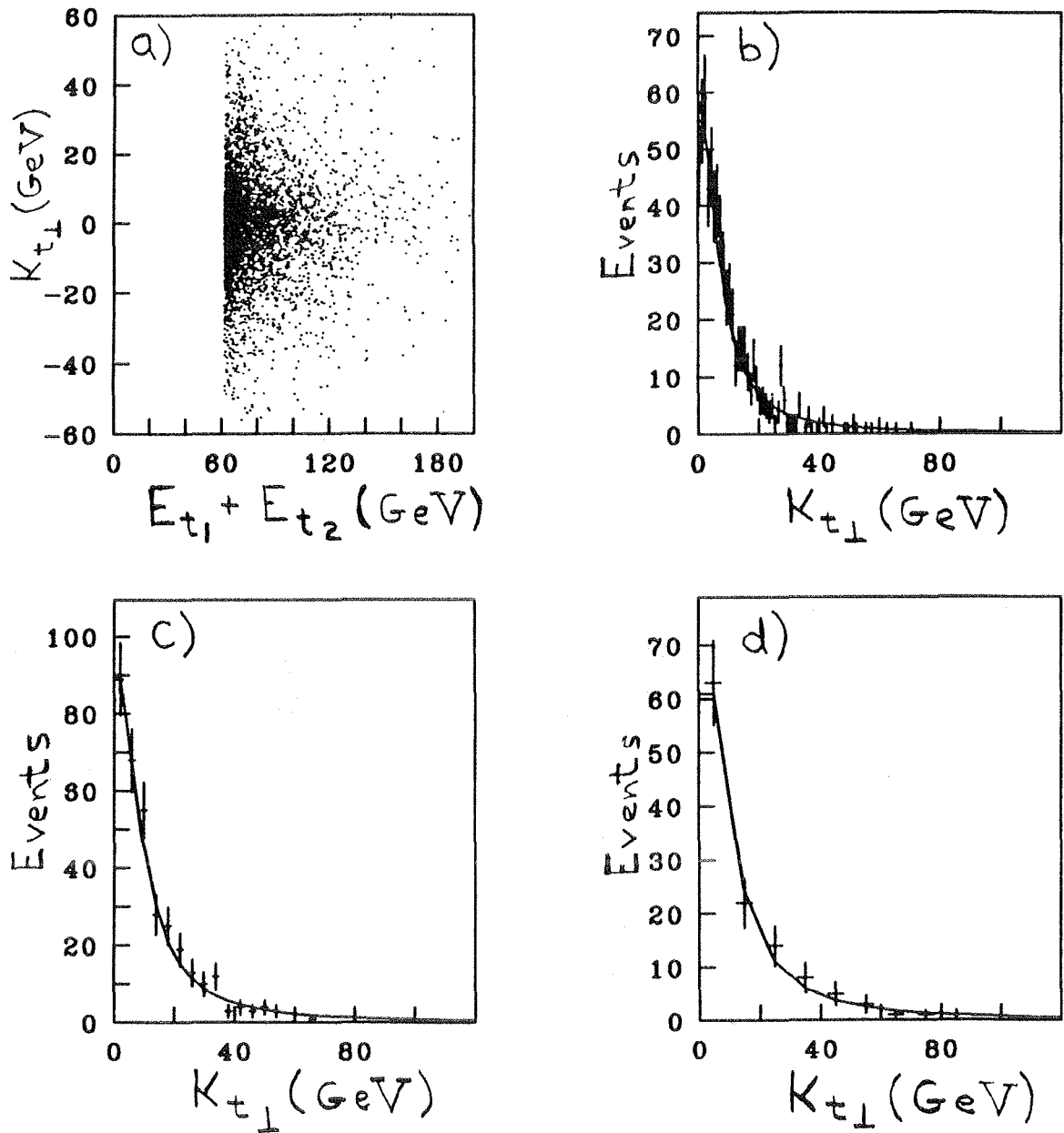
Figure 5.5: K_{t\perp} distributions. a) A scatter plot of K_{t\perp} versus the sum of the two leading jets E_t . b) K_{t\perp} distribution for 80 < E_{t1} + E_{t2} < 90 GeV fit to a Lorentzian with Full Width at Half Maximum \Gamma = 15 GeV. c) K_{t\perp} distribution for 100 < E_{t1} + E_{t2} < 120 GeV fit to a Lorentzian with FWHM \Gamma = 19 GeV. d) K_{t\perp} distribution for 140 < E_{t1} + E_{t2} < 200 GeV fit to a Lorentzian with FWHM \Gamma = 21 GeV.
