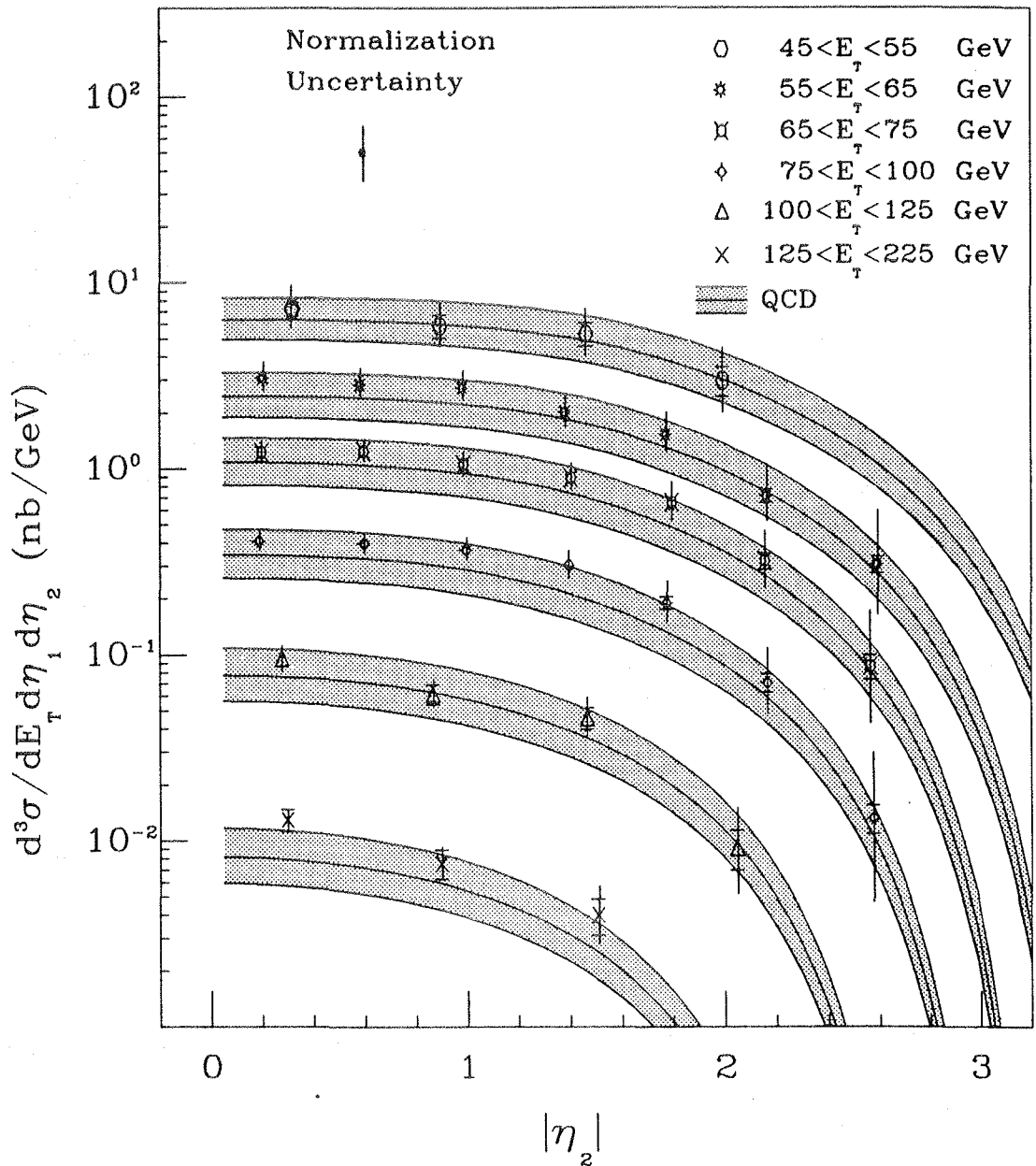
Figure 6.4: The measured and corrected two jet differential cross section (points) compared to a lowest order QCD prediction (shaded). Outer error bars include E_t and |\eta_2| dependent systematic uncertainties and statistical uncertainties (inner error bars). An E_t and |\eta_2| independent systematic uncertainty, common to all points, is shown as the overall normalization uncertainty. The QCD prediction uses EHLQ set 2 structure functions, and was calculated for three different values of Q^2 : the upper curves in each band are for Q^2 = E_t^2/4 , the middle curves are for Q^2 = E_t^2 , and the lower curves are for Q^2 = 4E_t^2 .
