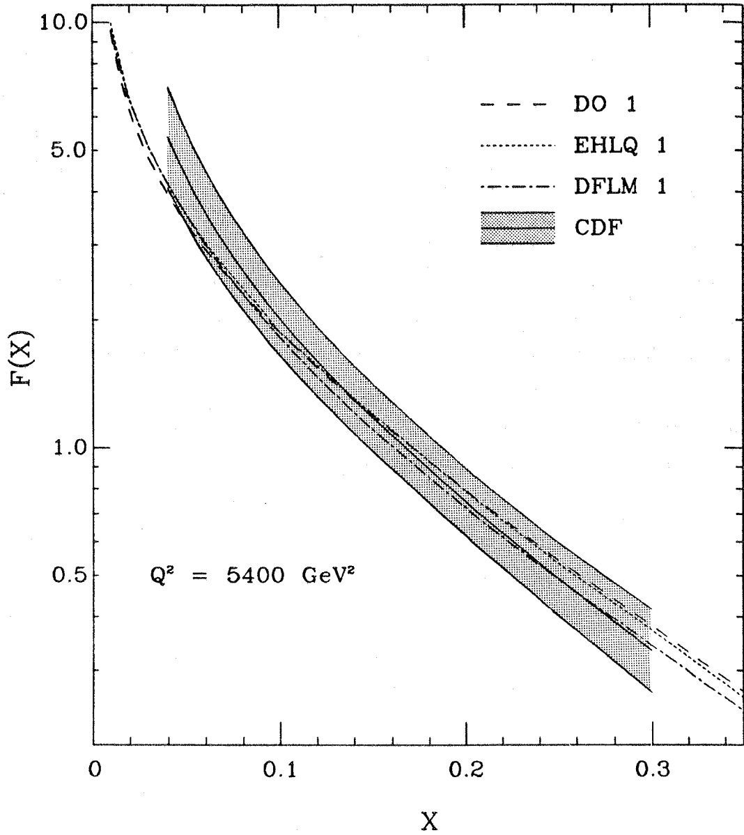
Figure 6.7: Our result for the proton effective structure function (band labeled CDF), is compared to predictions for F(x) = G(x) + \frac{4}{9}(Q(x) + \bar{Q}(x)) from QCD evolutions of deep inelastic scattering measurements.
