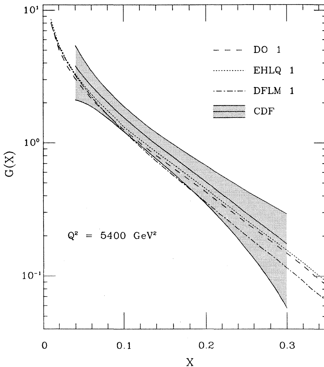
Figure 6.9: An estimate of the gluon structure function (band labeled CDF) compared to predictions from QCD evolutions of deep inelastic scattering measurements.
