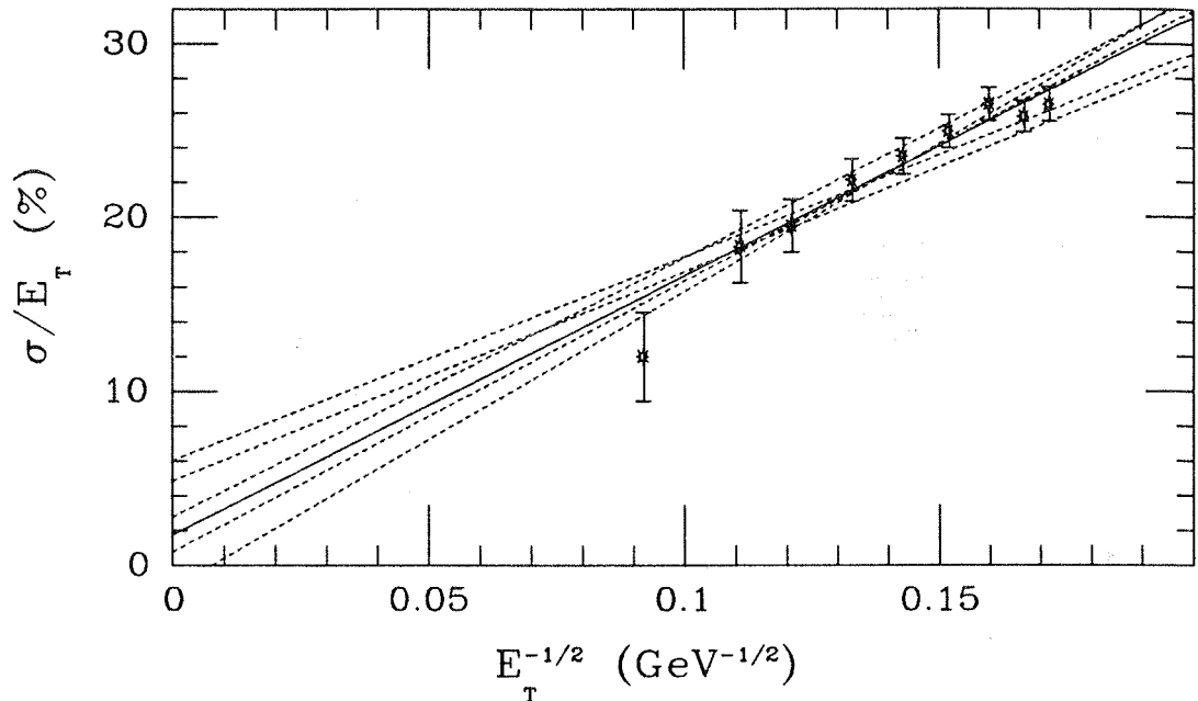
Figure 5.4: The Gaussian E_t resolution of the two jet system, including the effects of QCD radiation, fit with a straight line (solid) as a function of 1/\sqrt{E_t} . The dotted lines are estimates of systematic bounds on the resolution function.
