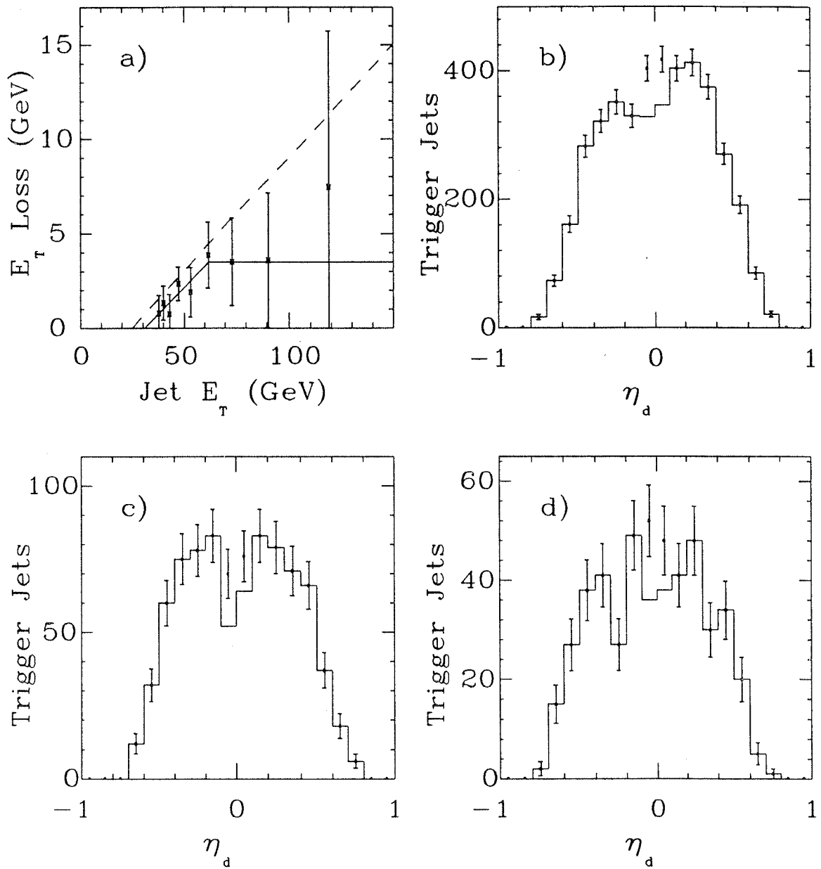
Figure 4.5: a) The transverse energy lost by a jet in the 90° crack (points) as a function of jet E_t . Also shown is the crack correction (solid) and an upper systematic bound (dashed). Plots b) , c) , and d) show the detector pseudorapidity distributions of trigger jets before (histogram) and after (points) crack correction for the medium, high, and burn trigger threshold respectively.
