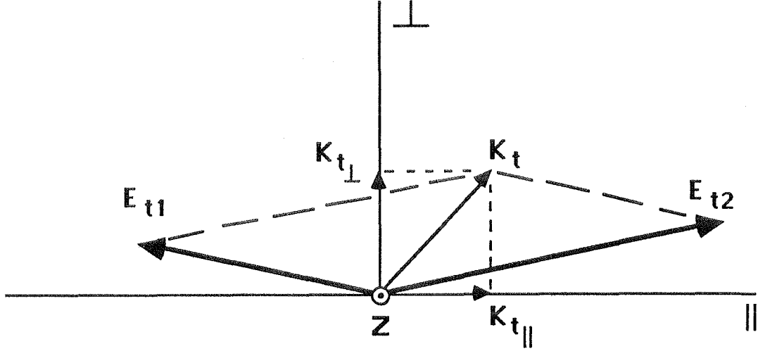
Figure 5.1: The E_t balance technique. The E_t vectors of two leading central jets in the transverse plane are shown. The \perp axis is the perpendicular bisector of \phi_{12} (the azimuthal angle between the two jets). The \parallel axis is orthogonal to the \perp axis in the transverse plane. K_t , the vector sum of E_{t1} and E_{t2} , is shown with its component along the parallel axis, K_{t\parallel} , and its component along the perpendicular axis, K_{t\perp} .
