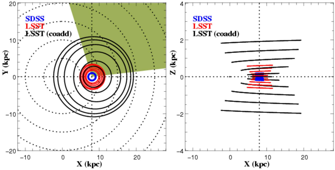
Figure 7.6: This plane-parallel view of the Galaxy ( left ) taken at Z=0.0 kpc (the Galactic plane) is used to illustrate the dust mapping limit at specific Galactic latitudes for the SDSS ( blue ), single epoch LSST observations ( red ), and the full LSST survey ( black , assuming 100 visits in g ). The survey limits at |b| = 0, 2, 4, 6, 8, and 10^\circ are computed using the vertical and radial exponential scale Galactic dust model described in § 3.7.1. The projected positions of the Galactic center and the Sun are at X = Y = 0 and X = 8 kpc, Y = 0 , respectively. The shaded region indicates the portion of the Galactic plane north of \delta = 34.5^\circ limit of the survey. The survey limits are shown on the right in projection onto the X - Z plane to illustrate the ability of LSST to probe structures several kpc above the Galactic disk at significant distances within the plane.
