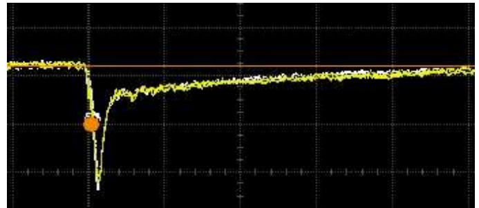
Fig. 2. Superposition of the outputs at the field strengths of 0T (white) and 2.3T (yellow). The scale is 50mV per cell on vertical axis and 50ns per cell on horizontal
