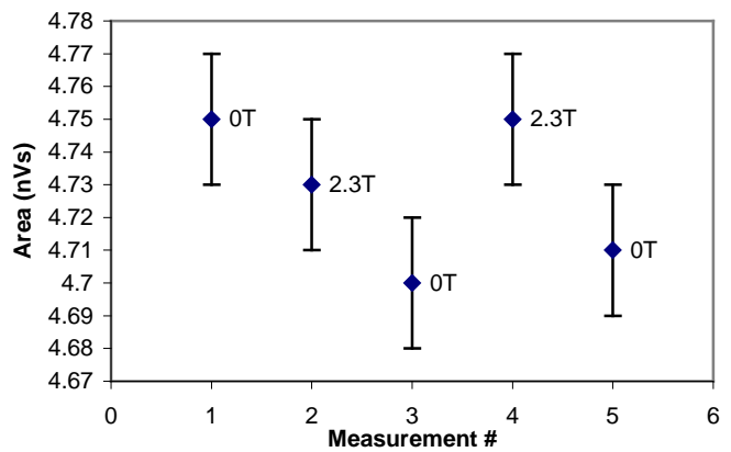
Fig. 3. Area of the MRS output for Bivar UV LED.
