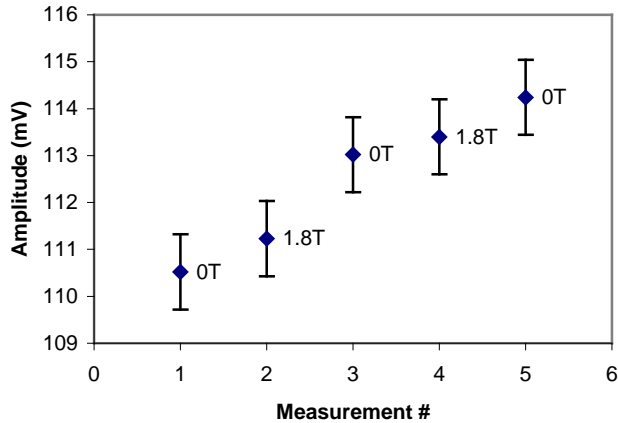
Fig.8. Amplitude of the MRS output for extruded scintillator.
