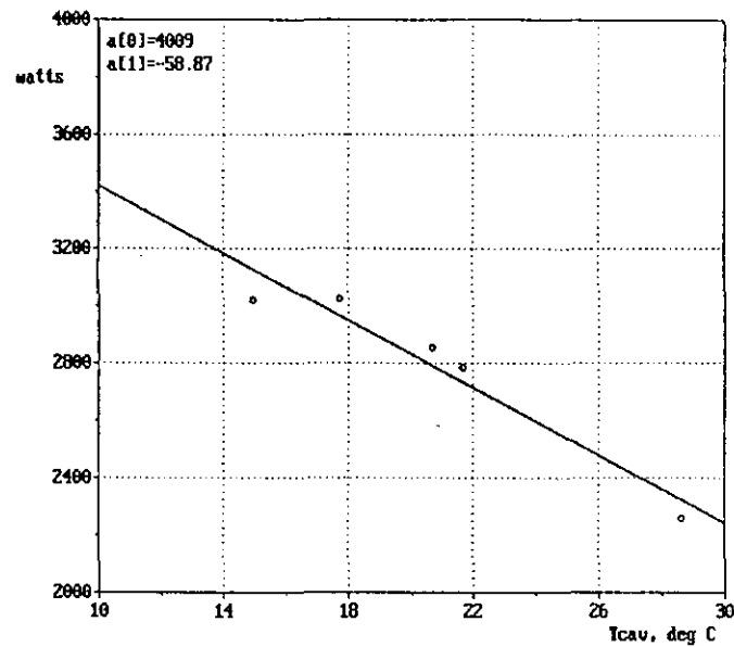
Figure 7. Required cooling power versus cavity temperature, input power is 2.4 KW.
