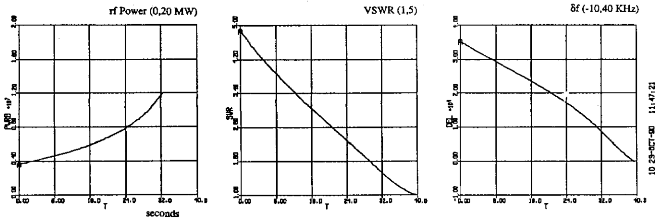
Figure 2. RF power, VSWR, and frequency error versus time during turn on.
