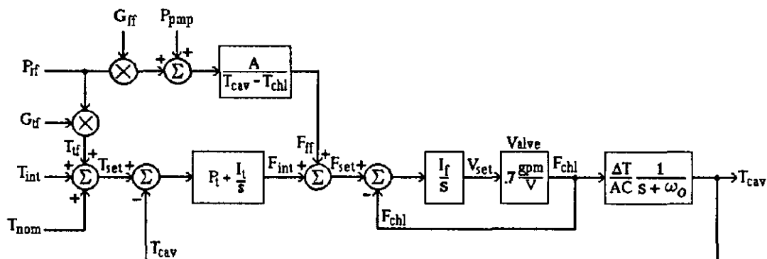
Figure 11. Block diagram of Temperature control loop.
