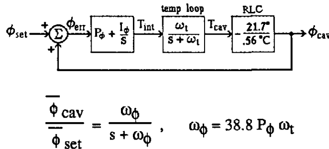
Figure 14. Block diagram of frequency control loop.
