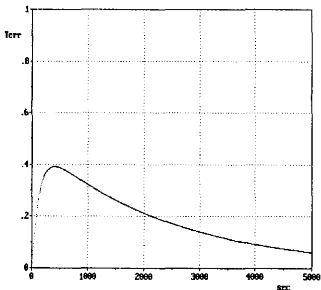
Figure 9. Cavity temperature error in response to a 3.2 KW, or .87 gpm, step change.
