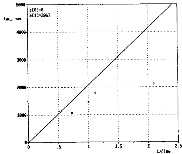
Figure 6. Measured time constant, a_2 = AC/F , versus 1/F for step changes in flow.
