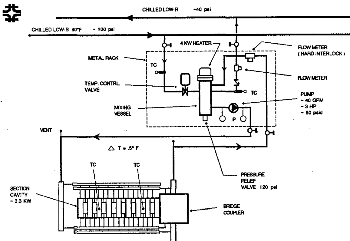
SCHMATIC OF TYPICAL ONE SECTION CAVITY TEMPERATURE CONTROL SYSTEM
