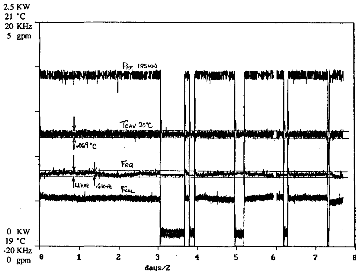
Figure 12. Temperature regulation of a 16 accelerating cell section.
