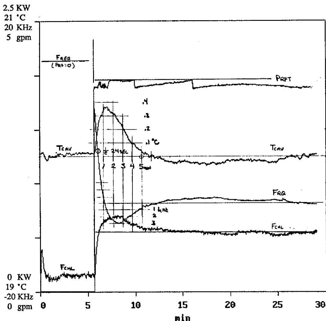
Figure 13. Transient temperature error caused by a 2 KW step change in rf power.
