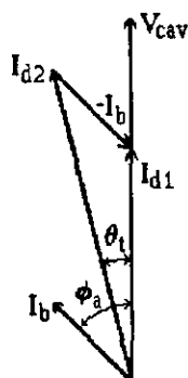
Figure 1. Vector diagram of cavity voltage, rf drive current, and beam current.
