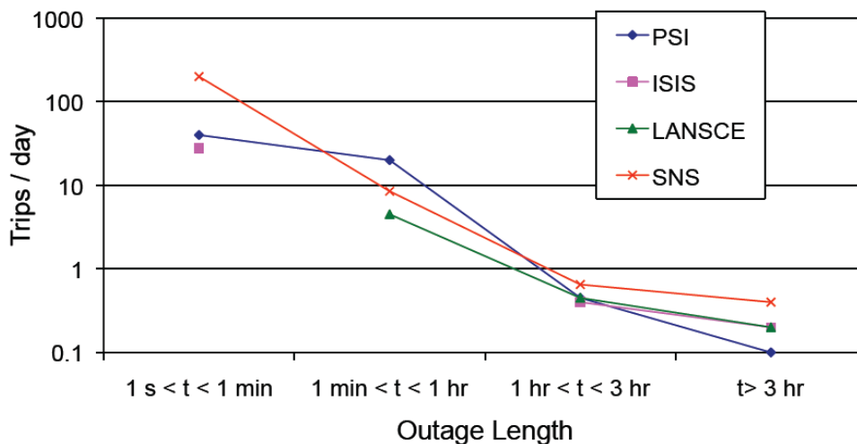
Figure 2: Beam trip frequency for operating high-power proton accelerators [19].
