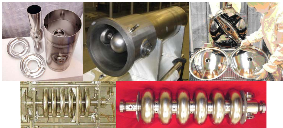
Figure 1: Superconducting accelerating structures for proton and ion beams. Structure types shown include half-wave, quarter-wave, spoke and elliptical resonators.
