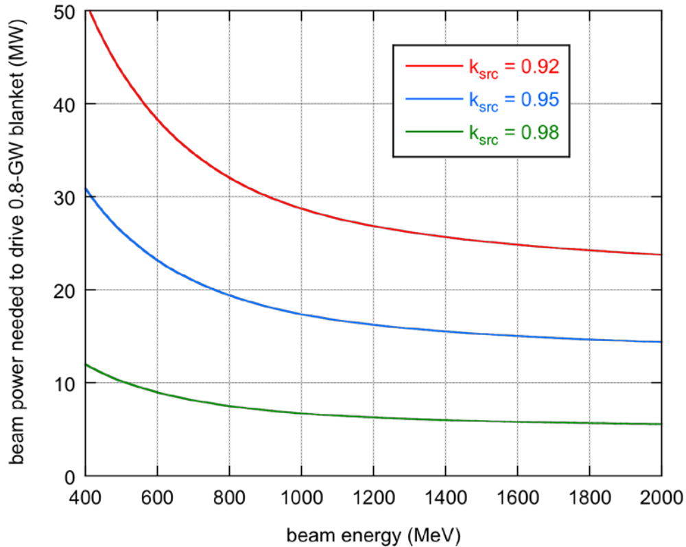
Figure 3. Beam power needed to drive a 0.8-GW ADS sub-critical core as a function of beam energy, for several values of core reactivity, k_{src} (assumes a 50-cm-diameter LBE spallation target).
