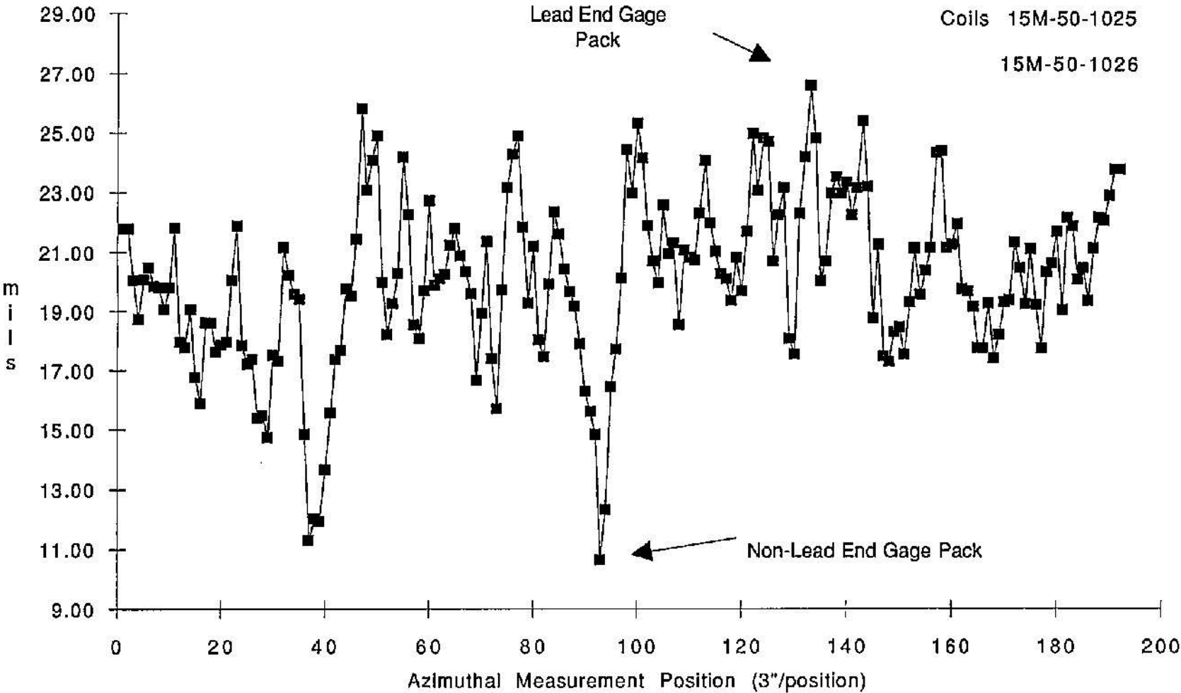
Summed Azimuthal Measurements vs. Longitudinal Position for DCA322
