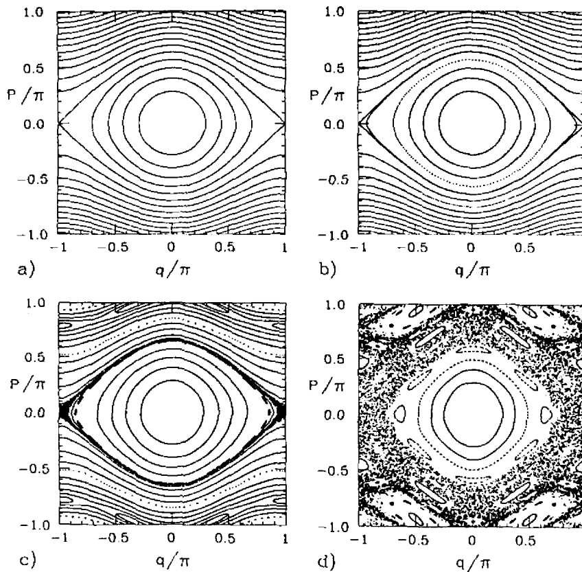
Figure 3. Standard map trajectories, with four different synchrotron tunes, Q_S , corresponding to different integration time steps, \Delta T . a) Contours of the Hamiltonian H = (P^2/2) p^2 - \cos(q) , representing the differential pendulum. b) Q_S = 0.06 . Almost indistinguishable from a), with no sign of chaos, even close to the “separatrix.” c) Q_S = 0.12 . A narrow chaotic region appears near the “separatrix,” and some secondary islands appear. d) Q_S = 0.18 . Most of phase space is chaotic, surrounding complex island structures.
