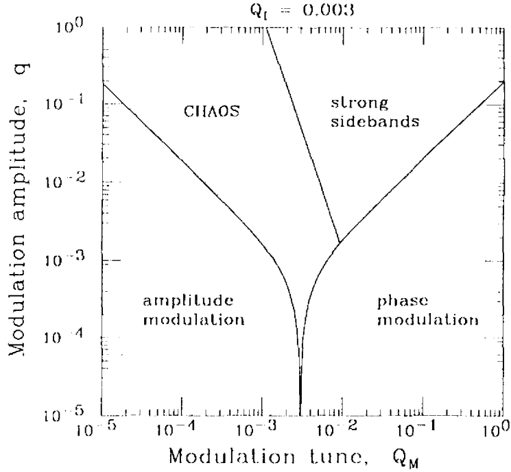
Figure 6. Dynamical behavior in different regions of the tune modulation parameter space (Q_M, q) , for a value of Q_I = 0.003 . The dotted line shows the region accessible to the E778 experiment, extending beyond the resonance pole at Q_M = Q_I for this particular value of the island tune, which is relatively small.
