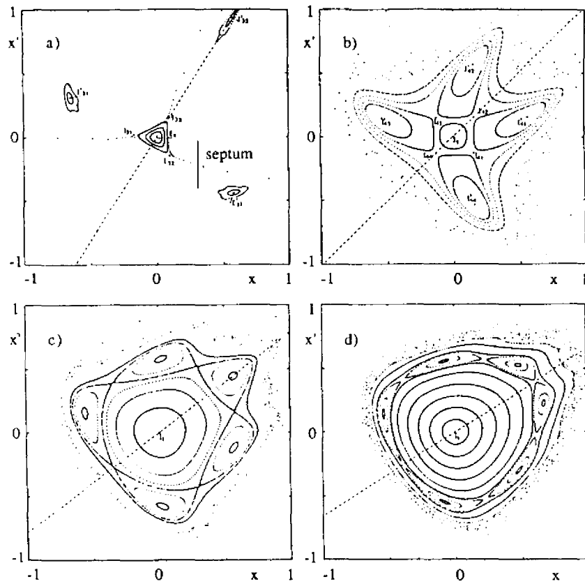
Figure 4. Trajectories obtained by Henon[41] from iterating his map with different base tunes, Q_0 . When Q_0 = 1/n , n resonance islands appear. a) Q_0 = 0.324 \approx 1/3 . The stable triangle and the divergent arms are well described by first order theory, but the outlying islands are not. b) Q_0 = 0.2516 \approx 1/4 . Four big islands at a small amplitude, with Q_0 very close to 1/4 . c) Q_0 = 0.211 \approx 1/5 . Five islands, surrounded by a stable KAM contour, and then chaos. d) Q_0 = 0.185 \approx 1/6 . The six islands are almost rotationally symmetric - they resemble each other and the standard map structure.
