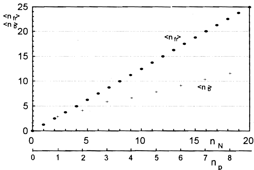
Fig.1. The derived \langle n_f \rangle - n_N and the \langle n_b \rangle - n_p dependences (formulas (8) and (5)), for Ag and Br targets in emulsions. \langle n_f \rangle — the mean number of the heavy fragments — both neutral and electrically charged together, n_N = 0, 1, 2, \dots the multiplicity of the emitted fast nucleons, with kinetic energies of about 20 up to about 500 MeV, \langle n_b \rangle — the mean number of the black track leaving charged fragments; n_p = 0, 1, 2, 3, \dots , the multiplicity of the emitted fast protons
