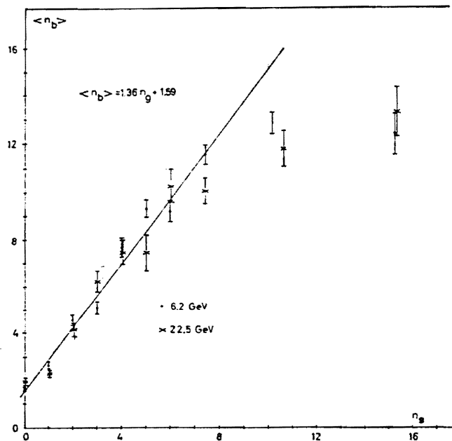
Fig.2. The \langle n_b \rangle - n_g correlation obtained experimentally by H. Winzeler [3]. \langle n_b \rangle is the mean number of the black track leaving particles — the mean number of the charged nuclear fragments; n_g = 0, 1, 2, 3, \dots the multiplicity of the emitted fast protons, mainly with kinetic energies from about 20 up to about 500 MeV
