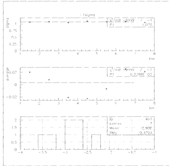
Figura 5.2: PseudoEsperimenti relativi a -1\sigma : \sigma_{pull} (a), pull(b), \delta m (c)
