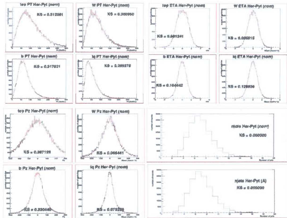
Figura 4.1: Herwig vs Pythia
