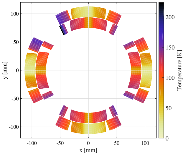
Fig. 5. Protection of the first HL-LHC Nb 3 Sn quadrupole prototype after a training quench just above I_{nom} . The magnet is protected by a combination of OL-H, CLIQ, and EE. Temperature distribution in the coil cross-section at the end of the transient.
