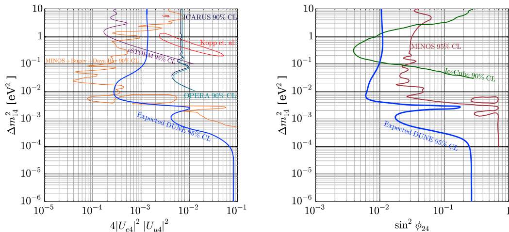
Figure 11.1: Sensitivity of the DUNE experiment to the fourth neutrino hypothesis, updated from [241]. See [241] for details. \Delta m_{14}^2 \equiv m_4^2 - m_1^2 while, in the right-side panel, \sin^2 \theta_{24} \equiv |U_{\mu 4}|^2 .
