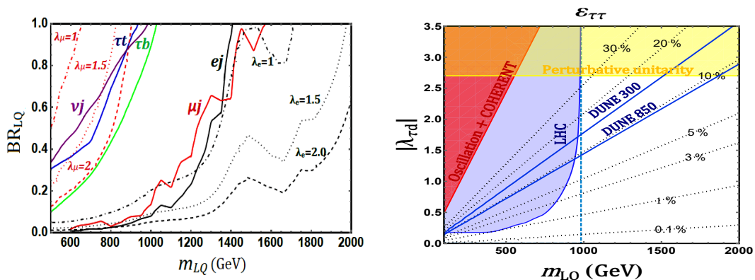
Figure 7.3: Left: LHC constraints on scalar leptoquark from pair and single production. Right: \varepsilon_{\tau\tau} prediction compared with various constraints. The shaded regions are excluded. See text and Ref. [142] for more details.
