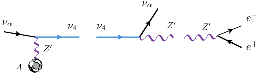
Figure 9.1: Diagram of production of MiniBooNE signature. A heavy neutrino, \nu_4 , is produced via the exchange of a dark photon with the nucleus. For the realization in [185], m_{Z'} < m_4 and the decay chain follows as shown. In the scenario by [211], m_{Z'} > m_4 and the decay chain shown is forbidden; instead once \nu_4 is produced a three body decay into \nu_\alpha e^+ e^- .
