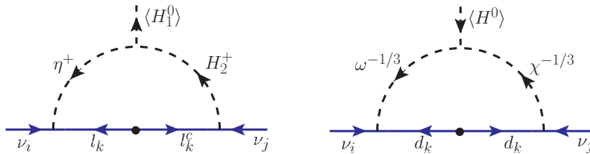
Figure 7.1: Neutrino mass generation at one-loop level: Zee model (left) and a colored variant with leptiquarks (right).
