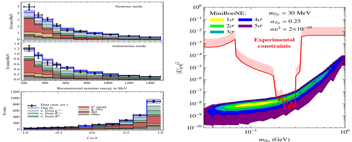
Figure 8.2: Left: The MiniBooNE electron-like event data [159] in the neutrino (top panel) and antineutrino (middle panel) modes as a function of E_\nu^{\text{rec}} , as well as the \cos\theta distribution (bottom panel) for the neutrino data. Note that the data points have only statistical uncertainties, while the systematic uncertainties from the background are encoded in the light blue band. The predictions of our benchmark point m_{N_D} = 420 MeV, m_{Z_D} = 30 MeV, |U_{\mu 4}|^2 = 9 \times 10^{-7} , \alpha_D = 0.25 and \alpha\epsilon^2 = 2 \times 10^{-10} are also shown as the blue lines. Right: Region of our model in the |U_{\mu 4}|^2 versus m_{N_D} plane satisfying MiniBooNE data at 1\sigma to 5\sigma CL, for the hypothesis m_{Z_D} = 30 MeV, \alpha_{Z_D} = 0.25 and \alpha\epsilon^2 = 2 \times 10^{-10} . The region above the red curve is excluded at 99% CL by meson decays, the muon decay Michel spectrum and lepton universality [103, 160].
