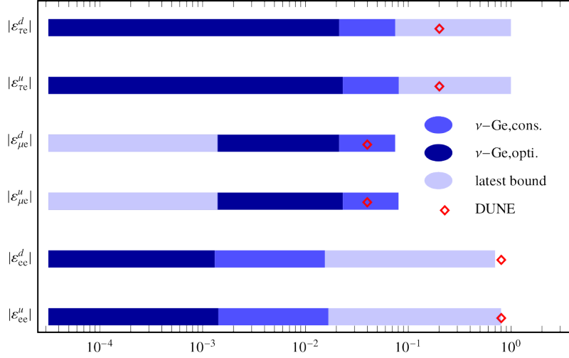
Figure 17.1: Future coherent bounds on NSIs, from Ref. [258].
