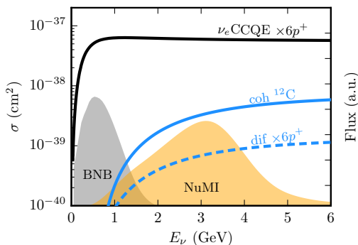
Figure 9.2: Cross section of dark neutrinos at benchmark point. The benchmark point is the same as in [185]. The blue lines correspond to the dark neutrino production cross section: solid blue for the coherent contribution and dashed blue for the diffractive contribution. For reference the \nu_e charged-current quasielastic cross section is shown as a solid black line.
