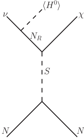
Figure 17.2: A process to produce dark matter in CEVNS proposed in Ref. [260].
