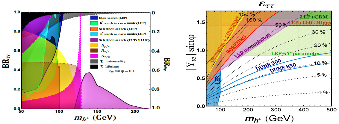
Figure 7.2: Left: Collider constraints on light charged higgs in the Zee model. Right: \epsilon_{\tau\tau} prediction. The shaded regions are excluded. See text and Ref. [142] for more details.
