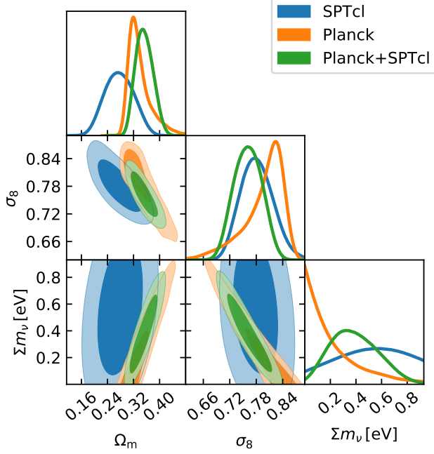
Figure 9. \nu\Lambda CDM constraints on \Omega_m , \sigma_8 , and \sum m_\nu . The SPTcl dataset comprises (SPT-SZ+WL+ Y_X ), Planck uses TT+lowTEB. Note that the cluster data constrain \Omega_m and \sigma_8 almost independently of \sum m_\nu .
