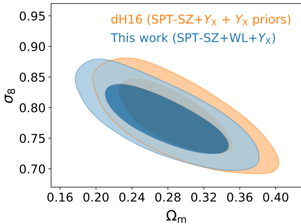
Figure 5. Constraints on \Omega_m and \sigma_8 from this analysis from a previous analysis that used the same cluster sample (dH16). The consistency ( 0.2\sigma ) indicates that our internal mass calibration using WL data agrees with the external X-ray mass calibration priors adopted in dH16.
