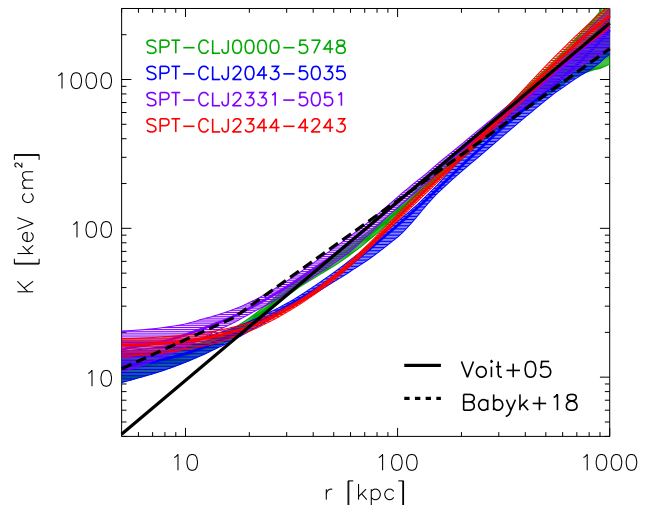
FIG. 5.— The three-dimensional entropy profile is computed combining the model three-dimensional temperature and density profiles ( K \equiv kTn_e^{-2/3} ). These profiles all agree well with one another, and with those from the literature, at large and small radii. We see a weak separation between “high-entropy” (SPT-CLJ0000-5748, SPT-CLJ2331-5051) and “low-entropy” (SPT-CLJ2043-5035, SPT-CLJ2344-4243) systems over the radial range 25–100 kpc, with the two groups merging at smaller and larger radii.
