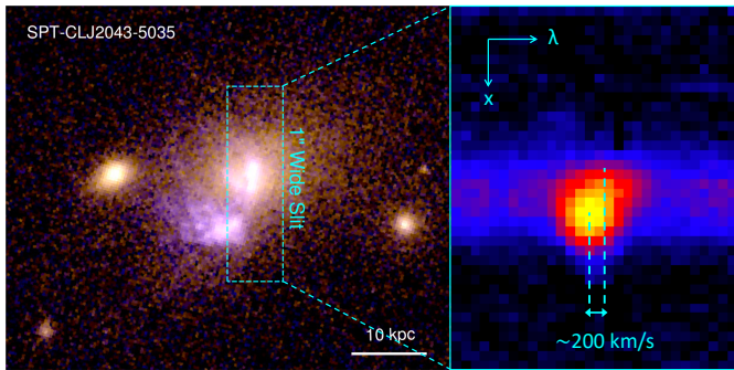
FIG. 9.— Left : Pseudo-color image, combining the F606W and F814W filters on HST, of the central galaxy in SPT-CLJ2043-5035. The cyan rectangle shows the position of the slit that was used to obtain the optical spectrum (Figure 2). Right : Two-dimensional spectrum, extracted along the slit shown in the left panel, and centered on the [O II] \lambda\lambda 3726,3729 doublet. This spectrum shows that the emission peak shifts by \sim 200 km/s over the extent of the extended line emission.
