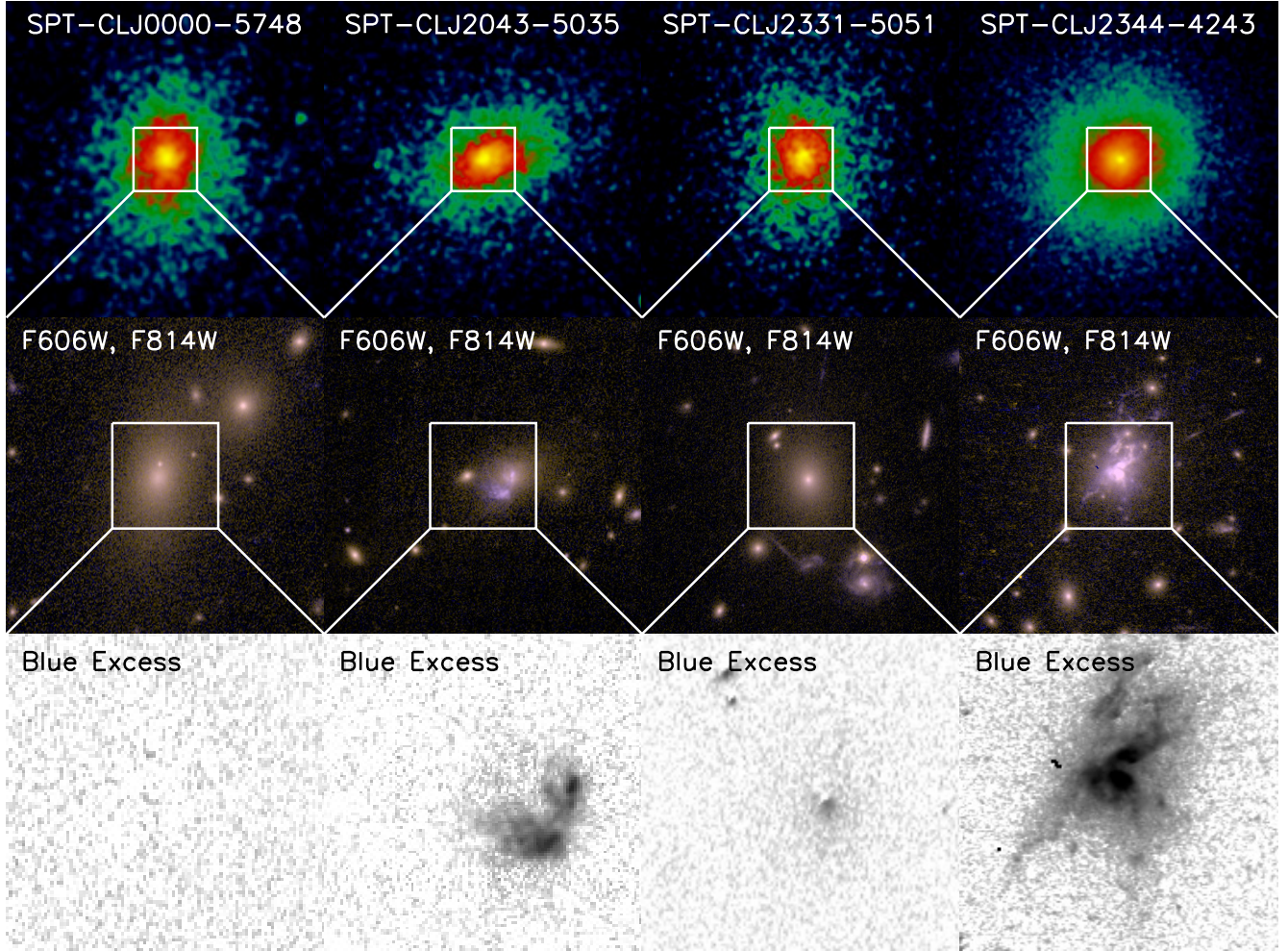
FIG. 7.— Upper row: X-ray image (0.7–4.0 keV) of each cluster, showing the relatively relaxed, centrally-concentrated morphology. Images are 1 Mpc on a side. Middle row: Zoomed-in optical images of the cluster core, showing the central BCG in each cluster. These images are made by combining the F606W (blue) and F814W (green, red) images from HST in such a way as to make the old stellar populations appear red and the young populations blue. Both SPT-CLJ0000-5748 and SPT-CLJ2331-5051 appear relatively quiescent in these colors, while SPT-CLJ2043-5035 and SPT-CLJ2344-4243 clearly have significant younger stellar components. Lower row: Zoomed in image showing the excess emission in the F606W band above the expectation for a passive stellar population, based on the F814W band image. These panels show an absence of emission for the quiescent (based on color) BCGs, and clumpy, extended emission for SPT-CLJ2043-5051 and SPT-CLJ2344-4243. This clumpy, blue emission, which is extended on scales of \sim 15 kpc (SPT-CLJ2043-5051) and \gtrsim 50 kpc (SPT-CLJ2344-4243), is further evidence for ongoing star formation.
