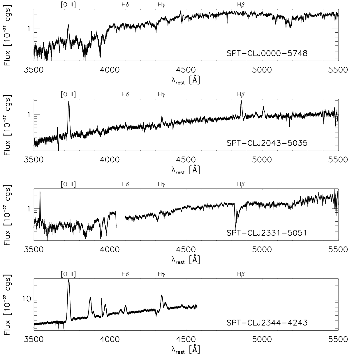
FIG. 2.— Optical spectra for the central, brightest cluster galaxy in each of our four clusters. These systems show a variety of features, including strong [O II] emission (SPT-CLJ2043-5035, SPT-CLJ2344-4243), weak [O II] emission (SPT-CLJ000-5748), strong 4000Å breaks (SPT-CLJ0000-5748, SPT-CLJ2331-5051), and a variety of absorption lines (SPT-CLJ0000-5748, SPT-CLJ2331-5051). For the analysis presented in this work, we consider only the brightness and width of the [O II] \lambda\lambda 3726,3729 doublet relative to the nearby continuum. We note that the missing data in the spectrum for SPT-CLJ2331-5051 is due to a chip gap, and the bright narrow line at \sim 3500Å is a residual sky line. For SPT-CLJ2344-4243 the choice of grating led to sensitivity at \lambda_{obs} < 7350 Å only.
