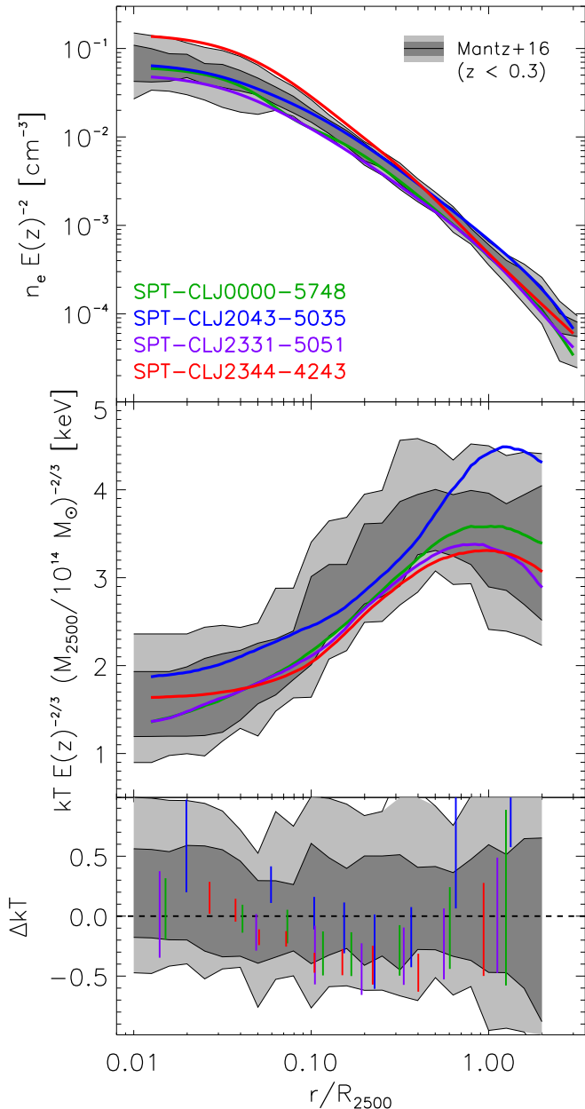
FIG. 4.— In all three panels, we compare the three-dimensional thermodynamic profiles for our four relaxed clusters to those of a similarly-selected sample of relaxed clusters at z < 0.3 from Mantz et al. (2016). The latter are depicted as gray bands, with dark and light bands representing the 1\sigma and 2\sigma scatter. All profiles have been scaled according to the Kaiser (1986) self-similar model, and are plotted as a function of scaled radius ( R_{2500} ). In the lower panel, we show the residual between individual clusters in our sample and the average relaxed cluster at z < 0.3 , demonstrating that, given the measurement uncertainty, all four clusters are consistent with self similar evolution over the past 6 Gyr.
