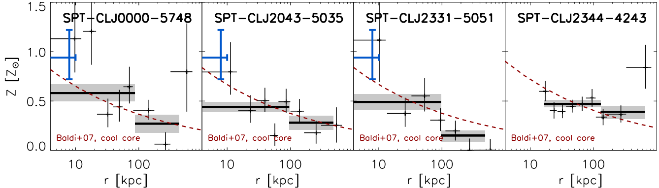
FIG. 6.— ICM metallicity profiles for the four clusters in our sample. Black crosses show the metallicity measured with the same sampling as the temperature profile (see Figure 3). We note that the inner 2.5'' for SPT-CLJ2344-4243 has been masked due to contamination by a bright central X-ray point source with an extremely high equivalent width Fe K\alpha emission line. Thick black lines with grey boxes show the metallicity and its uncertainty measured in annuli of 0 < r < 0.1R_{500} and 0.1R_{500} < r < 0.5R_{500} , following Mantz et al. (2017). Blue points show the joint constraint on the metallicity in the inner 10 kpc from SPT-CLJ0000-5748, SPT-CLJ2043-5035, and SPT-CLJ2331-5051, assuming all three clusters have a shared temperature and metallicity (see §3.2 for more details). We compare these profiles to the average profile for low- z cool core clusters (red dashed line; Baldi et al. 2007), finding that the profiles agree well at all radii, with weak ( \sim 1\sigma ) evidence for a slightly higher than average central ( r < 10 kpc) metallicity in the high- z clusters.
