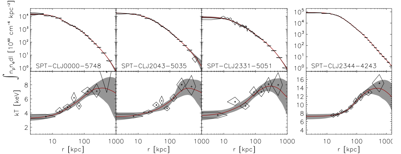
FIG. 3.— Thermodynamic profiles for all four clusters, as described in §2.2. We note that, since SPT-CLJ2344-4243 has a factor of \sim 2 higher mass than the other three systems, we have adjusted the plotting limits for the temperature and density profiles. Upper row: These panels show the emission measure profile for each of the clusters, with sampling chosen to produce a high signal-to-noise, well-sampled profile. This projected profile is fit with a three-dimensional model (see Equation 1), which has been projected along the line of sight and along the radial direction within each bin. All four clusters exhibit a central overdensity, indicative of a cool core. Lower row: These panels show the projected temperature profile, with a coarser sampling that reflects the added complexity of constraining the spectroscopic temperature and metallicity. These profiles have been fit with a three-dimensional model (see Equation 2) which has been projected along the line of sight following Equation 3. All four clusters have similar temperature profiles, reaching a maximum projected temperature at \sim 300 kpc that is \sim 2\times higher than the minimum, projected temperature measured at \sim 10 kpc.
