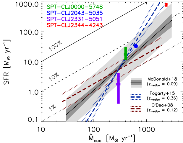
FIG. 8.— BCG star formation rate compared to classical cooling rate ( \dot{M}_{cool} \equiv M_g(r < r_{cool})/t_{cool} ) for the four clusters in our sample. These star formation rates are based on the [O\ II] emission line, and are corrected for intrinsic extinction as measured from the CIGALE fit to the broadband SED. For comparison, we show the relations found in O’Dea et al. (2008, dark red) and McDonald et al. (2018, black/grey) for clusters at z \sim 0.1 . For the latter, we show the uncertainty on the fit in dark grey, and the measured scatter in light grey. In blue, we show the fit to CLASH clusters from Fogarty et al. (2015), which are at considerably higher redshift. Overall, the relaxed clusters in the SPT sample (including Phoenix, (McDonald et al. 2012), which is the most relaxed SPT-selected cluster) tend to host BCGs with higher SFR per unit cooling ICM than clusters at z \sim 0 .
