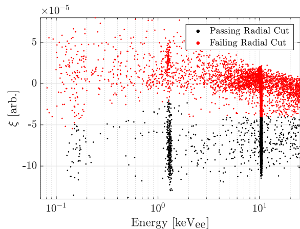
Figure 8. Distribution of the radial parameter \xi vs. energy in the DM search data. An energy-dependent cut on \xi defines the fiducial volume below 2keV ee , while a stricter constant cut is used above 2keV ee .
