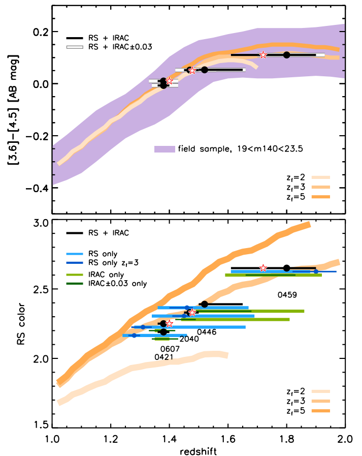
Fig. 5: Photometric redshift constraints for all clusters (black points with 1\sigma errorbars reported in both panels) as determined with the simultaneous modeling of the red sequence (RS) and [3.6]-[4.5] color in Sect. 4. Red stars show the spectroscopic redshifts for SPT-CLJ2040 and SPT-CLJ0607, as well as the best current constraint for SPT-CLJ0459 (see Sect. 4). Bottom panel – Adopted model RS m814-m140 color at M^* vs. redshift, for formation redshifts 2 < z_f < 5 (orange lines). Light blue bars show the 1\sigma constraints from modeling only the RS color (dark blue assuming z_f = 3 ). Light green bars show constraints from the [3.6]-[4.5] color alone. Top – Adopted model [3.6]-[4.5] color vs. redshift, for 2 < z_f < 5 as in the bottom panel. The shaded area shows for reference the 16^{\text{th}} - 84^{\text{th}} percentile range of [3.6]-[4.5] color vs. redshift for field galaxies in the magnitude range of our samples ( m140 \leq 23.5 ). Dark green (bottom panel) and white (top panel) bars show the impact on the best-fit redshift (from IRAC color alone and RS + IRAC color, respectively) of a \pm 0.03 AB mag systematic offset on the [3.6]-[4.5] color.
