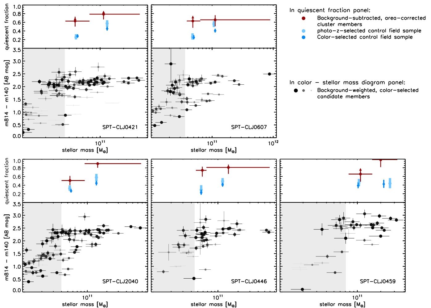
Fig. 7: For each cluster: Bottom panel : m814-m140 color vs. stellar mass of candidate cluster members within r < 0.7r_{500} . Symbol size and color reflect the statistical background subtraction weight as in Fig. 1. The light-gray shading shows the stellar mass range below the mass completeness limit. Top panel : quiescent fraction within r < 0.7r_{500} at masses above the individual mass completeness limit of the cluster (red symbols; error bars show the width of the stellar mass bin and the 1\sigma binomial confidence intervals, see Sect. 5.2). Where applicable, red triangles show quiescent fractions assuming that all unclassified galaxies are quiescent (rather than all star-forming, see Sect. 5.2). Blue symbols show the quiescent fraction in the same stellar mass bins for photo- z and color-selected field samples as in Fig. 1, as indicated. All symbols are plotted at the median mass of the given sample.
