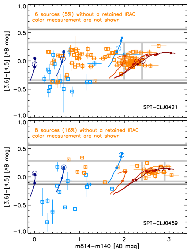
Fig. 2: Two examples of the selection of candidate cluster members (see Sect. 3.1). Vertical gray lines bound the m814-m140 RS sample used for the initial definition of the IRAC color selection range, shown by the horizontal light-gray lines. Groups of red and blue tracks show, respectively, the colors as a function of redshift in the range 1 < z < 2 of quiescent (SSPs with z_f = 2, 3, 5 ) and actively star-forming (100 Myr old constant star formation, A_v = 0, 1, 3 ) stellar populations, used to obtain the final adopted IRAC color selection range (dark-gray lines, see Sect. 3.1 for full details). Small solid points along the tracks indicate z=1.3, 1.6, 1.9 ; the large circle indicates the cluster redshift. Orange and blue squares mark the galaxies in the cluster field classified as candidate members or interlopers, respectively, with the full IRAC+ HST color selection criteria described in Sect. 3.1.
