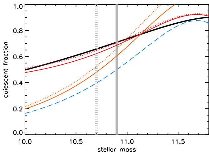
Fig. C.2: Test of the quiescent fraction vs. stellar mass modeling discussed in Sect. 5.4. The black line shows the observed quiescent fraction vs. stellar mass in z \sim 1 clusters from van der Burg et al. (2013). The red and orange solid (dotted) lines (color coding as in Fig. C.1) show the estimated quiescent fraction vs. mass using the two approaches shown in Fig. C.1, starting from the observed quiescent fraction in a mass complete sample with \log(M/M_{\odot}) > 10.9 (10.7, respectively, as shown by vertical gray lines). Blue dashed line shows the field quiescent fractions vs. mass at the same redshift.
