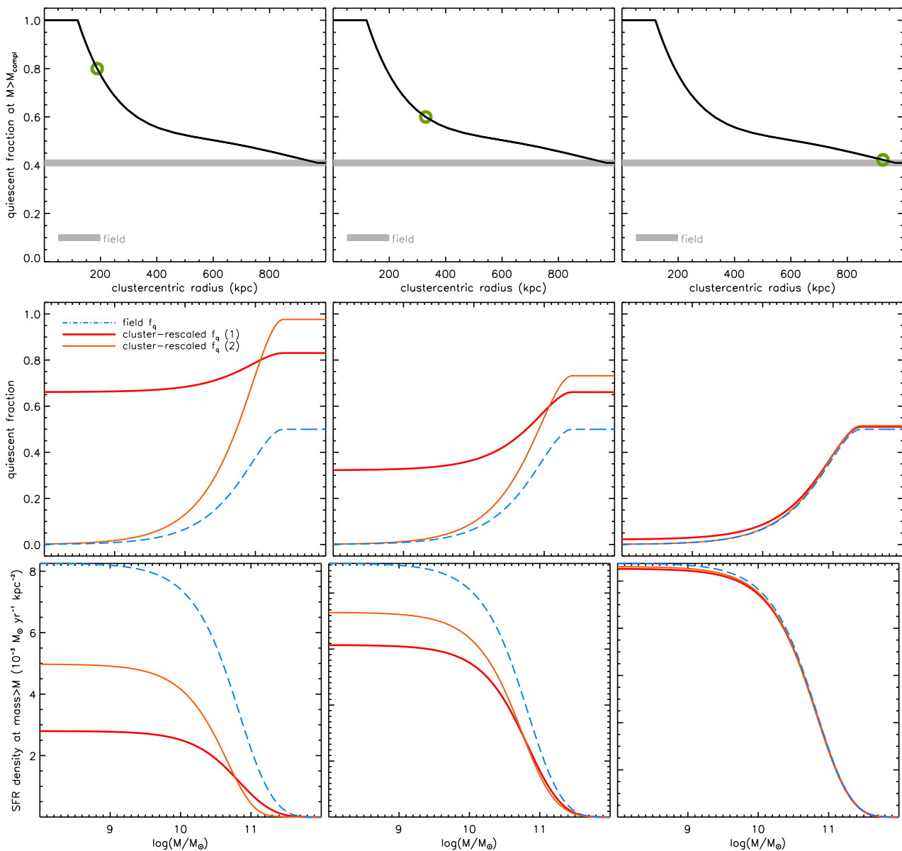
Fig. C.1: Example illustration of the modeling of the quiescent fraction vs. stellar mass. Top panels : The assumed radial profile of the quiescent fraction above mass completeness. In the three panels a green circle highlights a given clustercentric distance, and thus quiescent fraction value. Based on these values, the corresponding middle panels show the quiescent fraction vs. stellar mass as estimated with both approaches described in Sect. 5.4 (red, orange lines). The blue line shows the quiescent fraction vs. mass in the field at the cluster redshift. The corresponding bottom panels show the overall contribution of galaxies above a given stellar masses to the total SFR density at the given clustercentric distance assuming the quiescent fraction vs. mass from the middle panels (see Sect. 5.4).
