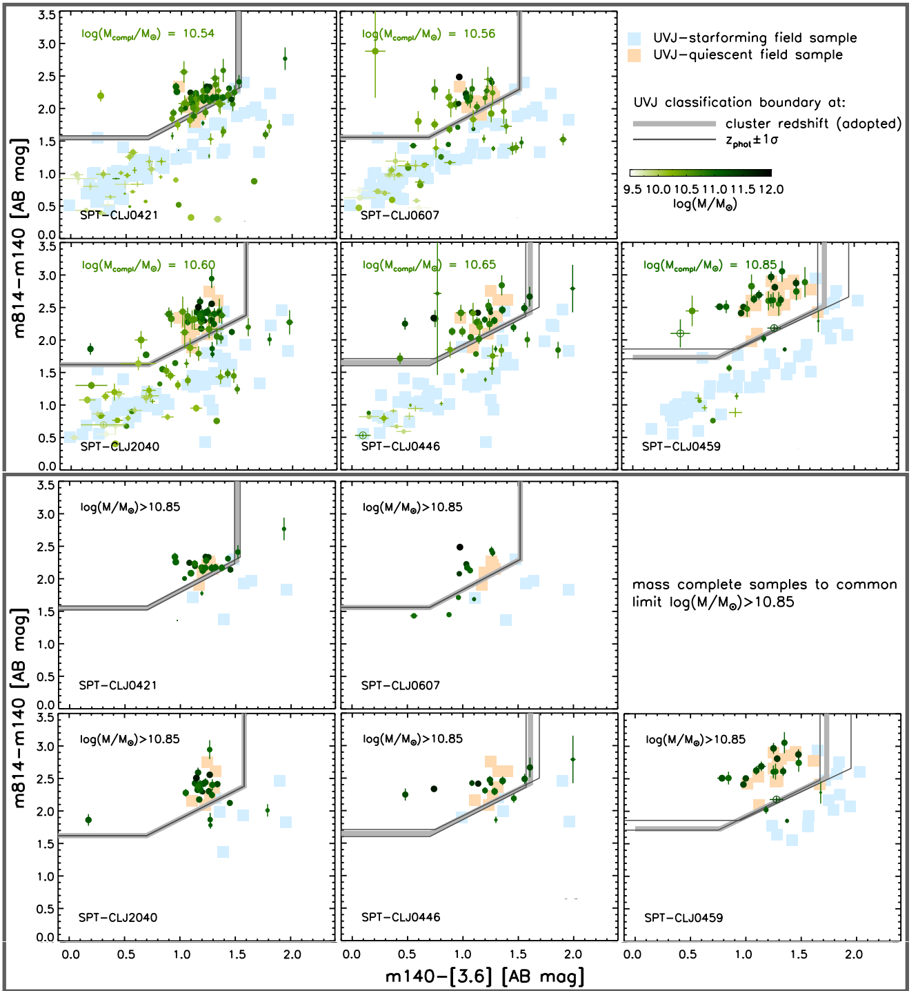
Fig. 6: Adopted quiescent vs. star-forming galaxy classification. The observed m814-m140 vs. m140-[3.6] color-color diagram of candidate members (green points) is shown for all clusters in the r/r_{500} < 0.7 region (the effective area covered for each cluster is indicated). The upper set of panels show m140 -selected (not mass complete) candidate member samples (the mass completeness limit for each cluster is indicated). The lower set of panels show galaxies down to the common stellar mass completeness limit for all clusters, \log(M/M_{\odot})=10.85 . Symbol size of green points scales with the statistical background-subtraction weights as in Fig. 1. Symbol color scales with stellar mass as shown by the color bar. Empty symbols show points for which a m140-[3.6] color was inferred using the 4.5\mu\text{m} flux (see Sect. 5.2). Light red and blue squares show, respectively, UVJ-quiescent and UVJ-starforming galaxies from the control field sample with the same magnitude (top panels) or mass (bottom panels) threshold as candidate cluster members, and with a photometric redshift within \pm 0.1 from the cluster redshift. The thick light-gray line shows the adopted quiescent vs. star-forming separation in the observed m814-m140 vs. m140-[3.6] color plane. For clusters without a final spectroscopic redshift confirmation (see Sect. 4), the thin dark-gray lines show the separation that would be adopted if assuming a redshift at the edges of the black+white error bars in Fig. 5 (top).
