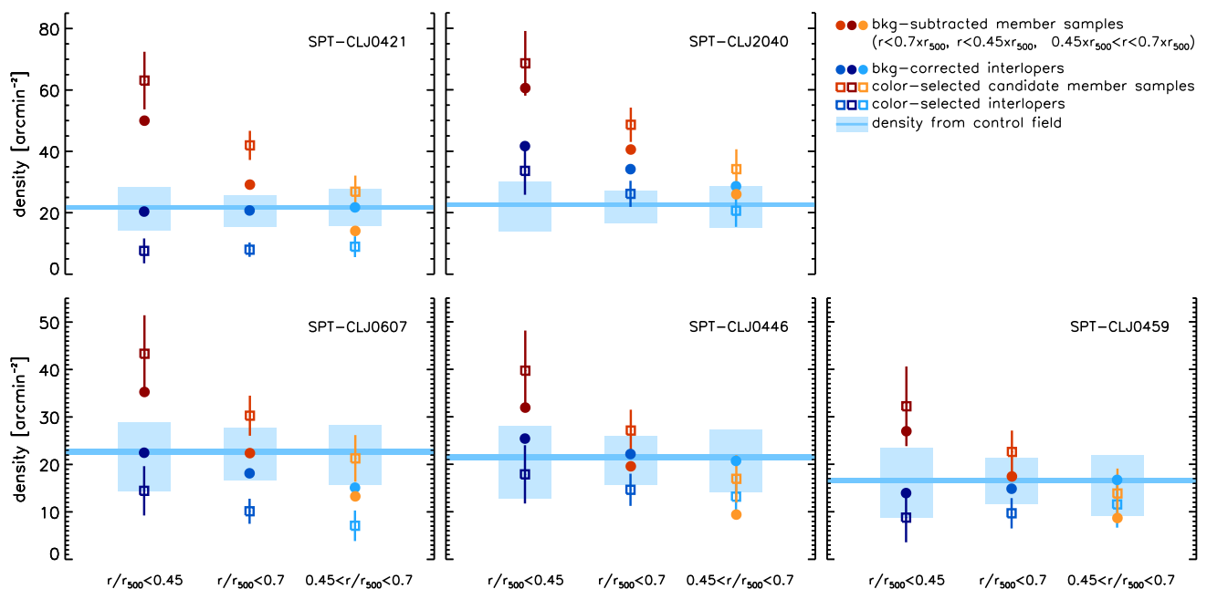
Fig. 3: Projected number density of candidate cluster members (shades of red) and interlopers (blue) in the five clusters as measured in three cluster regions, as indicated. Empty squares show densities for color-selected samples (see Sect. 3.1), and filled circles show how member number density decreases – and interloper density increases – after applying the statistical subtraction of residual background contamination described in Sect. 3.2. The blue line shows the average density of control field galaxies in the same magnitude range adopted for the cluster, with the light-blue shaded areas showing the density variation ( 16^{\text{th}} – 84^{\text{th}} percentiles) in apertures corresponding to the three probed regions. The relative flatness of the interloper density profiles constrains the cluster member sample incompleteness due to member misclassification (see Sect. 3.3).
