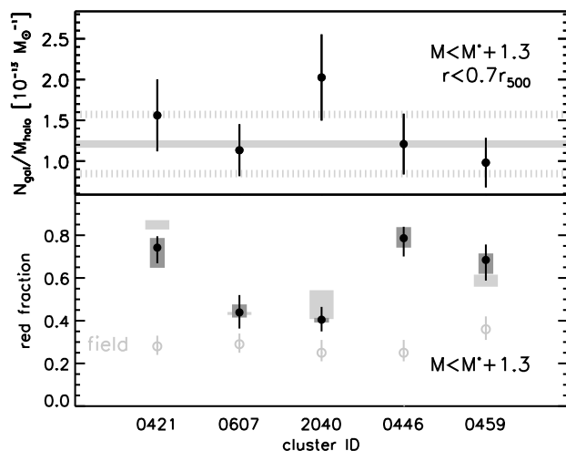
Fig. A.1: Top panel – Black points show for all clusters the estimated total number of background-subtracted cluster members at m_{140} < M^* + 1.3 and within r < 0.7r_{500} divided by the total projected halo mass within the same region ( N_{gal}/M_{halo} ). The solid gray line shows the median value for this cluster sample. The dashed lines show an estimate of the intrinsic scatter of N_{gal}/M_{halo} . See text for details. Bottom panel – Estimate of the effect of differences in the background density along the line of sight of the clusters on the estimated red fraction of cluster galaxies. Black points show the red fraction for all clusters as estimated adopting the default control field for the statistical residual background subtraction (Sect. 3.2). Dark gray bars show the effect on the estimated red fraction of adopting control sub-fields with densities in the 10 th to 90 th percentile range across the default control field. Light gray bars show the effect of considering the background-subtracted cluster member samples contaminated or incomplete according to the face-value N_{gal}/M_{halo} of each cluster with respect to the median N_{gal}/M_{halo} of the sample. See text for details. For comparison, light gray empty circles show the red fraction in field galaxies in the same m_{140} magnitude range, and with a photo- z within \pm 0.15 of the cluster redshift.
