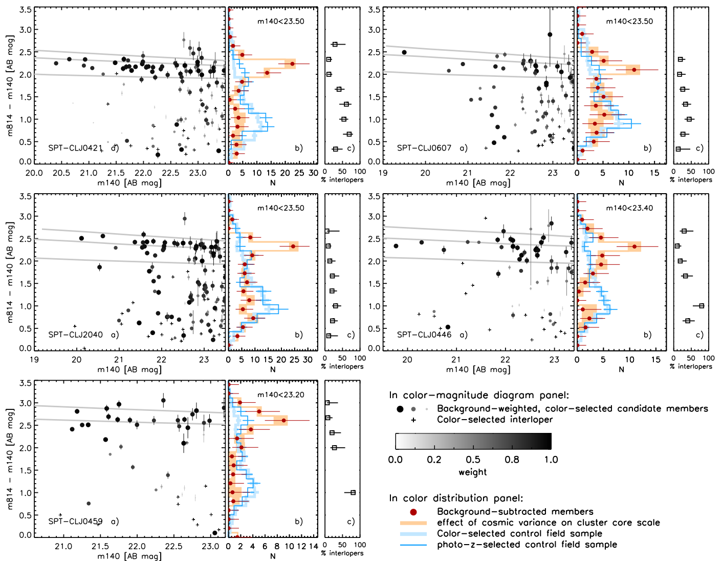
Fig. 1: Color-magnitude diagrams and derived properties within the r < 0.7r_{500} region of each cluster are shown in subfigures, each with three panels. Panel a ): Visualization of the background-subtracted color-magnitude diagram, where size and color of each galaxy point scale according to its statistical background subtraction weight (see color bar in legend) determined in Sect. 3.2. All galaxies are shown, but color-rejected interlopers (see Sect. 3.1) are shown as crosses. Gray lines show Kodama & Arimoto (1997) red-sequence (RS) models with formation redshifts z_f = 2, 3, 5 . The color range is the same for all clusters to facilitate direct comparison of RS colors. Panel b ): Color distribution of background-subtracted and area-corrected cluster members (red points with error bars) down to the indicated m_{140} limit. The orange shaded area shows an estimate of the impact of cosmic variance on the scale of the cluster core field, as detailed in Sect. 5.1. The blue histograms show the color distribution (rescaled by total number of galaxies) in the control-field sample, using the same color selection as for cluster candidate members (light blue), or a photometric redshift selection within \pm 0.2 of the cluster redshift (darker blue). All clusters show a clear excess of red galaxies with respect to the field distribution. Panel c ): Estimated fraction of interlopers in the color-selected candidate member sample as a function of color (down to the indicated m_{140} limit), based on the weights in panel a . Contamination is low for RS galaxies but significant for blue galaxies. Error bars show binomial confidence intervals ( 1\sigma ) computed following Cameron et al. (2011).
