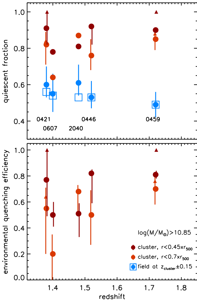
Fig. 10: Top : Quiescent fraction of cluster galaxies within r < 0.45r_{500} (dark red) and r < 0.7r_{500} (light red) above the common mass completeness limit \log(M/M_{\odot}) > 10.85 . Error bars account for uncertainties in the quiescent vs. star-forming classification as described in Sect. 5.3. Blue symbols show the quiescent fraction in corresponding photo- z selected control field samples (see Sect. 5.3). Large empty blue squares show values from the COSMOS field (see text). Bottom : Environmental quenching efficiency as derived from cluster and field quiescent fractions in the top panel. Color coding reflects the top panel. In both panels empty triangles show, where applicable, the quiescent fraction and derived quenching efficiency assuming that galaxies lacking a quiescent vs. star-forming classification are all quiescent (rather than all star-forming, see Sect. 5.2, Table 2).
