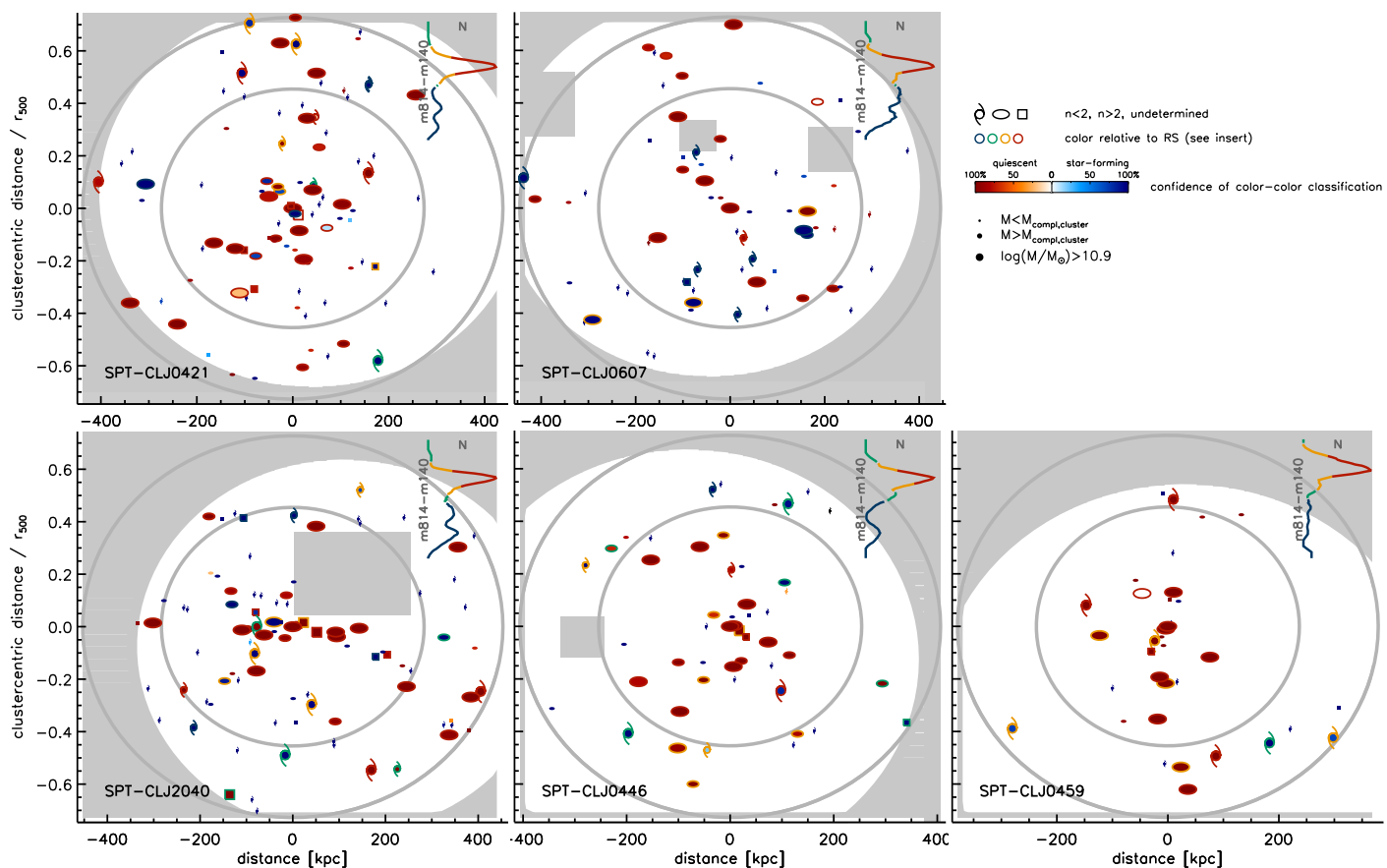
Fig. 9: Projected distribution of candidate cluster members. All candidate members are shown regardless of their statistical background subtraction weight. Each symbol has two colors. The color of the symbol boundary scales with the m814-m140 color of each galaxy relative to the cluster RS color (see insert). The internal symbol color, in red or blue shade according to the galaxy classification as quiescent or starforming, scales with the reliability of this classification only accounting for the distance of the galaxy colors from the adopted selection dividing line and the relevant photometric errors. Symbol shape reflects the estimated Sérsic index as indicated. Masked areas and regions deemed to be outside of our uniform coverage are gray shaded. The two circles show the limiting radii of the adopted cluster regions ( r < 0.45r_{500} , r < 0.7r_{500} ).
