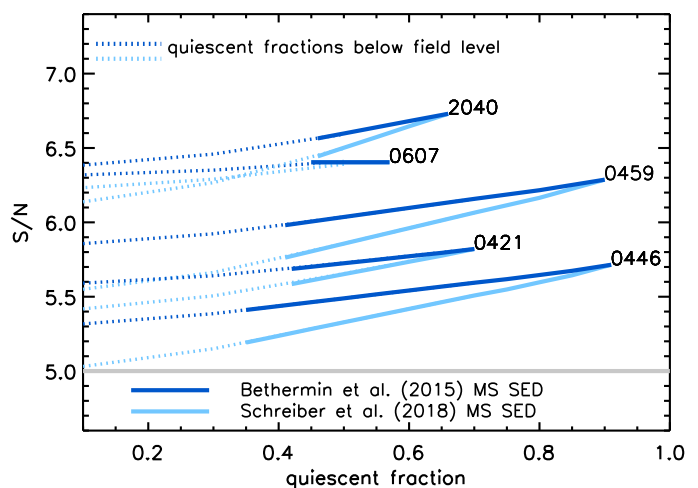
Fig. 11: Retrieved S/N of the cluster SZE detection obtained as a function of the r < 0.45r_{500} quiescent fraction, from the observed value down to the field level (solid lines) at the cluster redshift and mass completeness limit (see Sect. 5.4). Dotted lines show for completeness the retrieved S/N for central quiescent fractions down to 10%. For each cluster, the S/N is shown for both MS SEDs adopted to convert SFRs to 95, 150 GHz fluxes, as indicated. The gray line marks the S/N > 5 limit of our original sample selection. According to the modeling in Sect. 5.4, all five clusters would have been included in our S/N > 5 sample even if environmental quenching were negligible.
