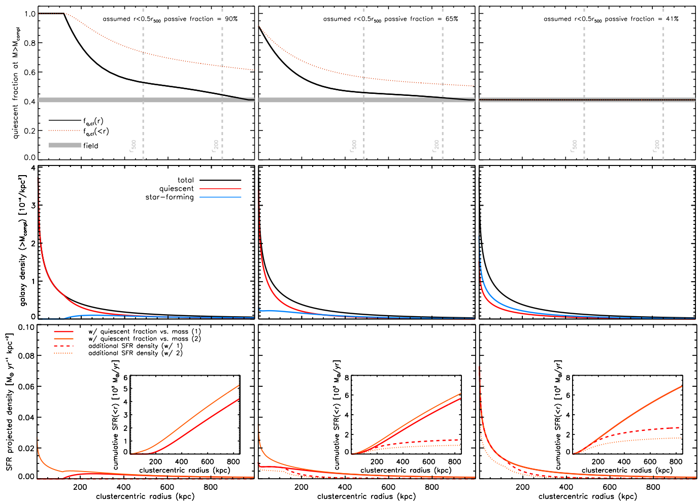
Fig. C.3: Example illustration of the modeling of the SFR density profiles described in Sect. 5.4, see text for full details. Left, middle and right panel columns correspond to three different values assumed for the r < r_{500} quiescent fraction above mass completeness, as indicated. Top panels show the radial profile of quiescent fraction above mass completeness (black, the field value is shown in gray). The dotted red line shows the quiescent fraction of the full mass complete sample out to the given clustercentric radius. Middle panels show the projected galaxy number density profile above mass completeness (black), and the derived profiles of star-forming and quiescent galaxies (blue and red) given the quiescent fraction profile in the corresponding top panel. Bottom panels show the corresponding projected SFR density profiles, derived with the two models of quiescent fraction vs. stellar mass as indicated (solid lines). Dashed and dotted lines show the additional SFR density profile over the prediction for the actually observed quiescent fraction (see text). Inserts show the corresponding cumulative SFR as a function of clustercentric radius.
