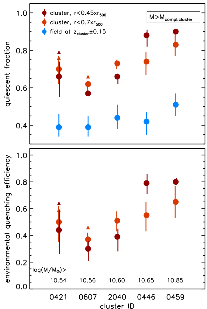
Fig. B.1: Top : Quiescent fraction of cluster galaxies within r < 0.45r_{500} (dark red) and r < 0.7r_{500} (light red) above the mass completeness limit of each cluster as reported in the bottom panel. Error bars account for uncertainties in the quiescent vs. star-forming classification as described in Sect. 5.3. Blue symbols show the quiescent fraction in corresponding photo-z selected control field samples (see Sect. 5.3). Bottom : Environmental quenching efficiency as derived from cluster and field quiescent fractions in the top panel. Color coding reflects the top panel. In both panels empty triangles show, where applicable, the quiescent fraction and derived quenching efficiency assuming that galaxies lacking a quiescent vs. star-forming classification are all quiescent (rather than all star-forming, see Sect. 5.2, Table 2).
