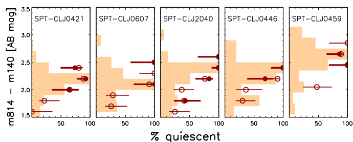
Fig. 8: Quiescent fraction vs. m814-m140 color for red ( m814-m140 > 1.5 ) galaxies in all five clusters. Galaxies bluer than m814-m140=1.5 are not shown as they are always classified as star-forming (thus 0% quiescent fraction, see Fig. 6). Shaded histograms represent the color distribution of cluster galaxies as in Fig. 1, arbitrarily rescaled. Empty and solid symbols show, respectively, quiescent fractions for the m140 -selected and for the \log(M/M_{\odot}) > 10.85 (common) mass complete samples. Error bars show binomial confidence intervals ( 1\sigma ). Color bins with < 2 galaxies are not shown.
