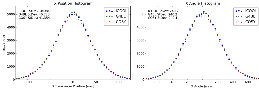
Figure 6. MICE Step IV upstream simulation (coils only).
