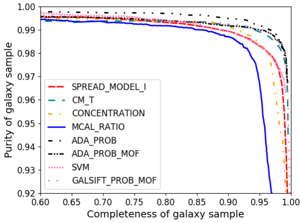
Figure 3. Precision-Recall (or completeness-purity) plot for classifiers tested on the SN fields over the Hubble-SC catalogue, using galaxies as truth. Magnitude range is given by MAG\_AUTO\_I = (17,24) . The SPREAD_MODEL-based cut is similar to the MODEST_CLASS used in DES Y1 analyses.
