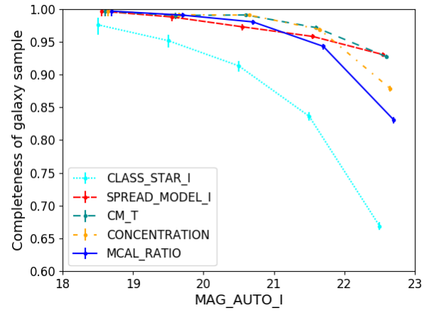
Figure 5. Completeness of a galaxy sample as a function of magnitude for classifiers tested on the COSMOS field, for a fixed galaxy purity of 99%.
