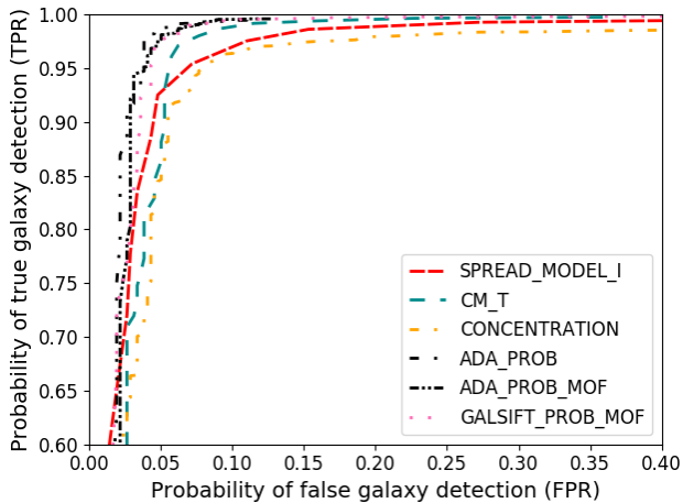
Figure 8. ROC plot for classifiers tested on the SN fields over the VVDS catalogues. Magnitude range is given by MAG\_AUTO\_I = (17,24) . The ROC curve is obtained by varying the threshold at which the classification divides the galaxy and star sample.
