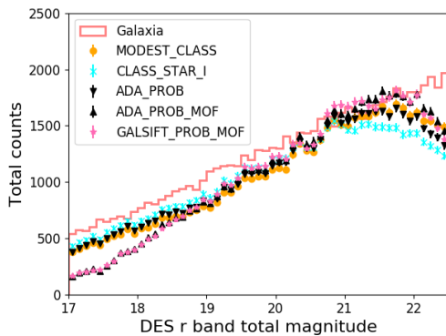
Figure 12. Counts for stars as classified by different algorithms compared to a Galaxia simulation (Sharma et al. 2011) using DES photometry, in the patch of the Y1 DES footprint with 45 < RA < 50 , -45 < DEC < -50 .
