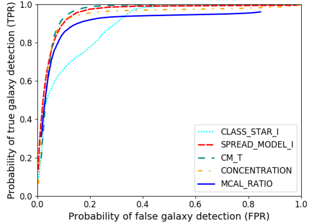
Figure 1. ROC plot for classifiers tested on the COSMOS field. Only non-ML codes are shown, as the machine-learning ones were trained in this dataset. Magnitude range is given by MAG\_AUTO\_I = (17,24) . The SPREAD_MODEL-based cut is similar to MODEST_CLASS used in Y1 analyses. The ROC curve is obtained by varying the threshold at which the classification divides the galaxy and star sample.
