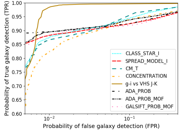
Figure 9. ROC plot for classifiers tested on the Stripe 82 region overlapping SDSS and VHS data. Magnitude range is given by MAG\_AUTO\_I = (17,21) . Note the logarithmic scale in the x-axis in this instance. The ROC curve is obtained by varying the threshold at which the classification divides the galaxy and star sample.
