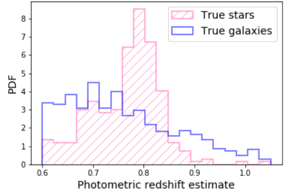
Figure 20. Normalised distribution of BPZ redshifts for a typical red galaxy sample that would be used for LSS studies, over a region with known identification of stars and galaxies through Hubble Space Telescope imaging.
