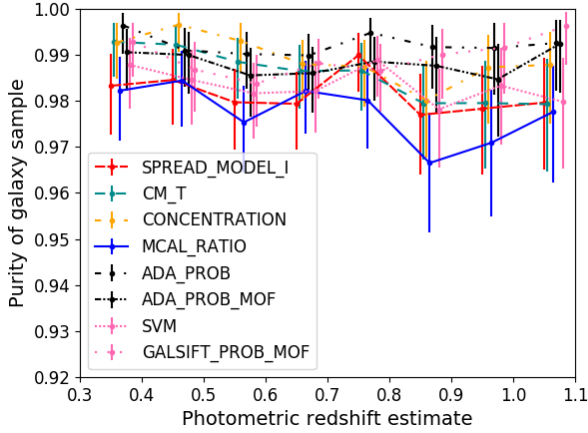
Figure 7. Purity of the galaxy sample as a function of photo- z for classifiers tested on Hubble-SC matches over the SN fields field, for a fixed 90% completeness. We use a random MonteCarlo sampling of the probability distribution function of redshift predicted by BPZ for that particular object as an estimate of its photo- z .
