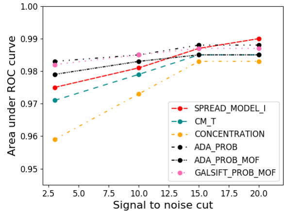
Figure 10. Area under the curve measured for the same classifiers as Figure 8, for different signal-to-noise thresholds, using the MAGERR\_AUTO quantity.
