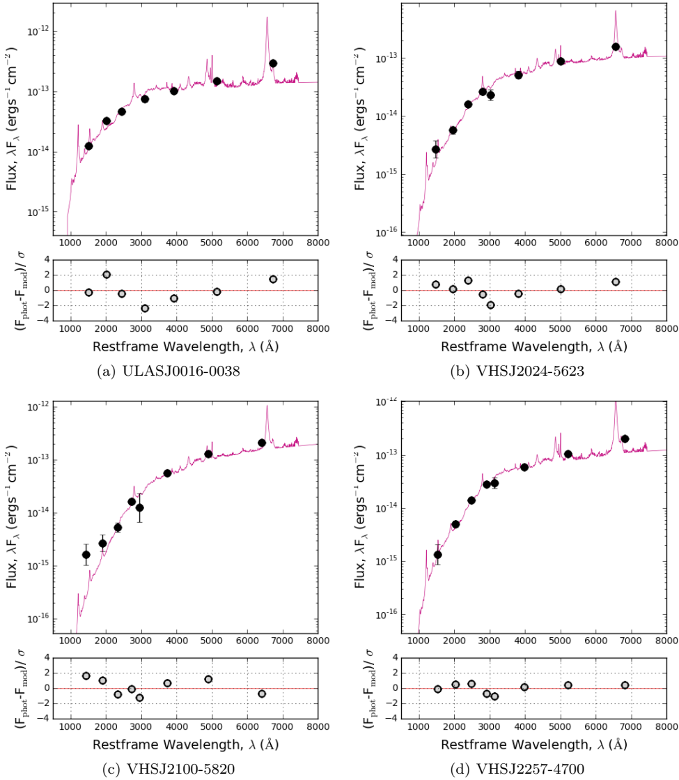
Figure 2. Upper panels: Best-fit quasar SEDs for ULASJ0016-0038 (a), VHSJ2024-5623 (b), VHSJ2100-5820 (c), VHSJ2257-4700 (d) for which \chi_{\text{red,QSO}}^2 < 2.5 . Black points show the grizY DES and JHK VHS/ULAS photometry. Lower panels: The error-weighted residuals for each fit.
