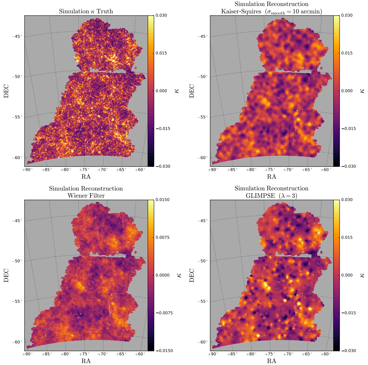
Figure 4. The top left panel is an example of a true convergence map, \kappa^{\text{truth}} , from simulation. The top right panel is the Kaiser-Squires reconstruction with a smoothing scale \sigma_{\text{smooth}} = 10 arcmin. The bottom right panel is the GLIMPSE reconstruction with regularisation parameter \lambda = 3.0 . Both tuning parameters were chosen to maximise the Pearson correlation coefficient r when tested on simulations (see Sec. 4.1). The bottom left panel is the Wiener filter reconstruction. Note that the colour scale for the Wiener filter is less than that for the other reconstructions, as the pixel values are closer to zero.
