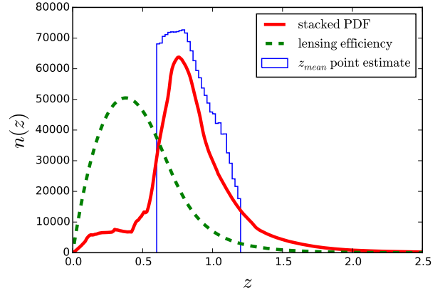
Figure 1. The redshift distribution from BPZ of the selected background galaxies with 0.6 < z_{\text{mean}} < 1.2 . The blue solid histogram is of the galaxies’ point estimate mean redshifts in bins of \Delta z = 0.02 . The red line is the stacked redshift probability density function (PDF) of all selected galaxies. The green dashed line is the lensing efficiency (equation 5) of the background galaxies.
