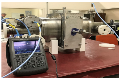
Figure 8: Setup for measuring tuner sensitivity for rf-dipole cavity.
