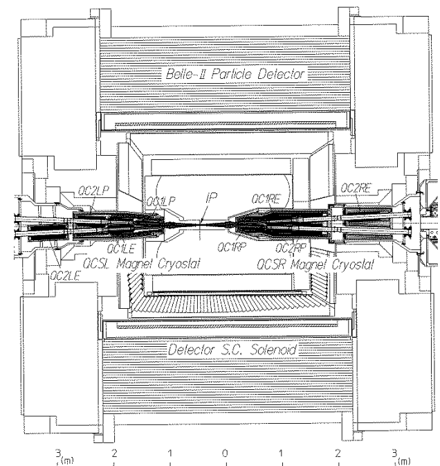
Figure 2: Horizontal cross section of the magnet-cryostats and the Belle II detector.
