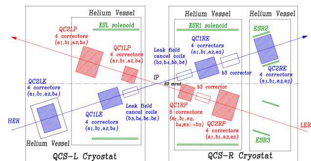
Figure 1: Layout of superconducting magnets in IR.
