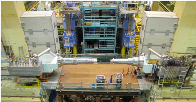
Figure 11: QCSL/R cryostats and Belle-II detector in IR.
