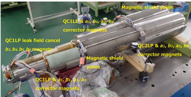
Figure 10: Assembled SC magnets in the front helium vessel of the QCSL cryostat.
