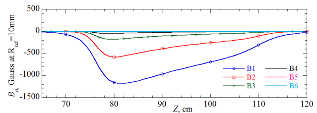
Figure 3: Leak field profiles along the HER beam line.
