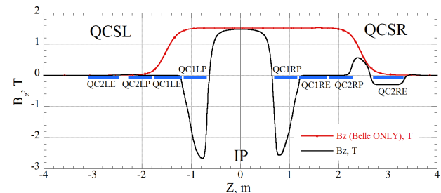
Figure 4: Solenoid field profiles along the beam lines.
