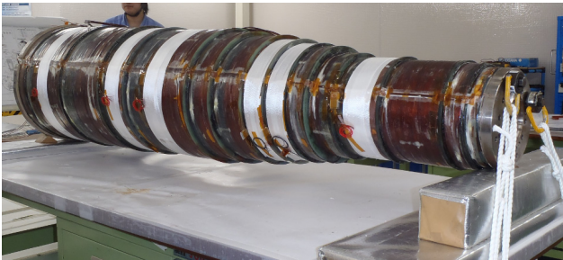
Figure 9: ESR1 compensation solenoid.
