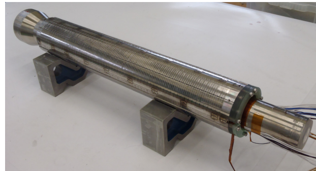
Figure 7: QC1LP with corrector magnets.
