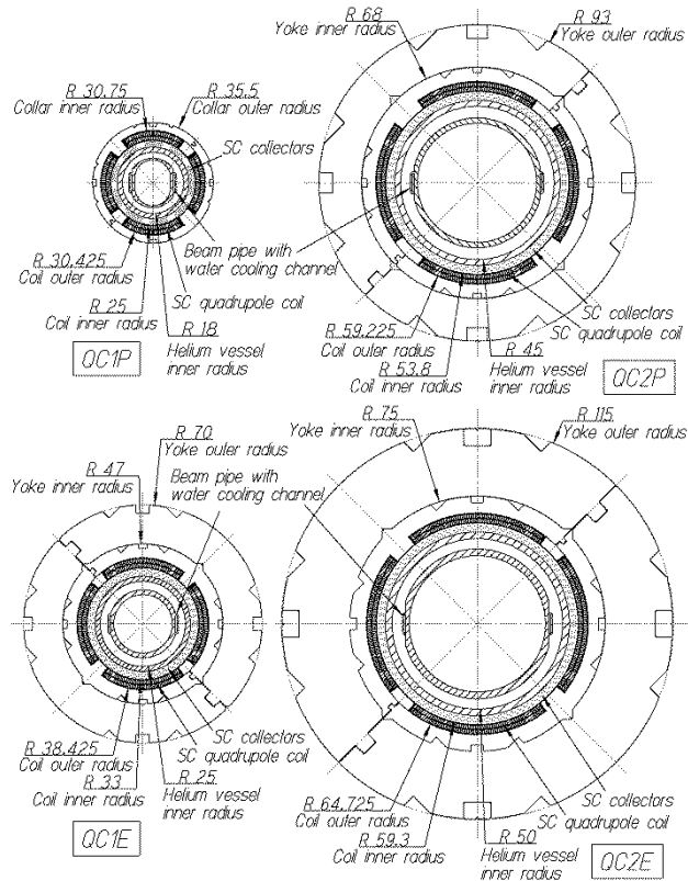
Figure 5: Cross section design of SC quadrupole magnets.
