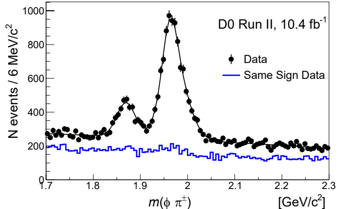
FIG. 2. The K^+ K^- \pi^\pm invariant mass distribution for the \mu^\pm \phi \pi^\mp sample (right sign) with the solid curve representing the fit. The lower mass peak is due to the decay D^\pm \rightarrow \phi \pi^\pm and the second peak is due to the D_s^\pm decay. The blue histogram below the data points is the invariant mass distribution for the same-sign sample, \mu^\pm \phi \pi^\pm .
