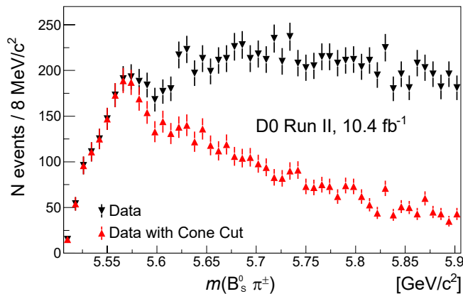
FIG. 3. The m(B_s^0\pi^\pm) distribution for the semileptonic data with (red upward triangles) and without (black downward triangles) the cone cut. Below 5.56 \text{GeV}/c^2 the red and black points have the same values.
