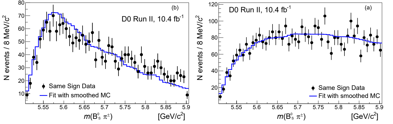
FIG. 6. The comparison of the m(B_s^0 \pi^\pm) background only distributions a) with the cone cut and b) without the cone cut, obtained using the weighted MC (histogram) and from the same sign data samples (points with error bars). The fluctuations in the number of MC events with the cone cut are due to the weighting procedure and the size of the sample.
