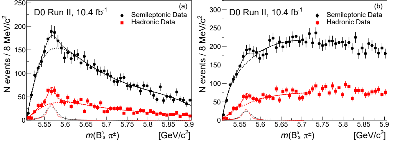
FIG. 11. The m(B_s^0 \pi^\pm) distribution for the hadronic (red squares) and semileptonic (black circles) data with the combined fitting function superimposed (a) with and (b) without the cone cut. (see text for details, the resulting fit parameters are given in Table VIII). The background parametrization function is taken from Eq. (1).
