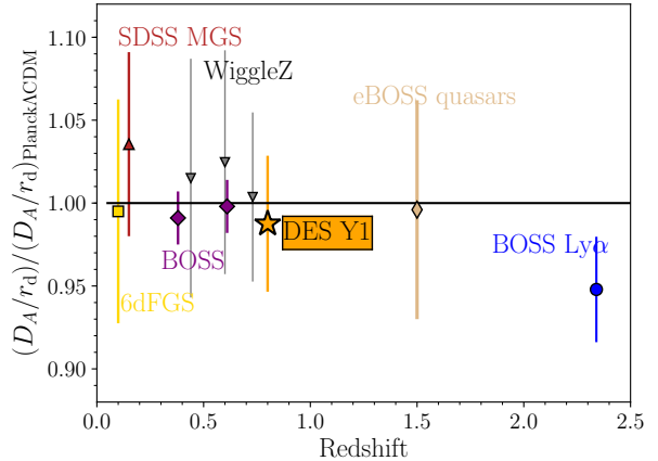
Figure 8. Measurement of the angular diameter distance measured from BAO, compared to the Planck \Lambda CDM prediction. The DES Y1 measurement is shown using a gold star. The additional measurements are described in the text. Where possible, we have used the available D_A measurement. Some studies have reported only spherically averaged distances; in these cases we have multiplied the uncertainty by 1.5 (as this is the approximate scaling between spherically averaged and transverse signal to noise). The results where this scaling was applied are 6dFGS, SDSS MGS, and eBOSS quasars.
