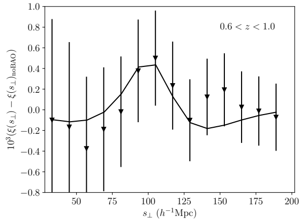
Figure 6. The BAO signal in DES Y1 clustering, observed in the auto-correlation binned in projected physical separation, \xi(s_\perp) , and isolated by subtracting the no BAO component of the best-fit model. Neighboring data points are strongly correlated.
