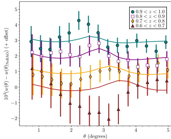
Figure 4. The BAO signal in DES Y1 clustering, observed in the angular auto-correlation, w(\theta) and isolated by subtracting the no BAO component of the best-fit model. The result has been multiplied by 10^3 and we add vertical offsets of 0, 1, 2, and 3 sequentially with redshift. The \theta values have been shifted by 0.03 for the 0.7 < z < 0.8 and by -0.03 for the 0.9 < z < 1.0 redshift bins. The BAO feature moves to lower \theta at higher redshift, as it has the same co-moving physical scale. The signal from these redshift bins is combined, accounting for the covariance between them, in order to provide a 4 per cent angular diameter distance measurement at the effective redshift of the full sample. Neighboring data points are strongly correlated. The total \chi^2/\text{dof} (including all cross-covariance between redshift bins) is 53/43 and other studies show that, despite its appearance, the 0.6 < z < 0.7 bin has a \chi^2/\text{dof} \sim 1 .
