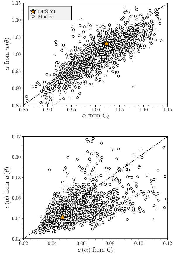
Figure 3. Same as Fig. 2, but the C_{\ell} results replace \xi(s_{\perp}) .
