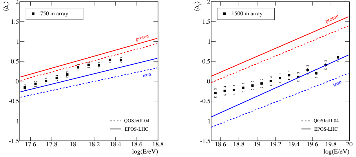
Figure 10: \langle \Delta_s \rangle as a function of the energy for the two surface arrays. Brackets correspond to the systematic uncertainties. Data are compared to the predictions obtained from simulations.
