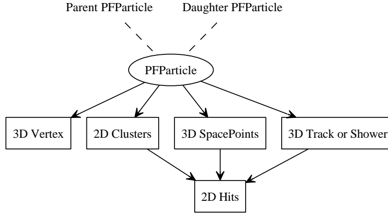
Fig. 1: The Pandora output data products, as persisted in the LArSoft Event Data Model. Navigation along PFPparticle hierarchies is achieved using the PFPparticle interface, represented by dashed lines. Navigation from PFPparticles to their associated objects is represented by solid arrows.
