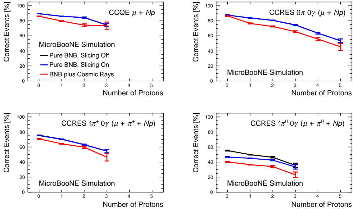
Fig. 20: The fraction of events deemed to have correct pattern recognition, shown for a selection of different BNB interactions with exclusive final states. Results are shown separately for samples of pure BNB events, with and without the slicing algorithm enabled, and for BNB events in the presence of cosmic-ray backgrounds. Correct events are those deemed to have exactly one reconstructed particle matched to each target MCParticle. The slicing algorithm has little impact for events with only track-like particles in the final state, so the blue and black lines overlap in three of the plots.
