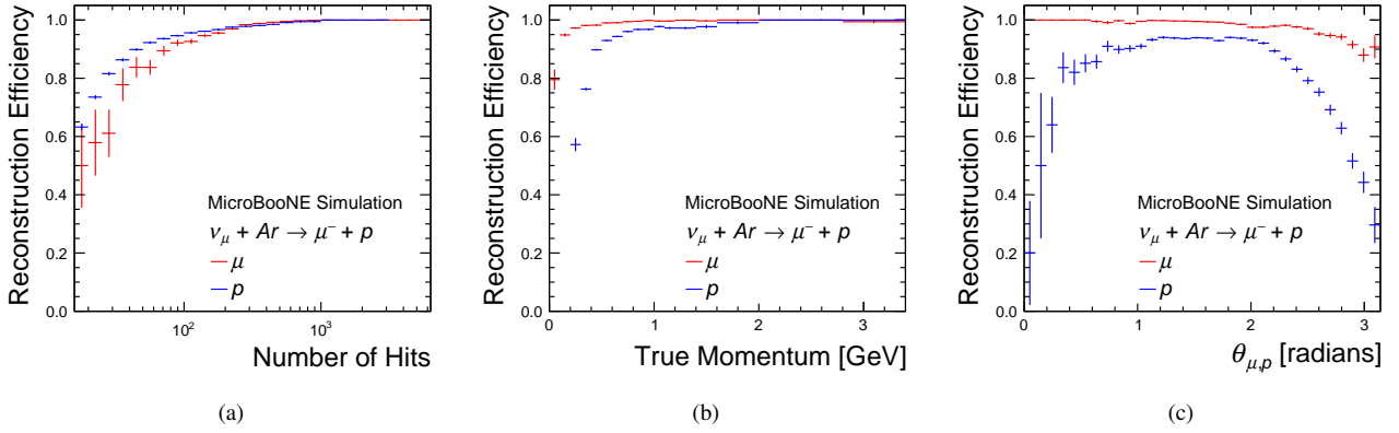
Fig. 11: Reconstruction efficiencies for the target muon and proton in simulated BNB CC \nu_\mu quasi-elastic interactions, (a) as a function of the numbers of true hits, (b) as a function of true momenta and (c) as a function of the true opening angle between the muon and proton.
